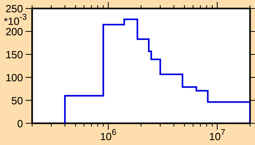
\sigma vs. E for ^{147}\text{Er}(n,n_4)
