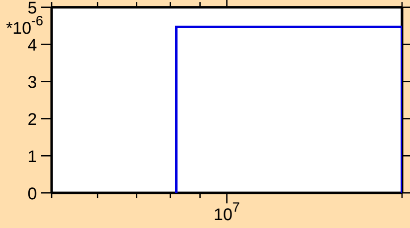
\sigma vs. E for ^{147}\text{Er}(n,2np)
