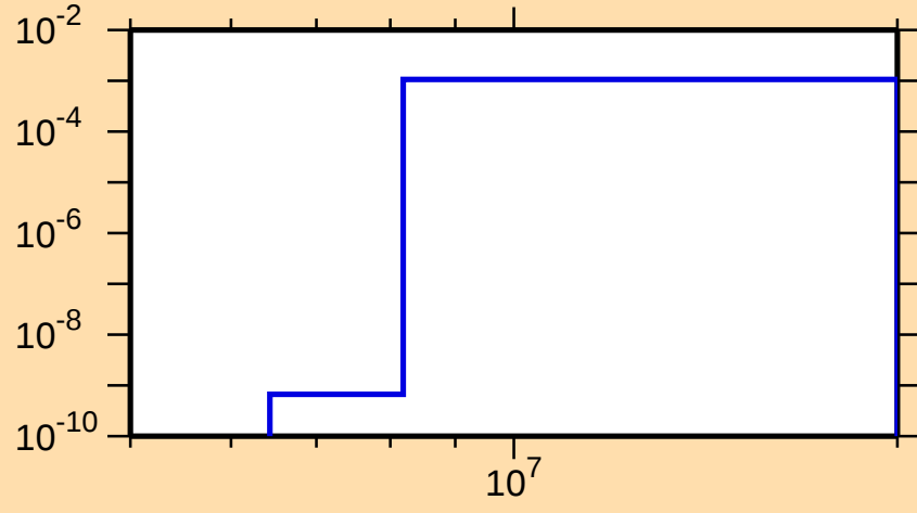
\sigma vs. E for ^{147}\text{Er}(n,\text{pd})
