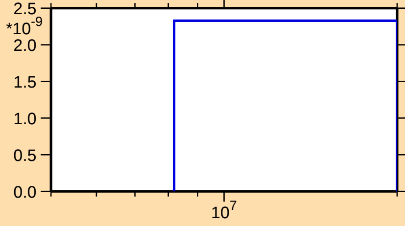
\sigma vs. E for ^{147}\text{Er}(n,\text{nd})
