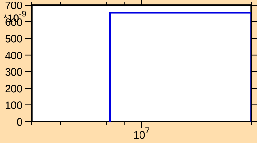
\sigma vs. E for ^{147}\text{Er}(\text{mt } 45)
