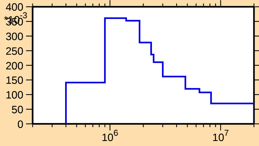
\sigma vs. E for ^{147}\text{Er}(n,n_3)
