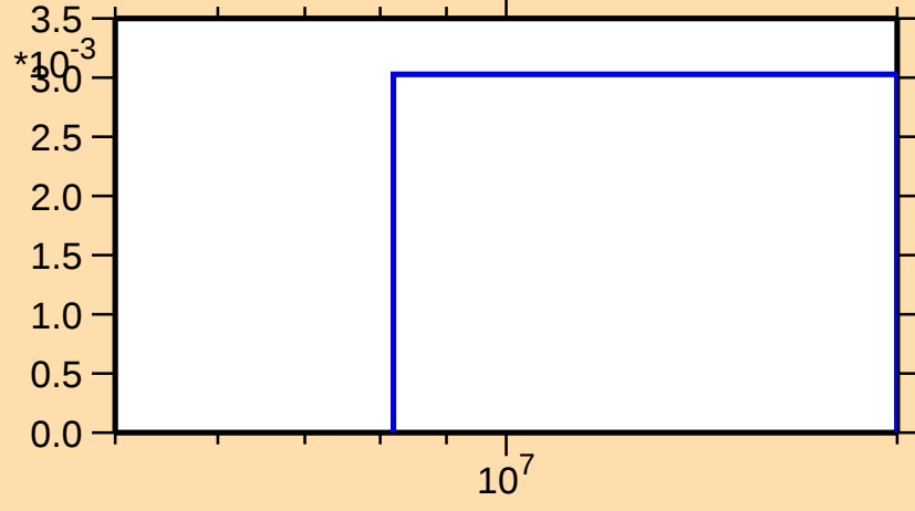
\sigma vs. E for ^{147}\text{Er}(n,2n)
