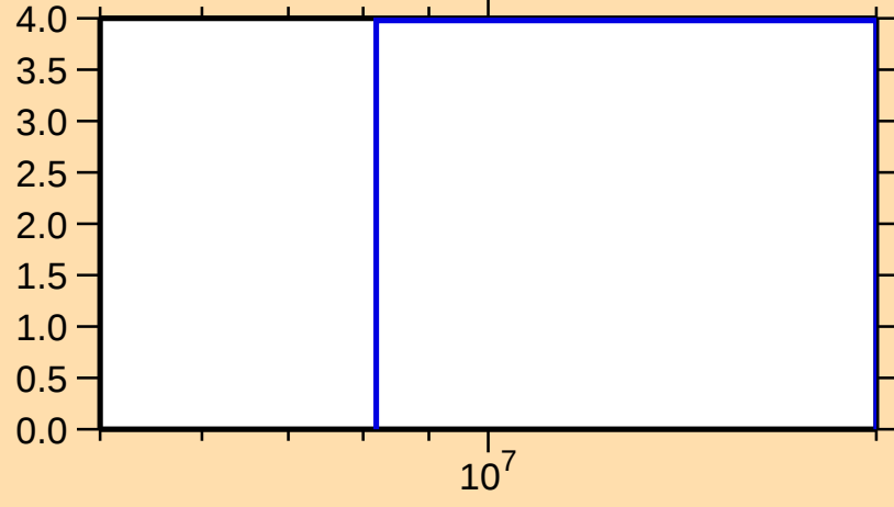
\Delta\sigma/\sigma vs. E for ^{147}\text{Er}(n,\text{tot.})
