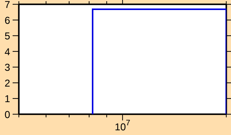
\Delta\sigma/\sigma vs. E for ^{147}\text{Er}(n,\text{el.})
