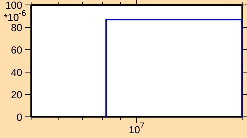
\sigma vs. E for ^{147}\text{Er}(n,t)
