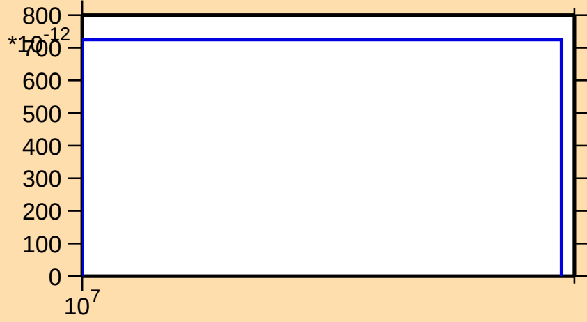
\sigma vs. E for ^{147}\text{Er} (mt 34)
