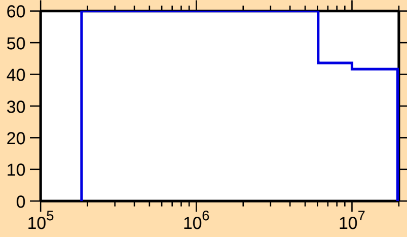
\Delta\sigma/\sigma vs. E for ^{147}\text{Er}(n,n\text{cont.})
