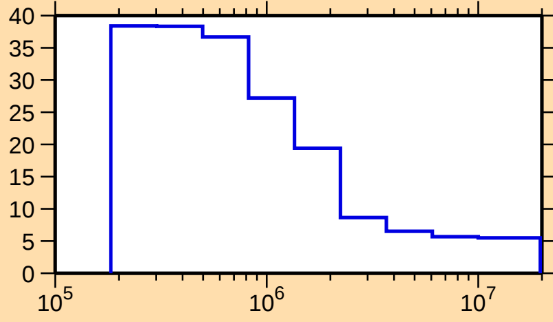
\Delta\sigma/\sigma vs. E for ^{147}\text{Er}(n,\text{nonel.})
