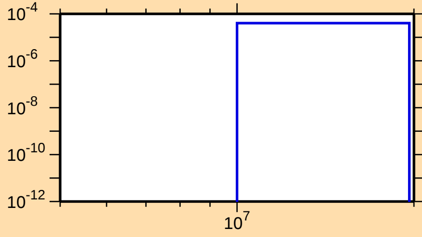
\sigma vs. E for ^{147}\text{Er}(n,t)
