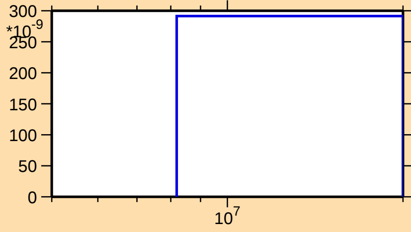
\sigma vs. E for ^{147}\text{Er} (mt 45)
