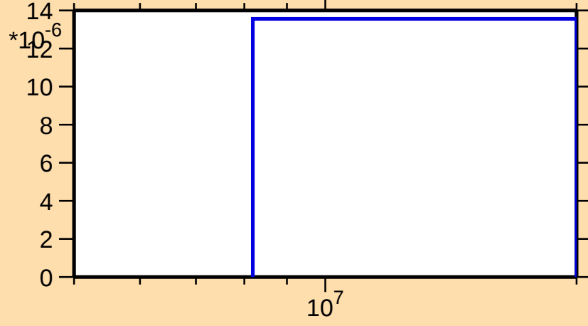
\sigma vs. E for ^{147}\text{Er}(n,\text{pt})
