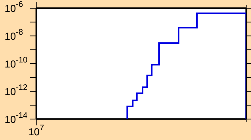
\sigma vs. E for ^{149}\text{Er}(n,\text{nd})
