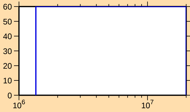
\Delta\sigma/\sigma vs. E for ^{149}\text{Er}(n,\text{ncont.})
