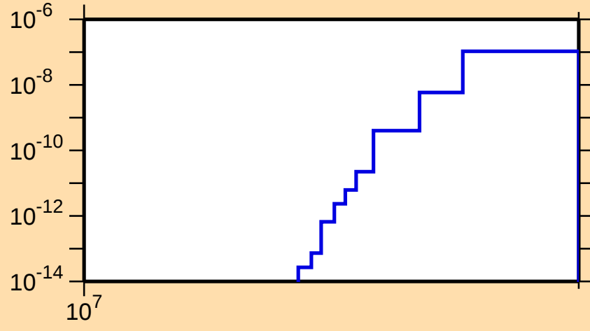
\sigma vs. E for ^{149}\text{Er}(n,2n\alpha)
