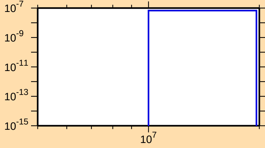
\sigma vs. E for ^{149}\text{Er}(\text{mt } 45)
