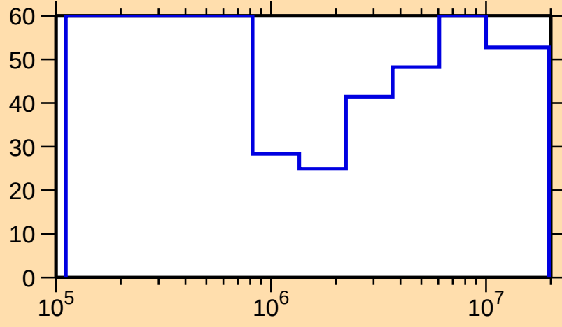
\Delta\sigma/\sigma vs. E for ^{149}\text{Er}(\text{n,el.})
