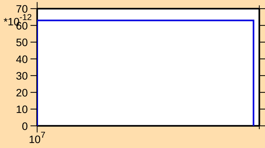
\sigma vs. E for ^{149}\text{Er}(\text{mt117})
