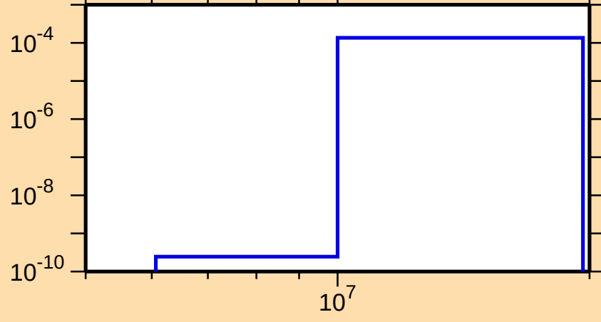
\sigma vs. E for ^{149}\text{Er}(n,\text{pd})
