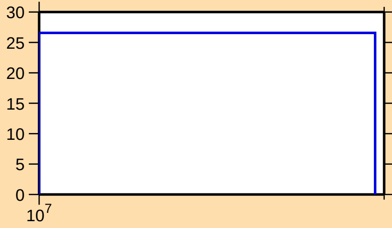
\Delta\sigma/\sigma vs. E for ^{149}\text{Er}(n,\text{tot.})
