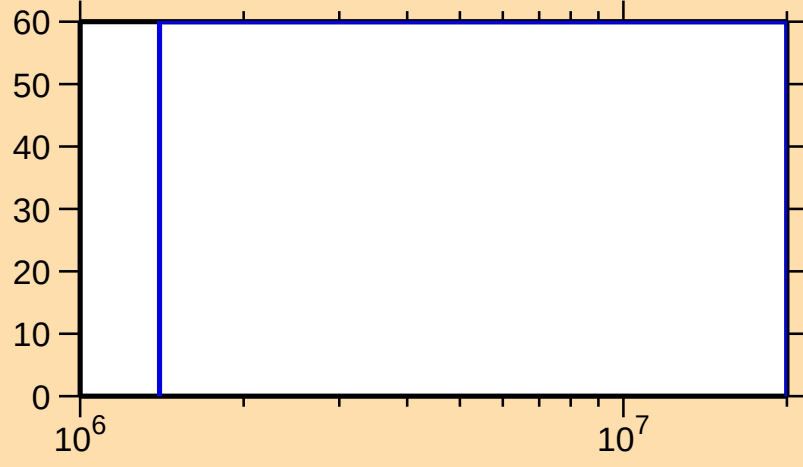
\Delta\sigma/\sigma vs. E for ^{149}\text{Er}(n,\text{ncont.})
