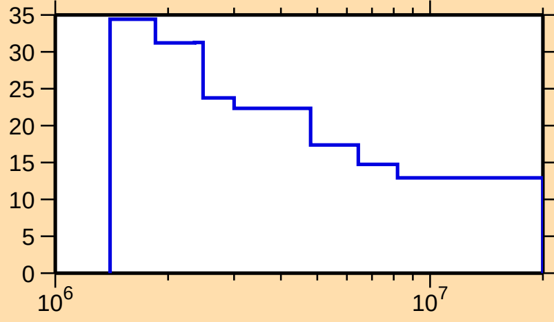
\Delta\sigma/\sigma vs. E for ^{149}\text{Er}(\text{n},\text{nonel.})
