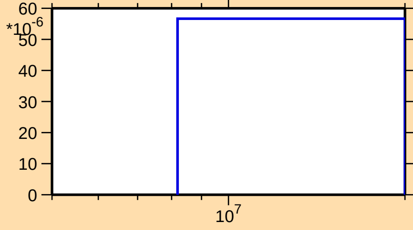
\sigma vs. E for ^{149}\text{Er}(n,t)
