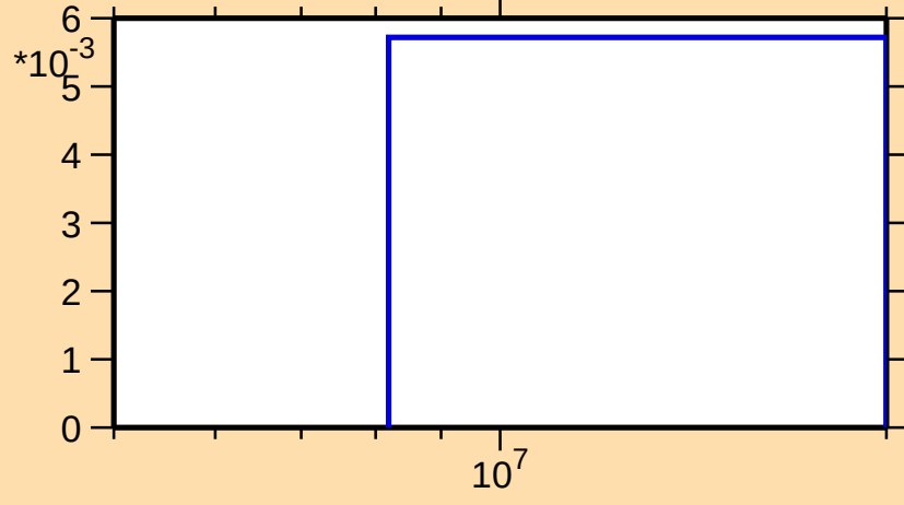
\sigma vs. E for ^{149}\text{Er}(n,2n)
