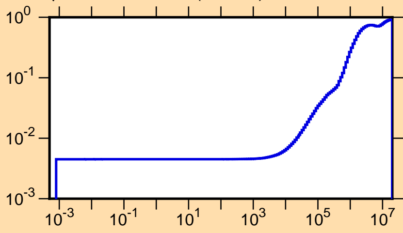
\mu vs. E for ^{150}\text{Er}(\text{mt251})
