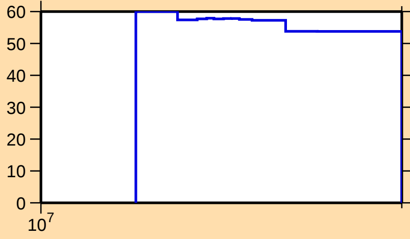
\Delta\sigma/\sigma vs. E for ^{150}\text{Er}(n,\text{inel.})
