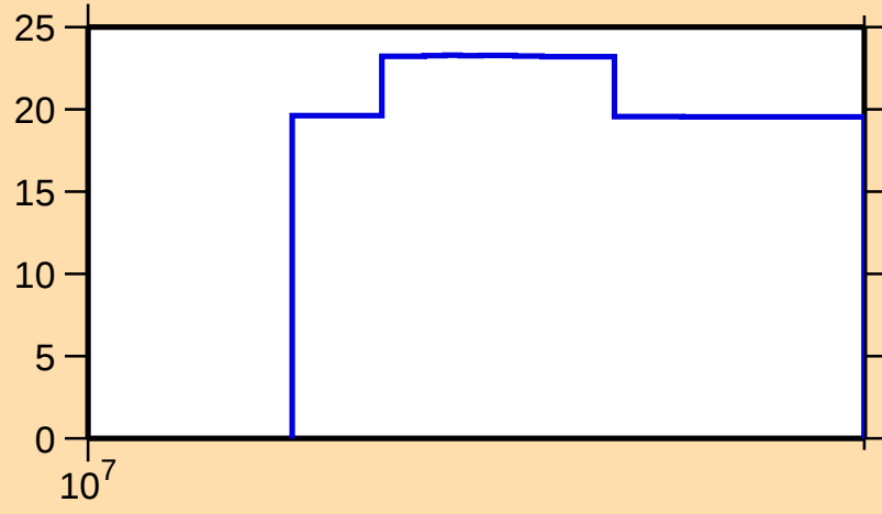
\Delta\sigma/\sigma vs. E for ^{150}\text{Er}(n,\text{nonel.})
