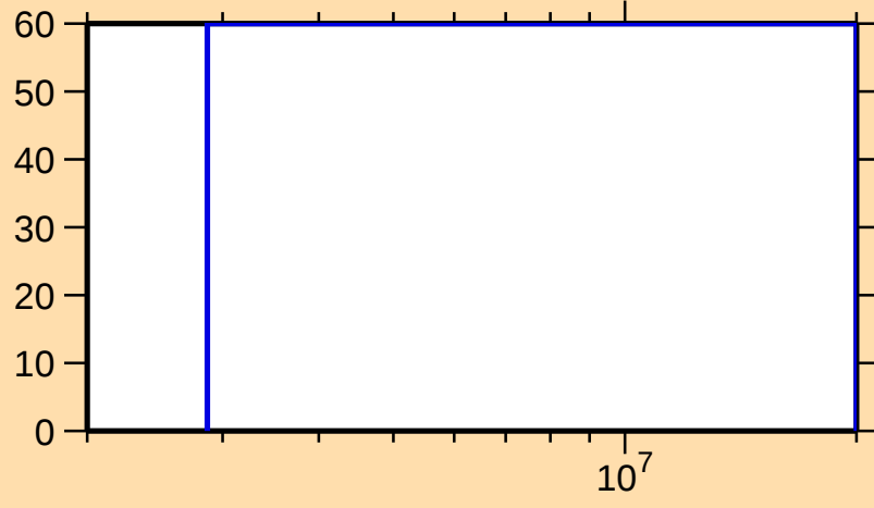
\Delta\sigma/\sigma vs. E for ^{150}\text{Er}(n,n\text{cont.})
