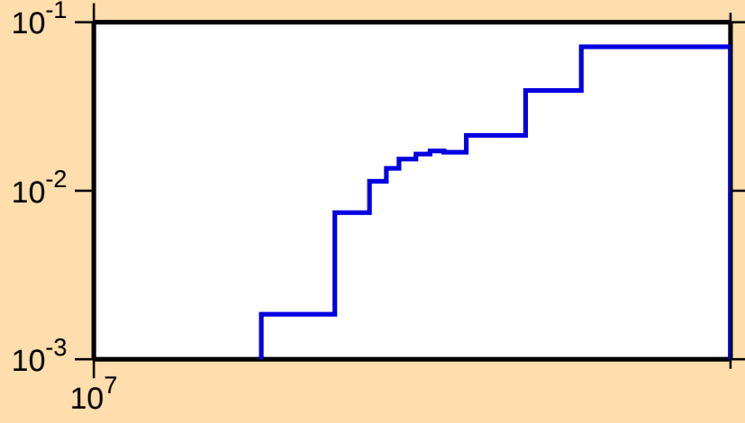
\sigma vs. E for ^{150}\text{Er}(n,2n)
