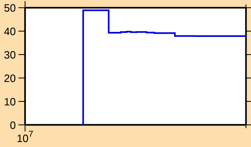
\Delta\sigma/\sigma vs. E for ^{150}\text{Er}(n,\text{el.})
