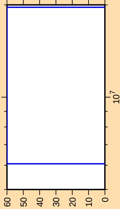
\Delta\sigma/\sigma vs. E for ^{150}\text{Er}(n,\text{pd})
