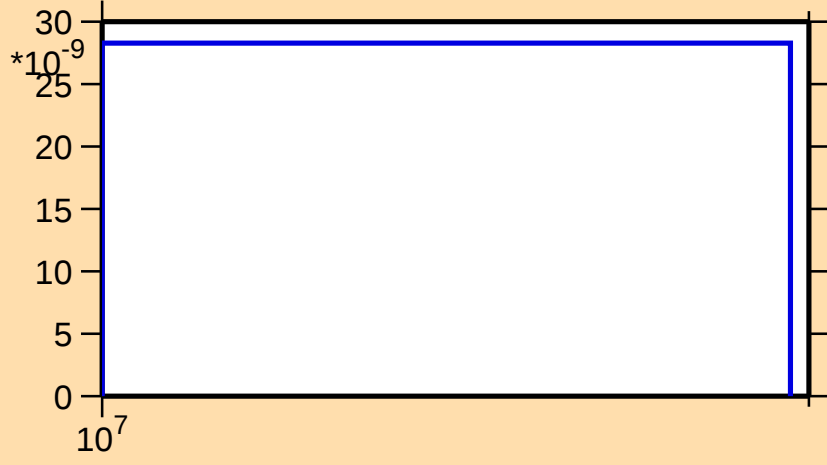
\sigma vs. E for ^{150}\text{Er}(n,2np)
