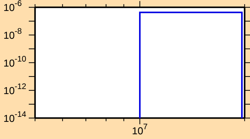
\sigma vs. E for ^{150}\text{Er}(\text{mt } 45)
