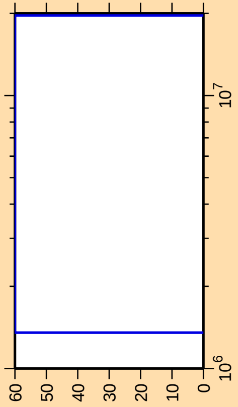
\Delta\sigma/\sigma vs. E for ^{150}\text{Er}(n,\gamma)
