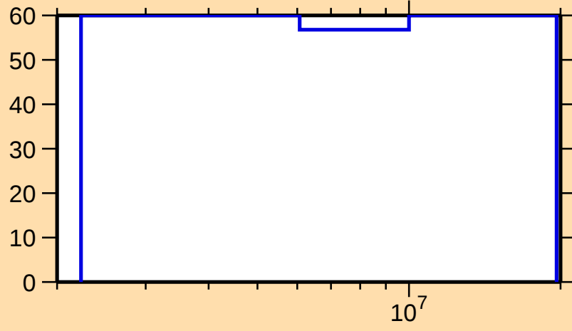
\Delta\sigma/\sigma vs. E for ^{150}\text{Er}(\text{n},\text{inel.})
