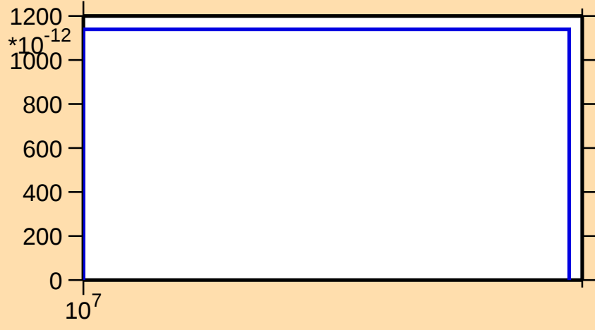
\sigma vs. E for ^{150}\text{Er}(n,\text{pt})
