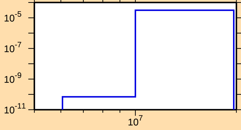
\sigma vs. E for ^{150}\text{Er}(n,\text{pd})
