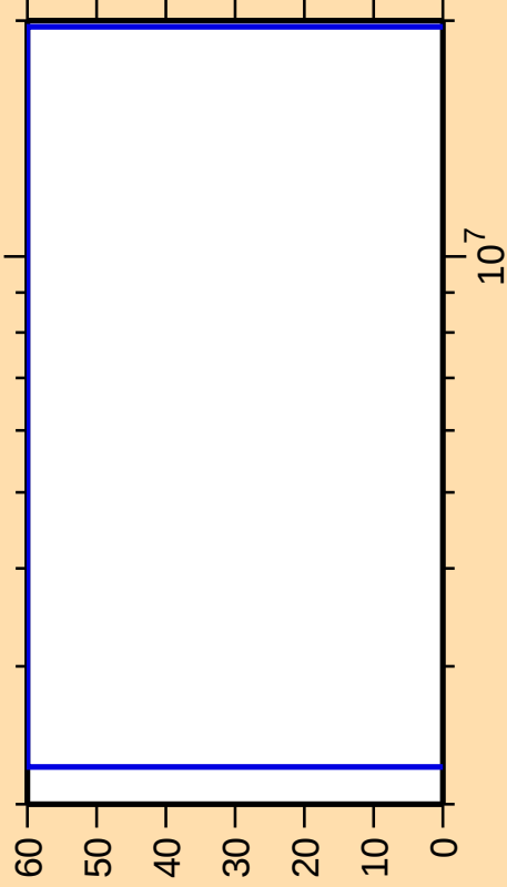
\Delta\sigma/\sigma vs. E for ^{150}\text{Er}(n,n_{\text{cont}})
