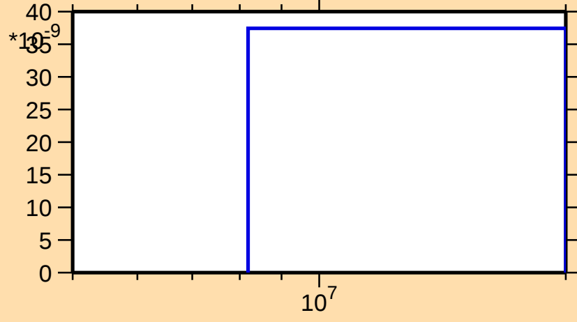
\sigma vs. E for ^{150}\text{Er}(n,2np)
