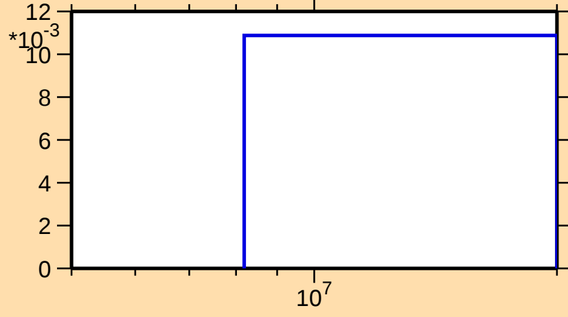
\sigma vs. E for ^{150}\text{Er}(n,2n)
