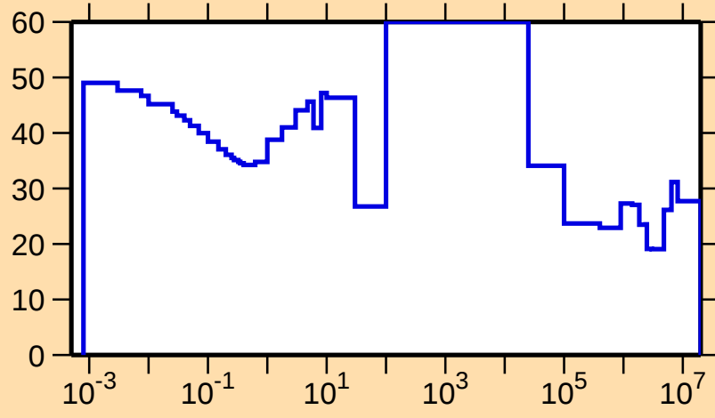
\Delta\sigma/\sigma vs. E for ^{150}\text{Er}(n,\text{tot.})
