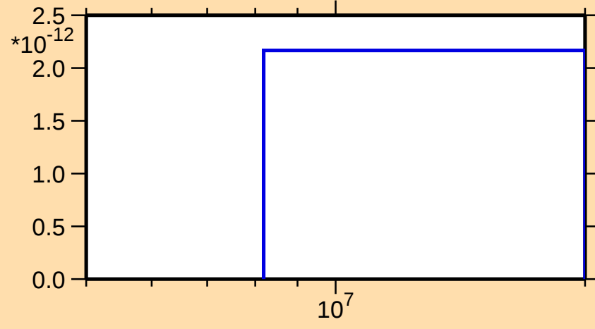
\sigma vs. E for ^{150}\text{Er}(n,2n\alpha)
