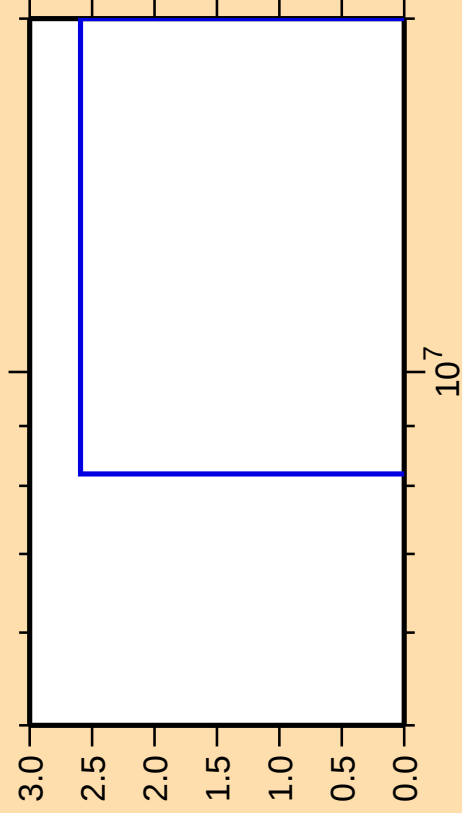
\Delta\sigma/\sigma vs. E for ^{150}\text{Er}(n,2n\alpha)
