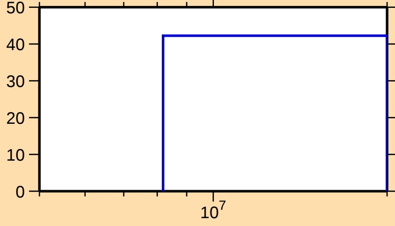
\Delta\sigma/\sigma vs. E for ^{150}\text{Er}(n,\text{el.})
