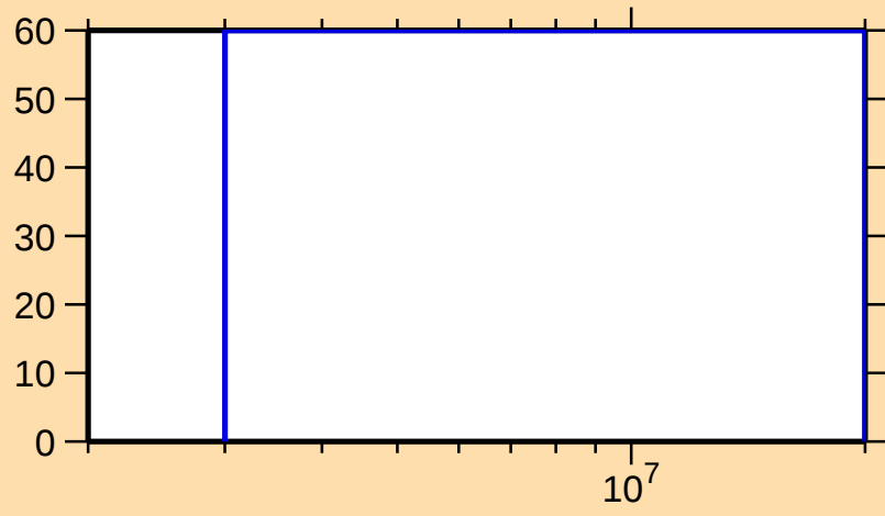
\Delta\sigma/\sigma vs. E for ^{150}\text{Er}(n,n\text{cont.})
