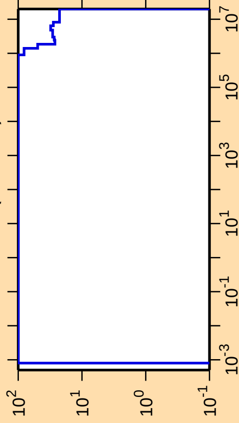
\Delta\sigma/\sigma vs. E for ^{150}\text{Er}(n,\text{nonel.})
