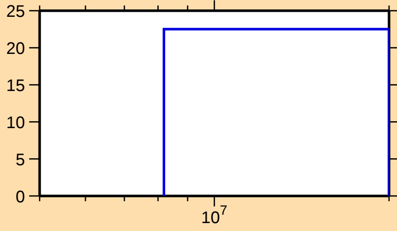
\Delta\sigma/\sigma vs. E for ^{150}\text{Er}(n,\text{nonel.})
