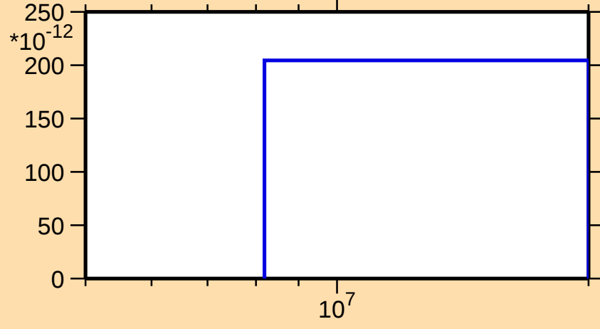
\sigma vs. E for ^{150}\text{Er}(n,\text{nd})
