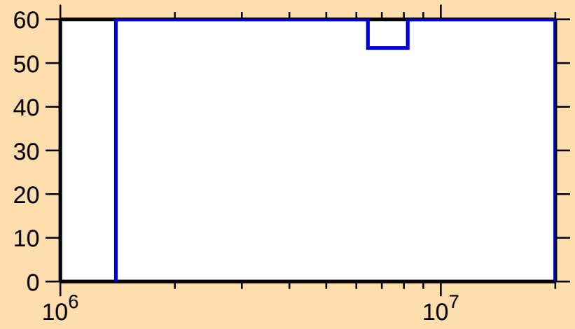
\Delta\sigma/\sigma vs. E for ^{150}\text{Er}(n,n_1)
