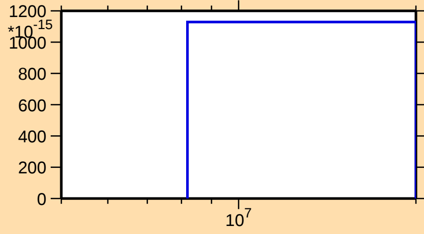
\sigma vs. E for ^{150}\text{Er}(\text{mt } 34)
