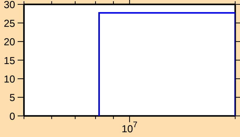
\Delta\sigma/\sigma vs. E for ^{150}\text{Er}(n,\text{tot.})
