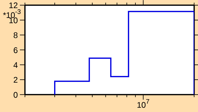
\sigma vs. E for ^{150}\text{Er}(n,n\text{cont.})
