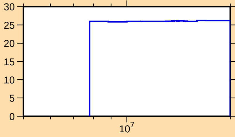
\Delta\sigma/\sigma vs. E for ^{151}\text{Er}(n,\text{nonel.})
