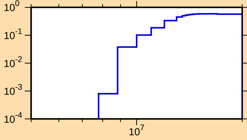
\sigma vs. E for ^{151}\text{Er}(n,2n)
