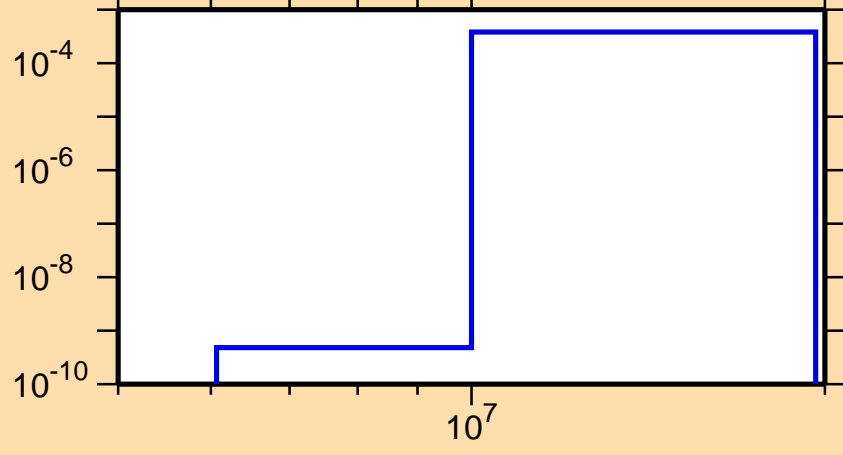
\sigma vs. E for ^{151}\text{Er}(n,t)
