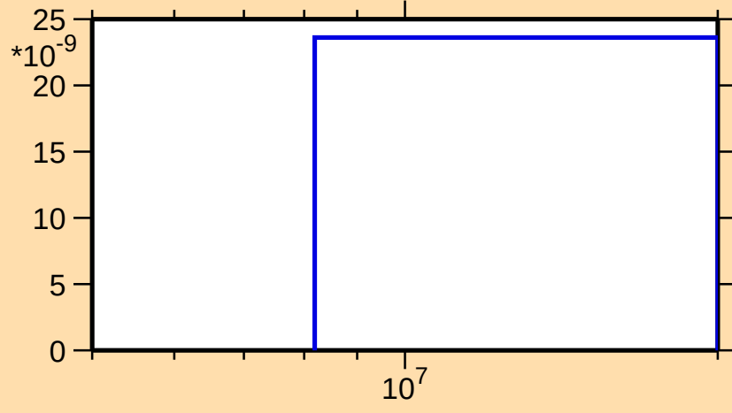
\sigma vs. E for ^{151}\text{Er}(n,2n\alpha)
