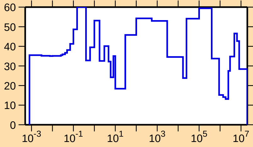
\Delta\sigma/\sigma vs. E for ^{151}\text{Er}(n,\text{tot.})
