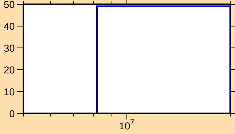
\Delta\sigma/\sigma vs. E for ^{151}\text{Er}(n,\text{el.})
