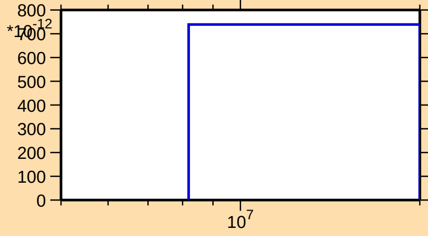
\sigma vs. E for ^{151}\text{Er}(\text{mt } 34)
