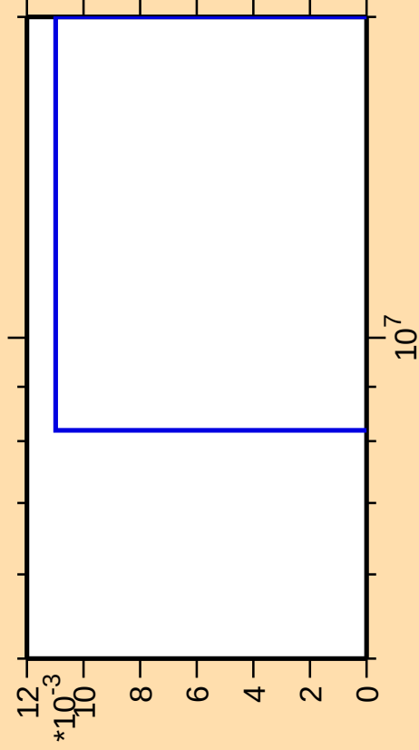
\Delta\sigma/\sigma vs. E for ^{151}\text{Er}(n,nt)
