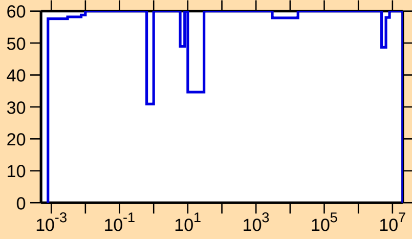
\Delta\sigma/\sigma vs. E for ^{151}\text{Er}(n,\gamma)
