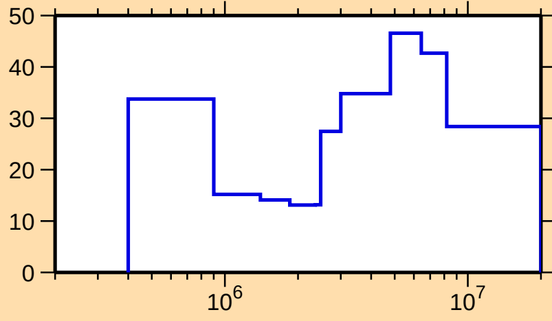
\Delta\sigma/\sigma vs. E for ^{151}\text{Er}(n,\text{tot.})
