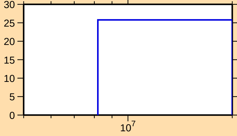
\Delta\sigma/\sigma vs. E for ^{151}\text{Er}(n,\text{nonel.})
