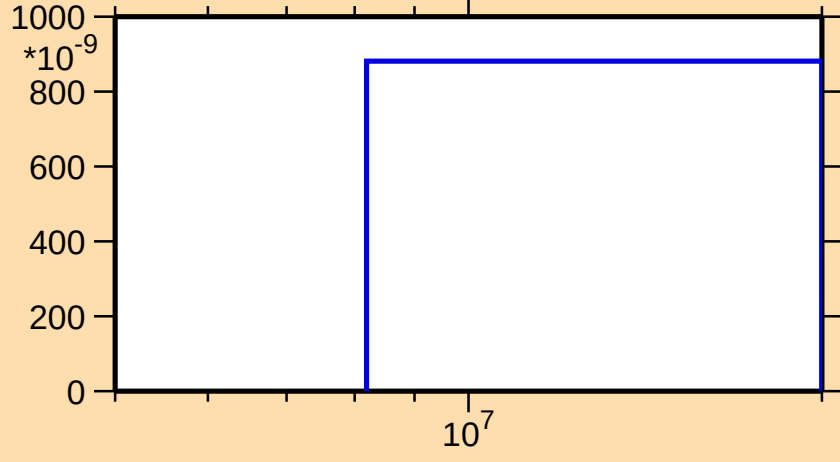
\sigma vs. E for ^{151}\text{Er}(n,\text{nd})
