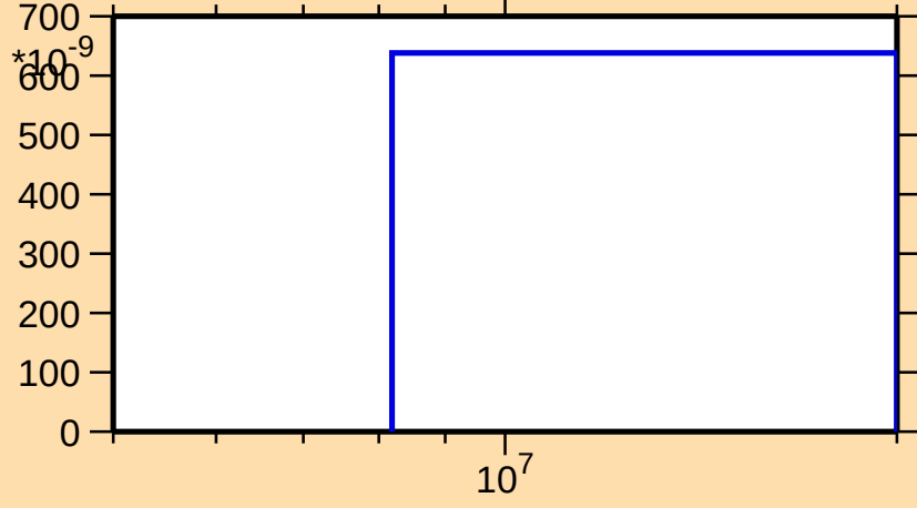
\sigma vs. E for ^{151}\text{Er}(n,\text{pt})
