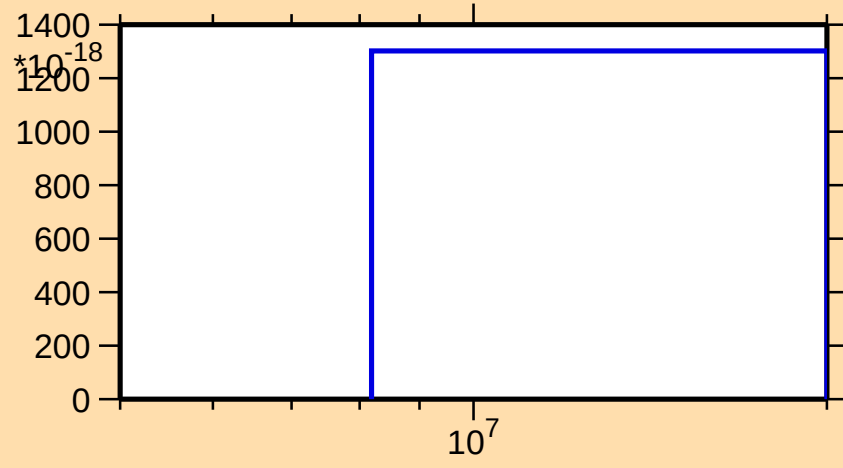
\sigma vs. E for ^{151}\text{Er}(n,nt)
