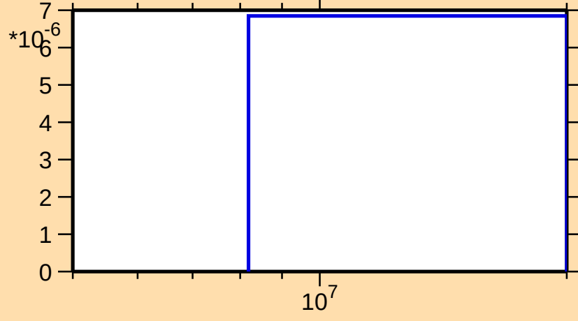
\sigma vs. E for ^{151}\text{Er}(n,\text{pd})
