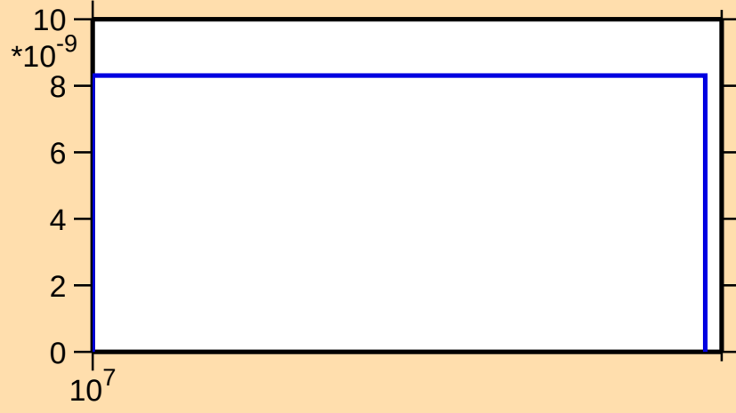
\sigma vs. E for ^{152}\text{Er}(n,\text{nd})
