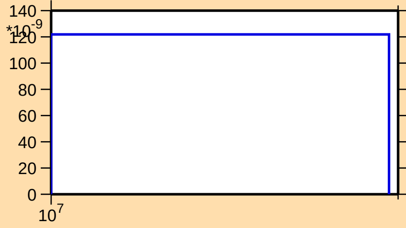
\sigma vs. E for ^{152}\text{Er}(n,3n)
