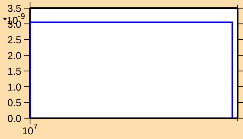
\sigma vs. E for ^{152}\text{Er}(n,\text{pt})
