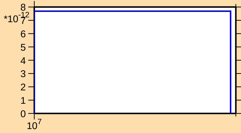
\sigma vs. E for ^{152}\text{Er}(n,\text{nt})
