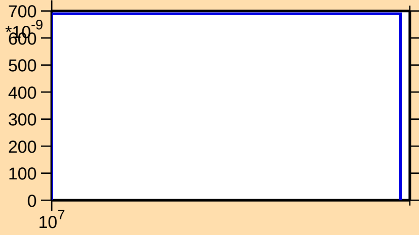
\sigma vs. E for ^{152}\text{Er}(n,2np)
