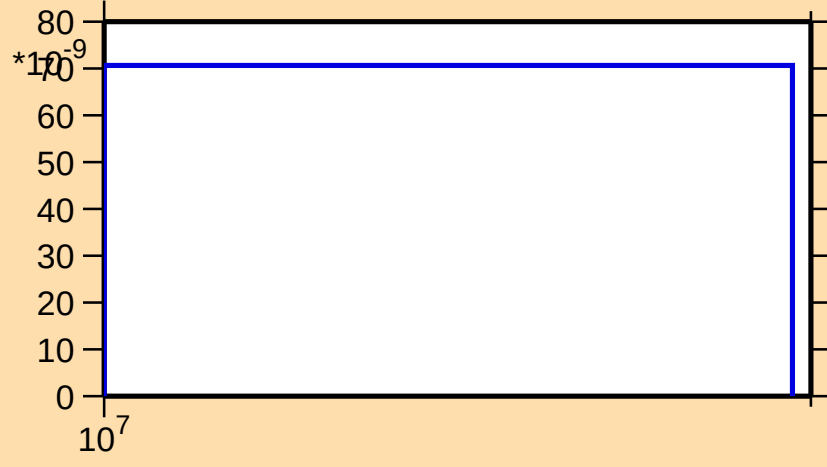
\sigma vs. E for ^{152}\text{Er}(n,2n\alpha)
