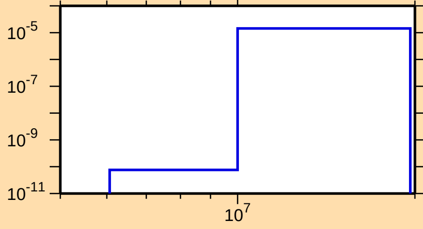
\sigma vs. E for ^{152}\text{Er}(\text{mt 45})
