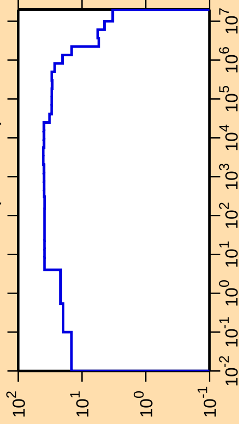
\Delta\sigma/\sigma vs. E for ^{152}\text{Er}(n,\text{nonel.})
