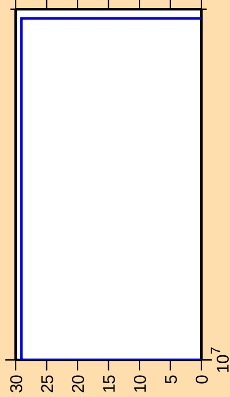
\Delta\sigma/\sigma vs. E for ^{152}\text{Er}(n,\text{nt})
