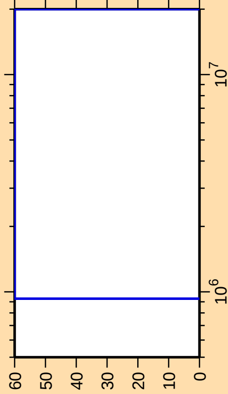
\Delta\sigma/\sigma vs. E for ^{153}\text{Er}(n,p\alpha)
