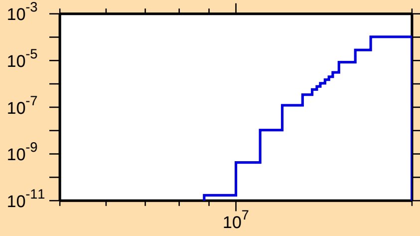
\sigma vs. E for ^{153}\text{Er}(\text{mt 45})
