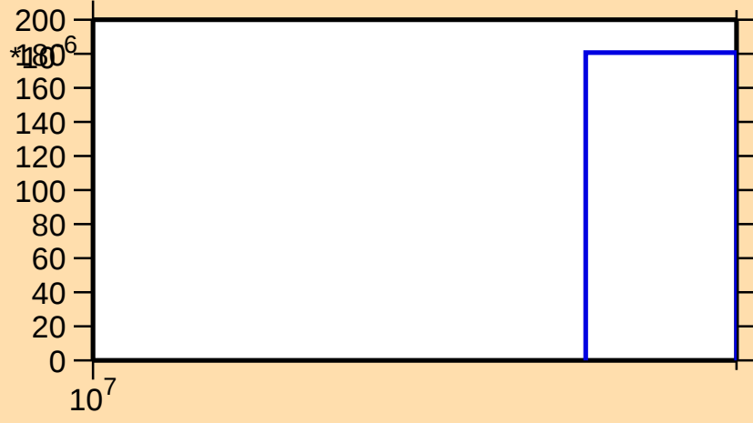
\sigma vs. E for ^{153}\text{Er}(n,3n)
