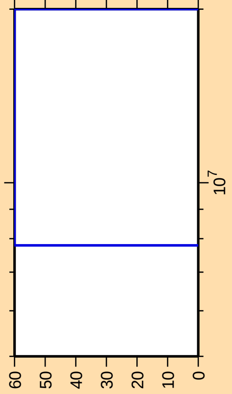
\Delta\sigma/\sigma vs. E for ^{153}\text{Er}(n,\gamma)
