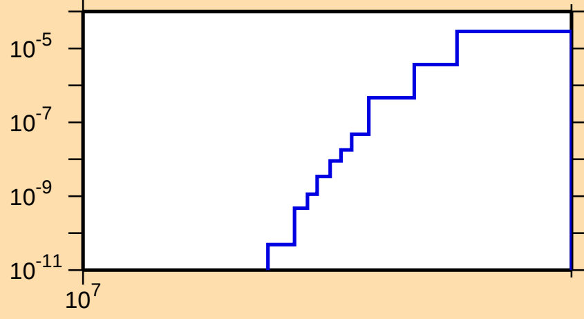
\sigma vs. E for ^{153}\text{Er}(n,\text{nd})
