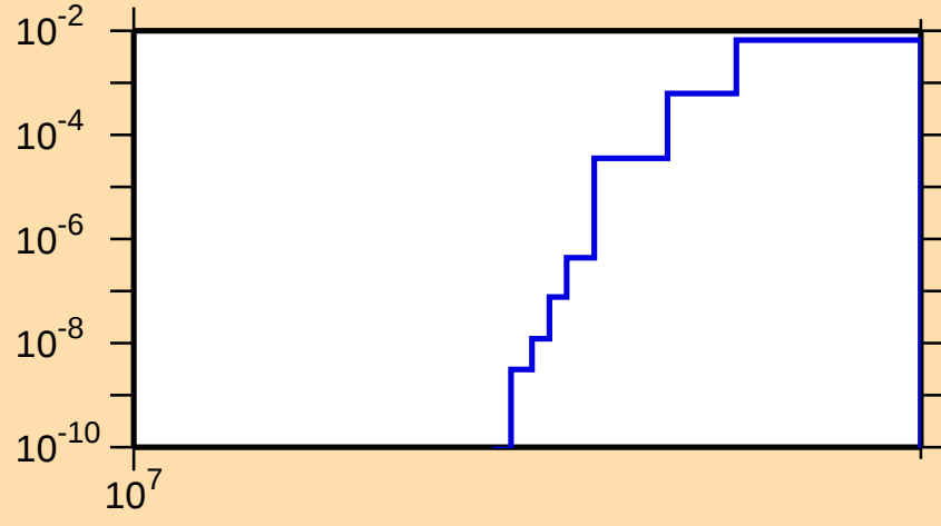
\sigma vs. E for ^{153}\text{Er}(n,2np)
