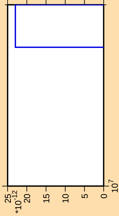
\Delta\sigma/\sigma vs. E for ^{153}\text{Er}(\text{mt 11})
