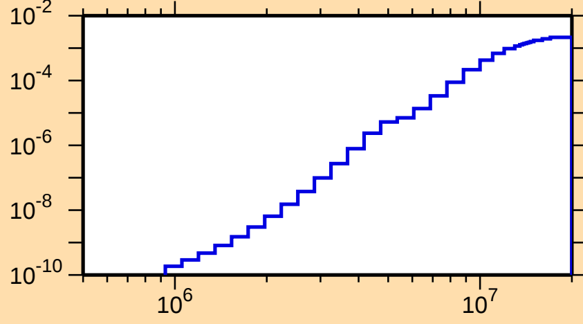
\sigma vs. E for ^{153}\text{Er}(n,p\alpha)
