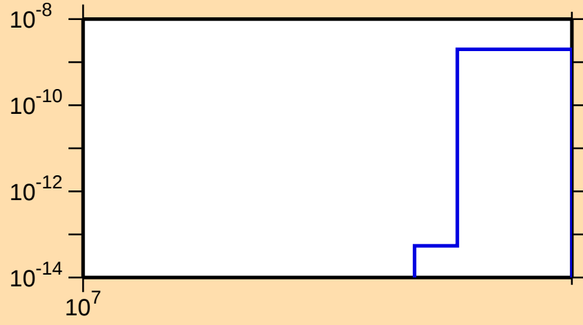
\sigma vs. E for ^{153}\text{Er}(n,nt)
