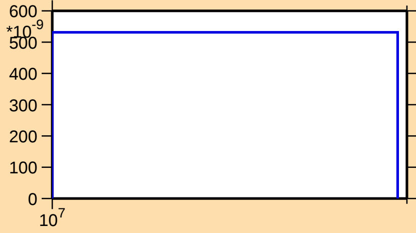
\sigma vs. E for ^{153}\text{Er}(n,\text{nd})
