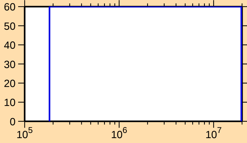
\Delta\sigma/\sigma vs. E for ^{153}\text{Er}(n,n_1)
