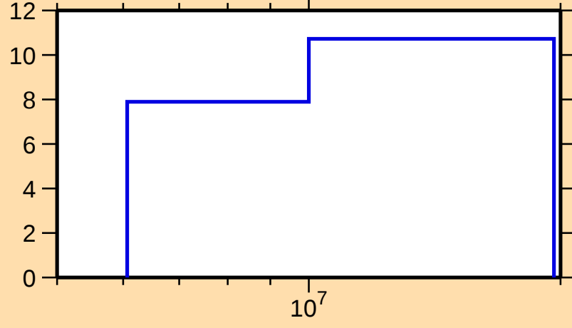
\Delta\sigma/\sigma vs. E for ^{153}\text{Er}(n,\text{tot.})
