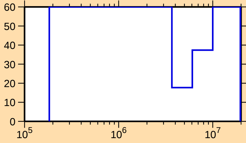
\Delta\sigma/\sigma vs. E for ^{153}\text{Er}(n,\text{inel.})
