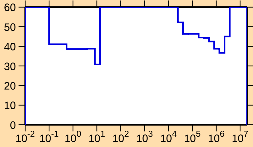
\Delta\sigma/\sigma vs. E for ^{153}\text{Er}(n,\gamma)
