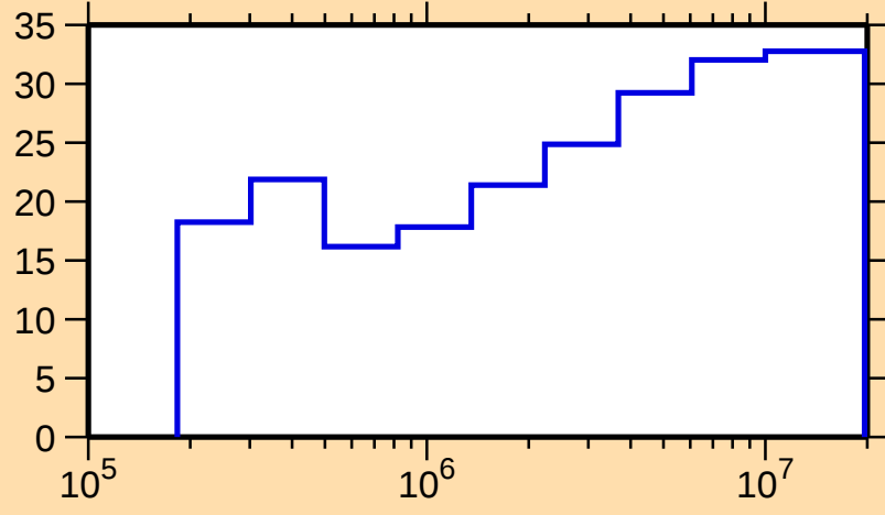
\Delta\sigma/\sigma vs. E for ^{153}\text{Er}(n,\text{el.})
