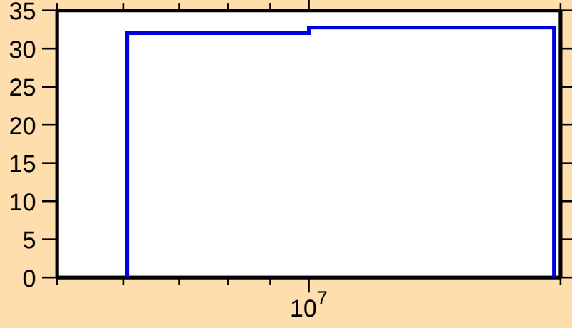
\Delta\sigma/\sigma vs. E for ^{153}\text{Er}(n,\text{el.})
