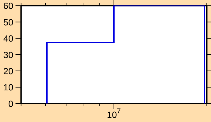
\Delta\sigma/\sigma vs. E for ^{153}\text{Er}(n,\text{inel.})
