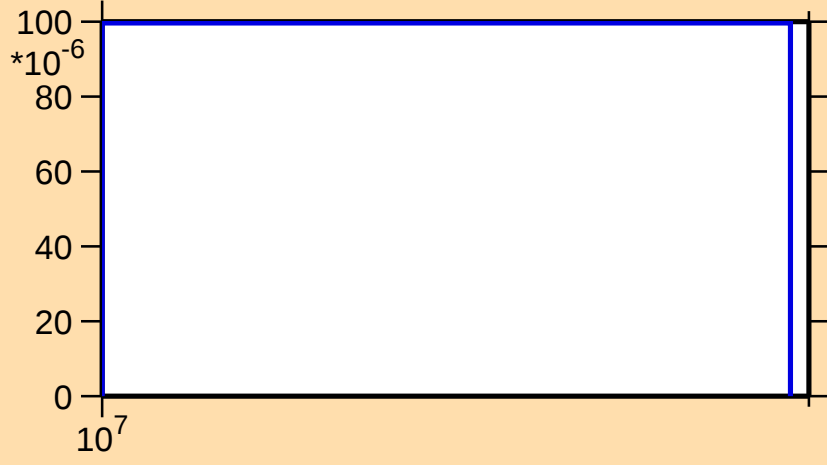
\sigma vs. E for ^{153}\text{Er}(n,2np)
