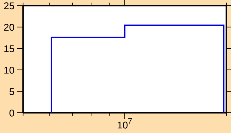
\Delta\sigma/\sigma vs. E for ^{153}\text{Er}(n,\text{nonel.})
