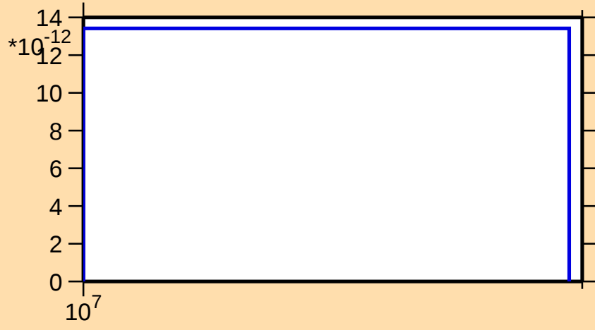
\sigma vs. E for ^{153}\text{Er}(n,\text{nt})
