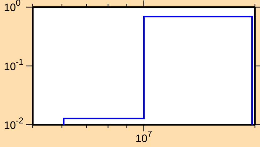
\sigma vs. E for ^{153}\text{Er}(n,2n)
