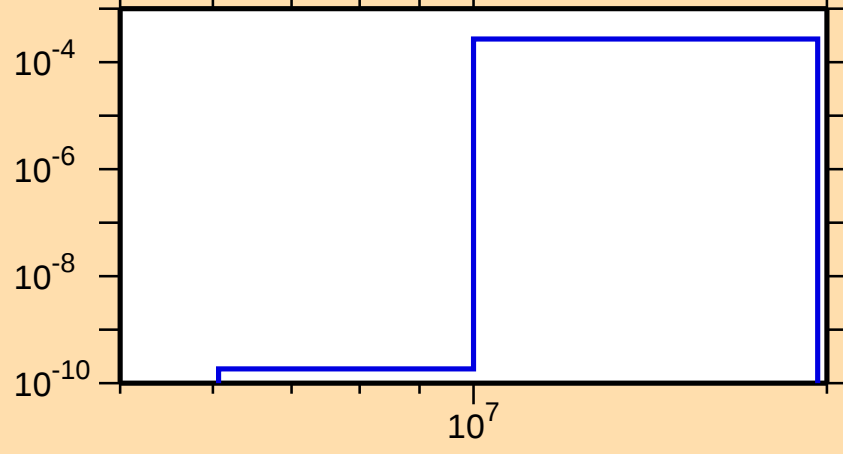
\sigma vs. E for ^{153}\text{Er}(n,t)
