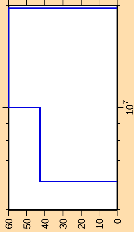
\Delta\sigma/\sigma vs. E for ^{153}\text{Er}(n,n\text{cont.})
