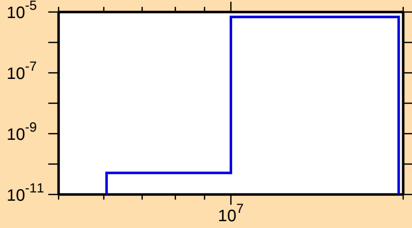
\sigma vs. E for ^{153}\text{Er}(n,\text{He3})
