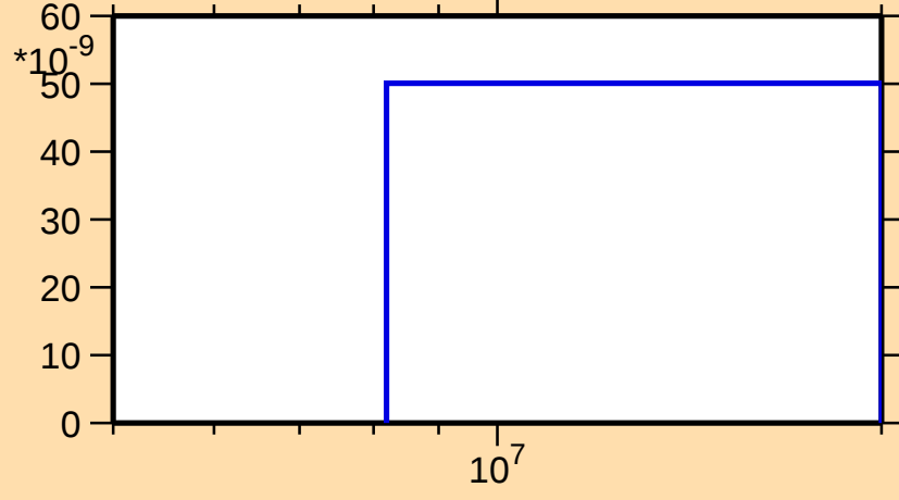
\sigma vs. E for ^{153}\text{Er}(n,\text{pt})
