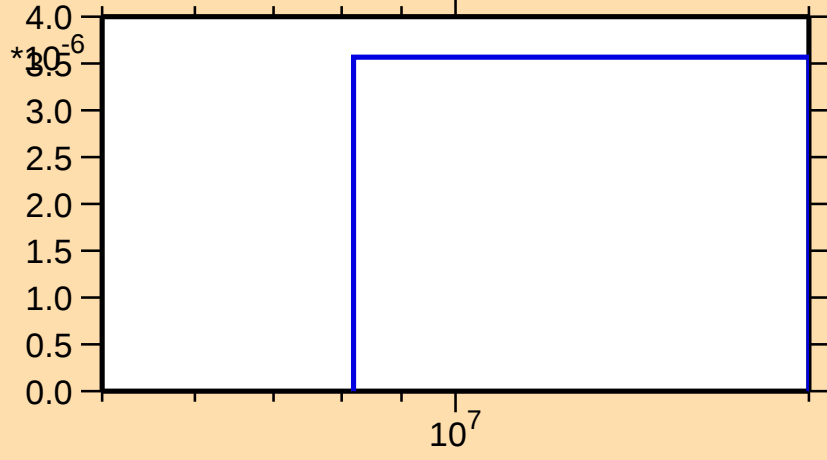
\sigma vs. E for ^{153}\text{Er}(\text{mt } 45)
