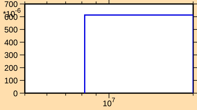
\sigma vs. E for ^{153}\text{Er}(n,2n\alpha)
