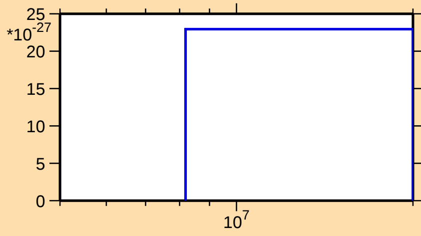
\sigma vs. E for ^{153}\text{Er}(\text{mt 11})
