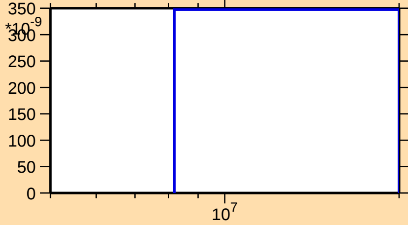
\sigma vs. E for ^{153}\text{Er}(n,\text{pd})
