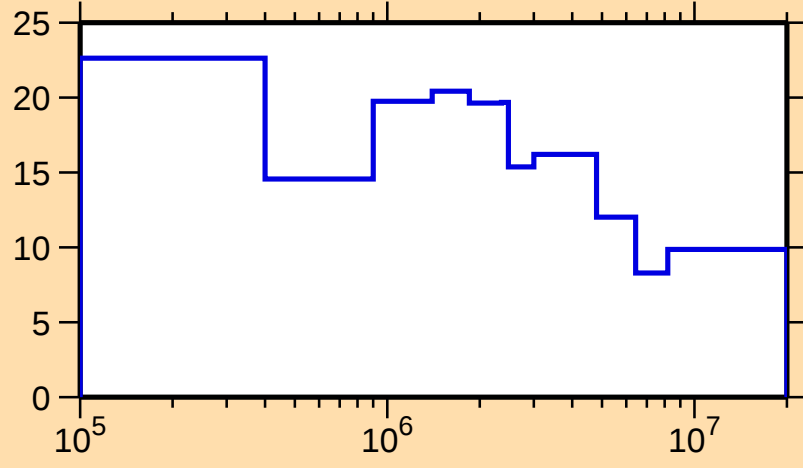
\Delta\sigma/\sigma vs. E for ^{153}\text{Er}(n,\text{tot.})
