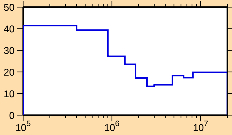
\Delta\sigma/\sigma vs. E for ^{153}\text{Er}(n,\text{nonel.})
