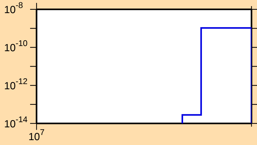
\sigma vs. E for ^{155}\text{Er}(n,nt)
