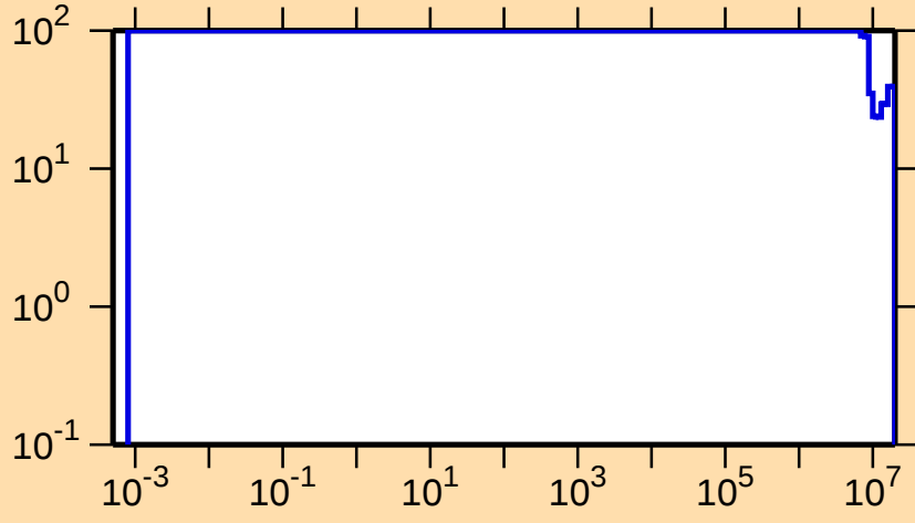
\Delta\sigma/\sigma vs. E for ^{155}\text{Er}(n,p)
