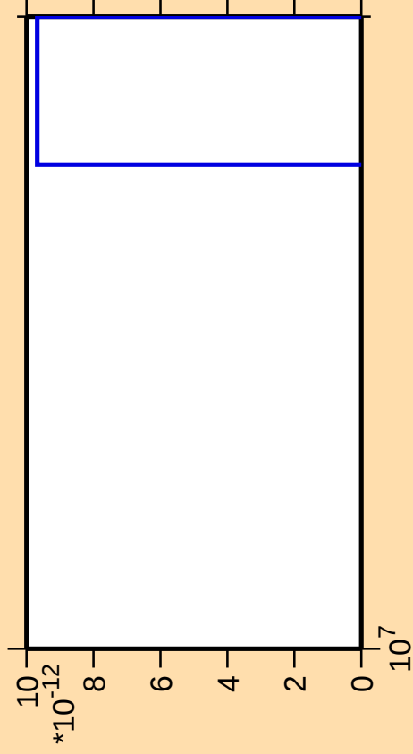
\Delta\sigma/\sigma vs. E for ^{155}\text{Er}(\text{mt } 11)
