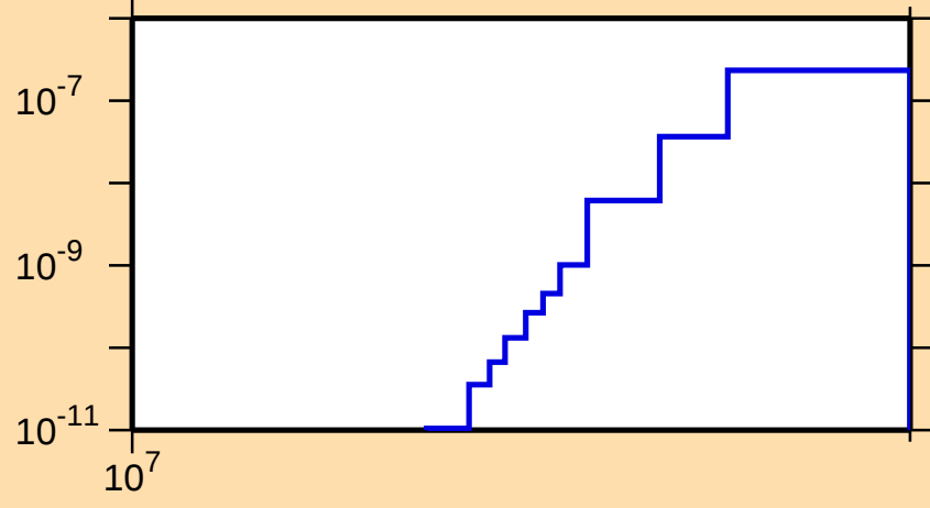
\sigma vs. E for ^{155}\text{Er}(n,\text{pd})
