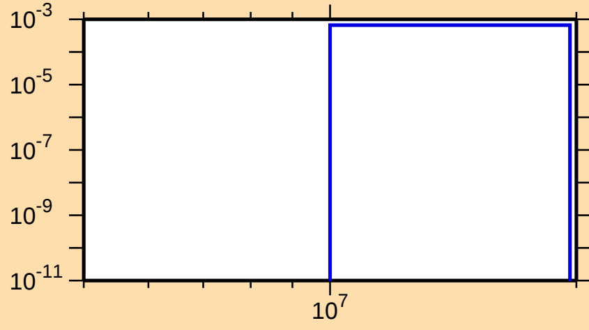
\sigma vs. E for ^{155}\text{Er}(n,2n\alpha)
