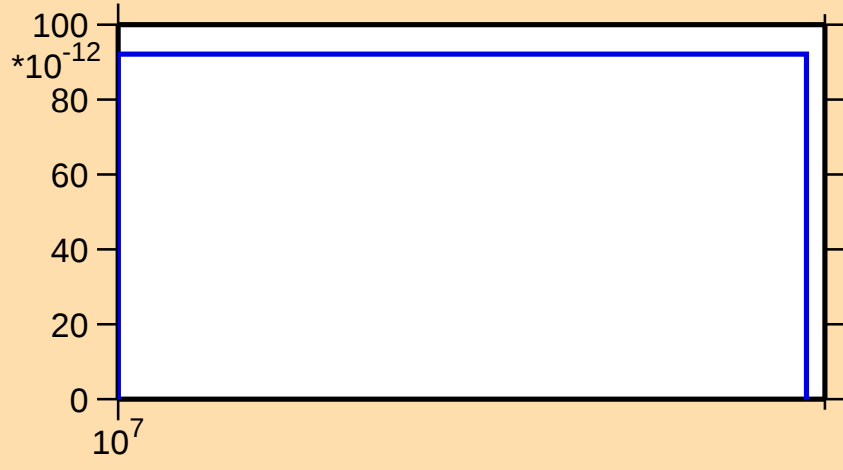
\sigma vs. E for ^{155}\text{Er}(\text{mt117})
