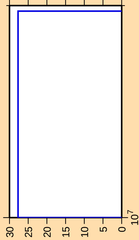
\Delta\sigma/\sigma vs. E for ^{155}\text{Er}(n,\text{nt})
