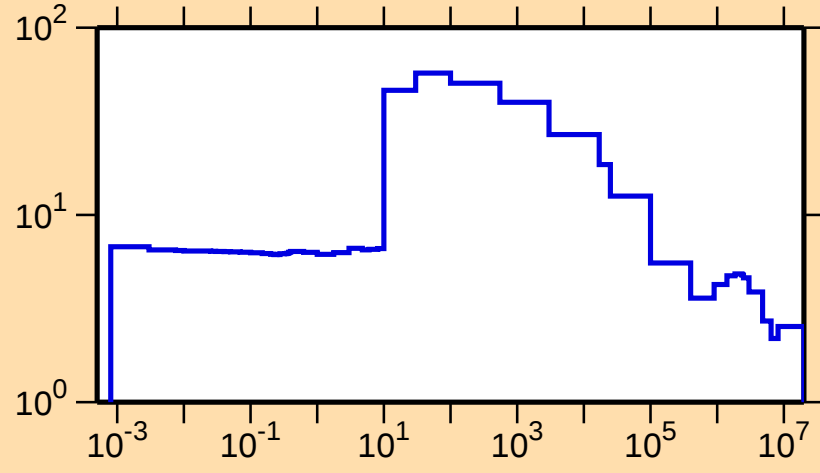
\sigma vs. E for ^{155}\text{Er}(n,\text{el.})
