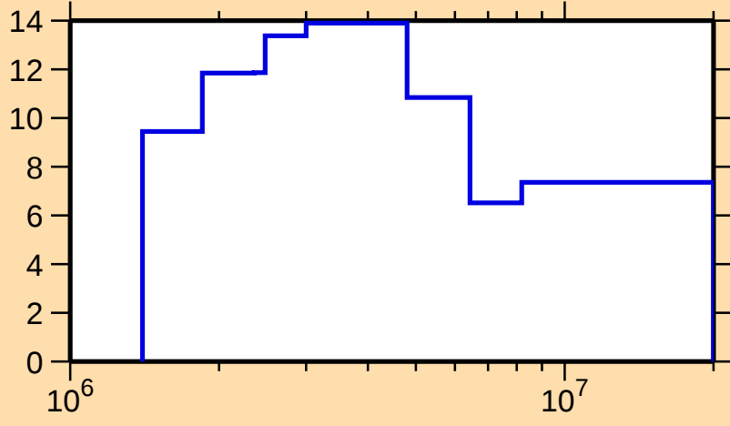
\Delta\sigma/\sigma vs. E for ^{155}\text{Er}(n,\text{el.})
