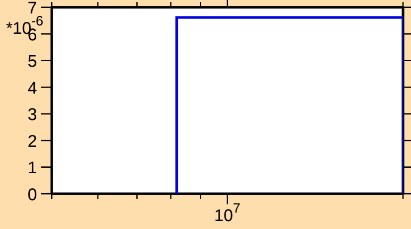
\sigma vs. E for ^{155}\text{Er}(n,3n)
