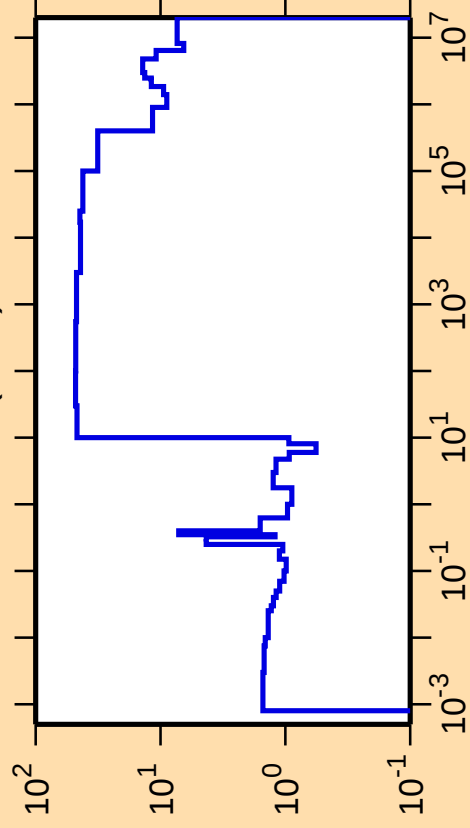
\Delta\sigma/\sigma vs. E for ^{155}\text{Er}(n,\text{el.})
