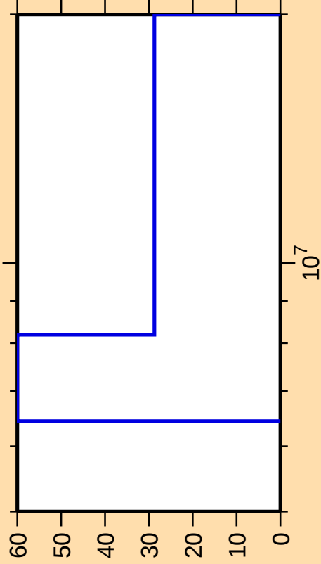
\Delta\sigma/\sigma vs. E for ^{155}\text{Er}(n,p)
