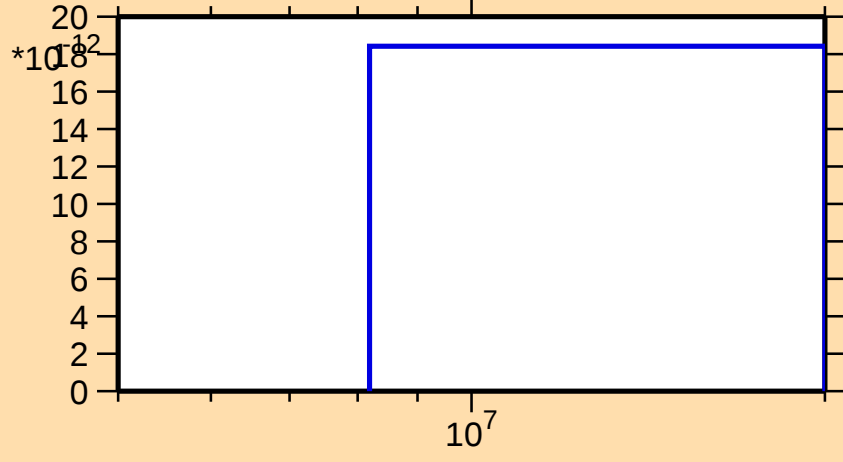
\sigma vs. E for ^{155}\text{Er}(\text{mt } 34)
