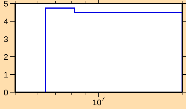
\Delta\sigma/\sigma vs. E for ^{155}\text{Er}(n,\text{nonel.})
