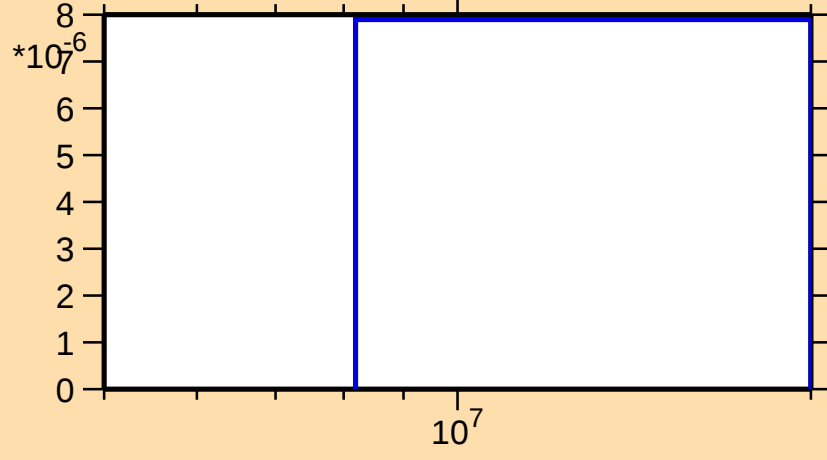
\sigma vs. E for ^{155}\text{Er}(n,2np)
