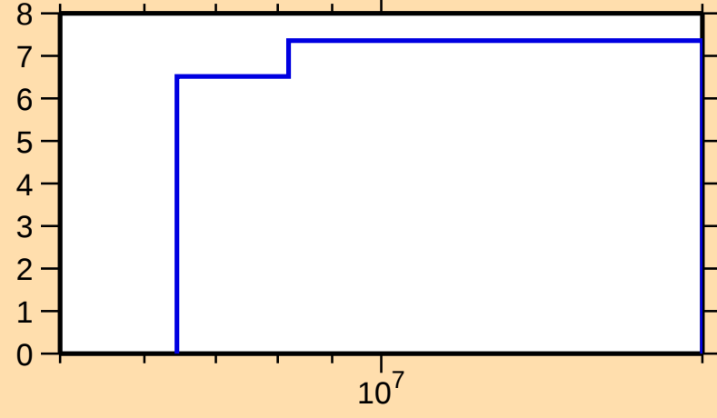
\Delta\sigma/\sigma vs. E for ^{155}\text{Er}(n,\text{el.})
