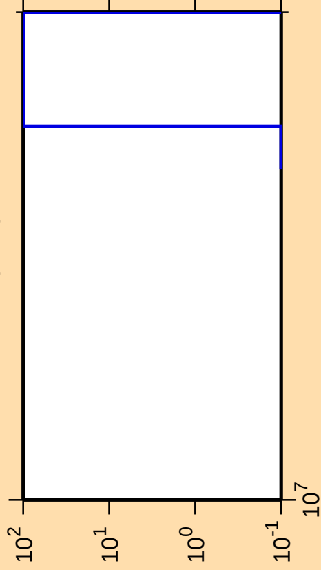
\Delta\sigma/\sigma vs. E for ^{156}\text{Er}(n,nt)
