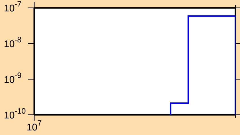
\sigma vs. E for ^{156}\text{Er}(n,\text{nd})
