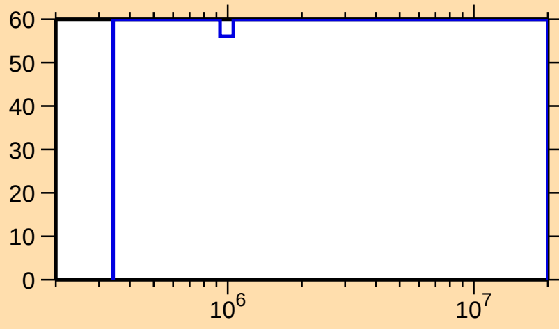
\Delta\sigma/\sigma vs. E for ^{156}\text{Er}(n,n_1)
