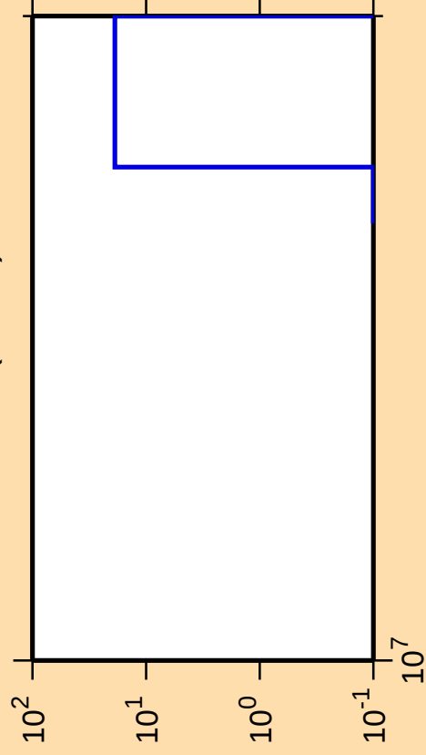
\Delta\sigma/\sigma vs. E for ^{156}\text{Er}(\text{mt } 34)
