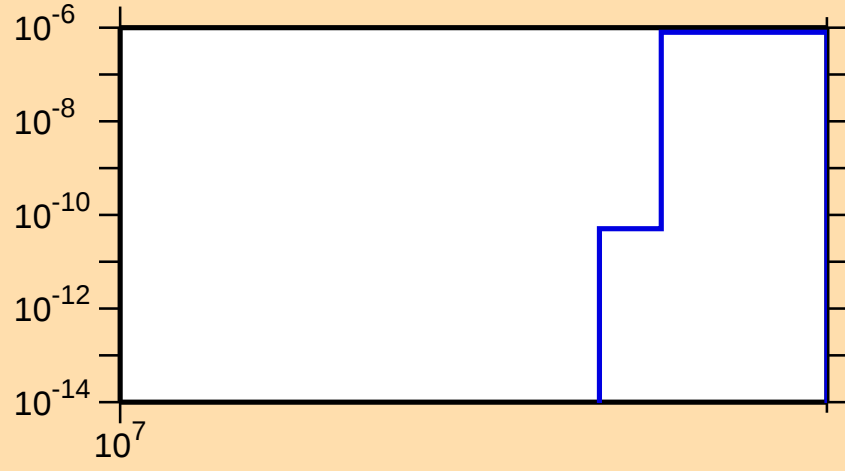
\sigma vs. E for ^{156}\text{Er}(n,2np)
