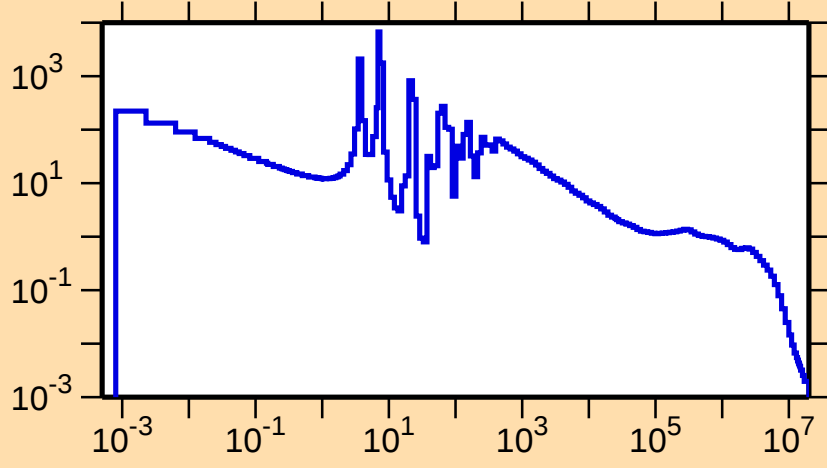
\sigma vs. E for ^{156}\text{Er}(n,\gamma)
