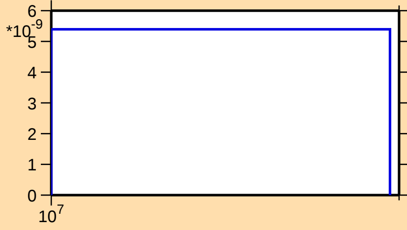
\sigma vs. E for ^{156}\text{Er}(n,2np)
