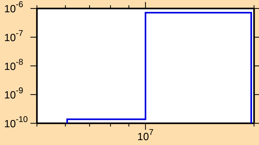
\sigma vs. E for ^{156}\text{Er}(n,p\alpha)
