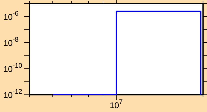
\sigma vs. E for ^{156}\text{Er}(n,2n\alpha)
