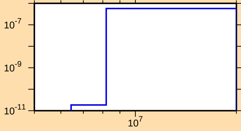
\sigma vs. E for ^{156}\text{Er}(n,p\alpha)
