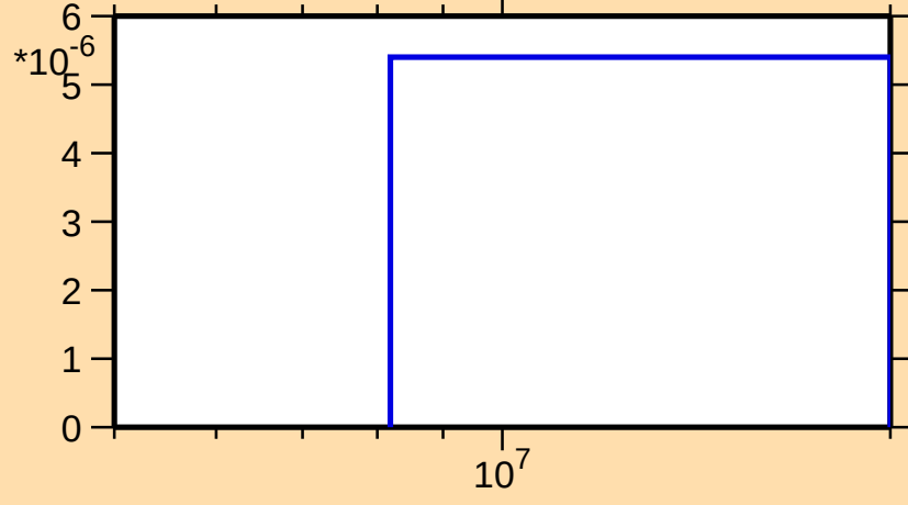
\sigma vs. E for ^{156}\text{Er}(n,3n)
