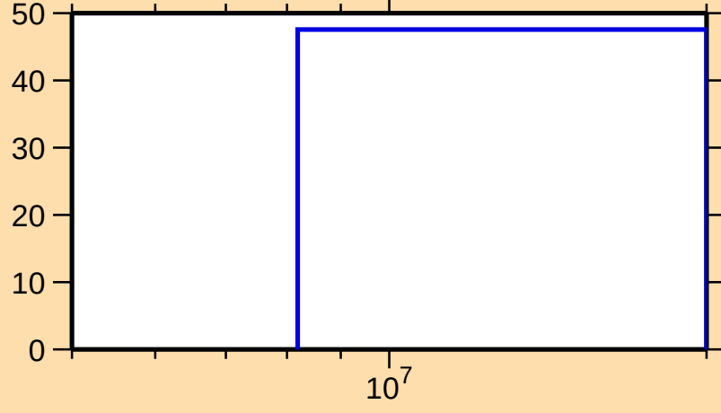
\Delta\sigma/\sigma vs. E for ^{156}\text{Er}(n,\text{inel.})
