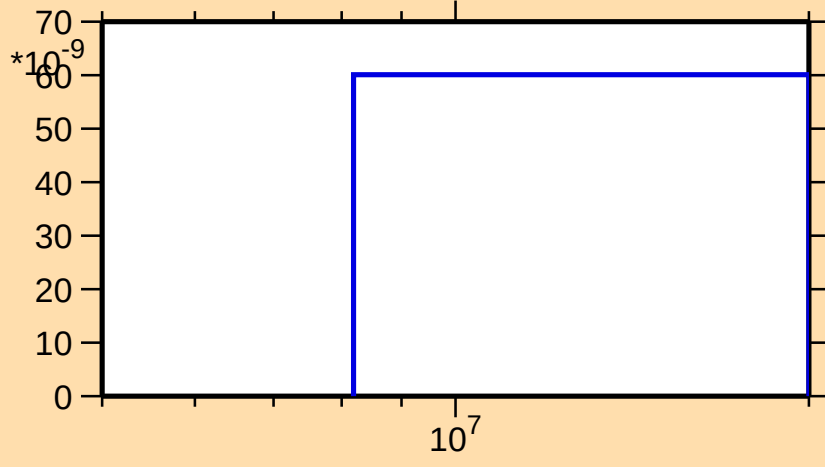
\sigma vs. E for ^{156}\text{Er}(n,\text{He3})
