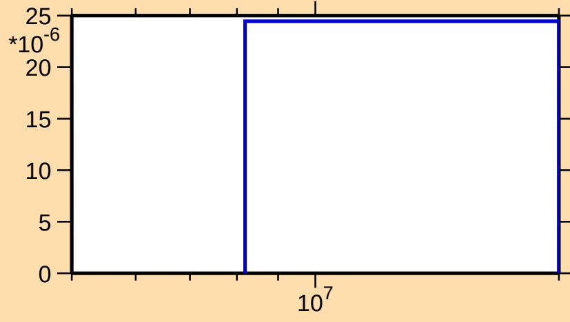
\sigma vs. E for ^{156}\text{Er}(n,t)
