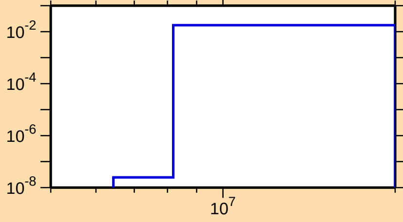
\sigma vs. E for ^{156}\text{Er}(n,np)
