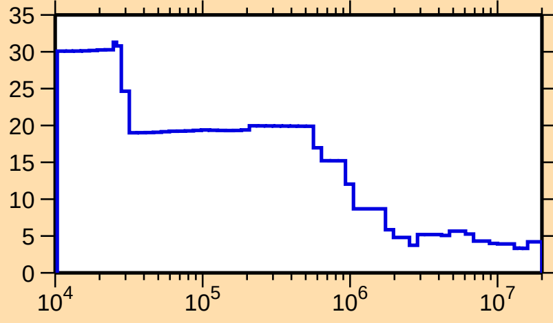
\Delta\sigma/\sigma vs. E for ^{157}\text{Er}(n,\text{nonel.})
