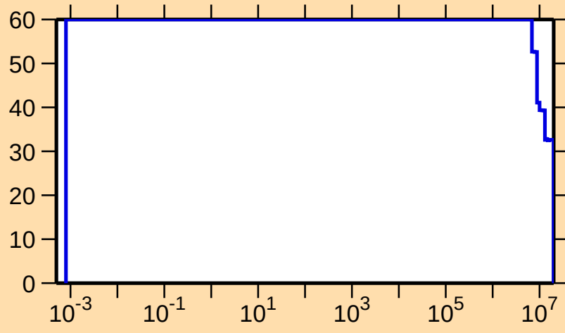
\Delta\sigma/\sigma vs. E for ^{157}\text{Er}(n,p)
