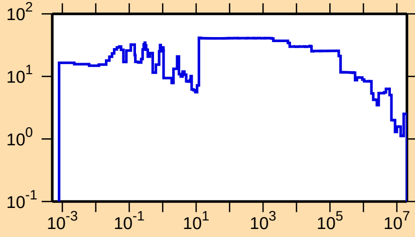
\Delta\sigma/\sigma vs. E for ^{157}\text{Er}(n,\text{tot.})
