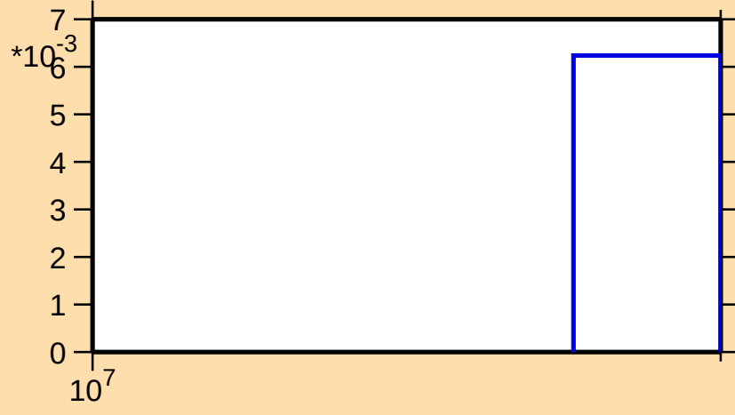
\sigma vs. E for ^{157}\text{Er}(n,3n)
