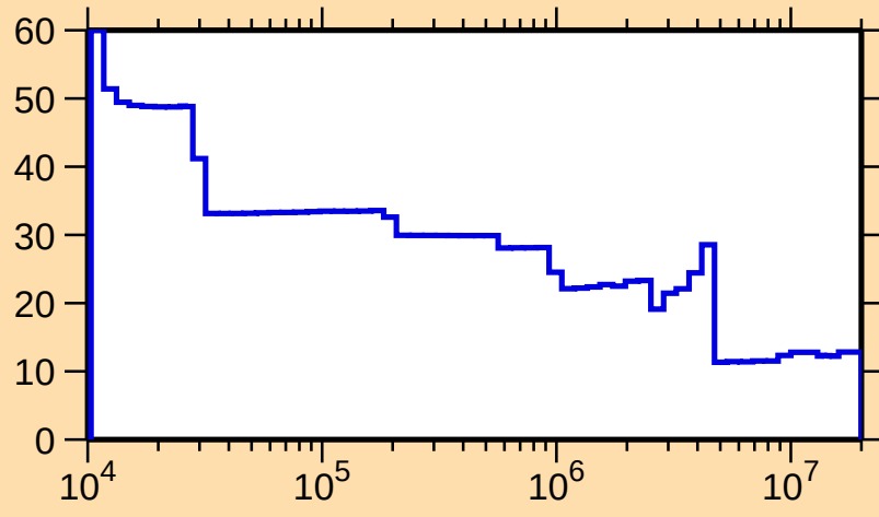
\Delta\sigma/\sigma vs. E for ^{157}\text{Er}(n,n_1)
