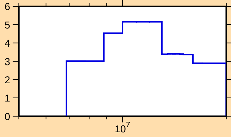
\Delta\sigma/\sigma vs. E for ^{157}\text{Er}(n,\text{el.})
