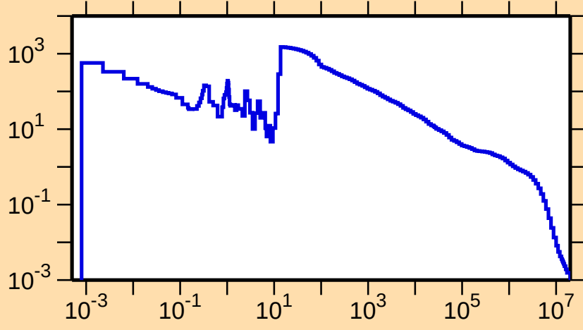
\sigma vs. E for ^{157}\text{Er}(n,\gamma)
