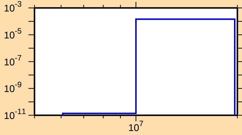
\sigma vs. E for ^{157}\text{Er}(n,t)
