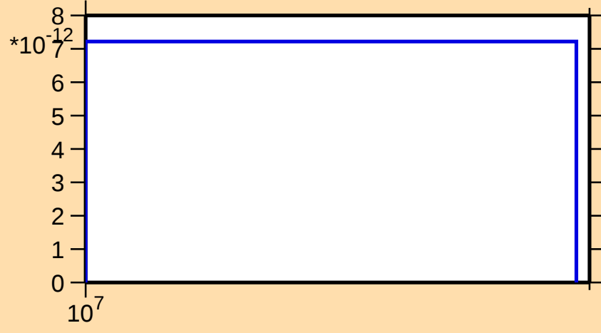
\sigma vs. E for ^{157}\text{Er}(n,\text{nt})
