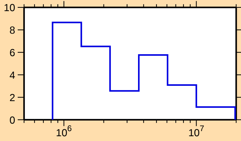
\Delta\sigma/\sigma vs. E for ^{157}\text{Er}(n,\text{tot.})
