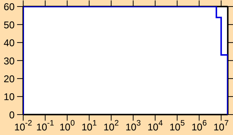
\Delta\sigma/\sigma vs. E for ^{157}\text{Er}(n,p)
