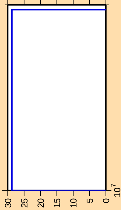
\Delta\sigma/\sigma vs. E for ^{157}\text{Er}(n,\text{nt})
