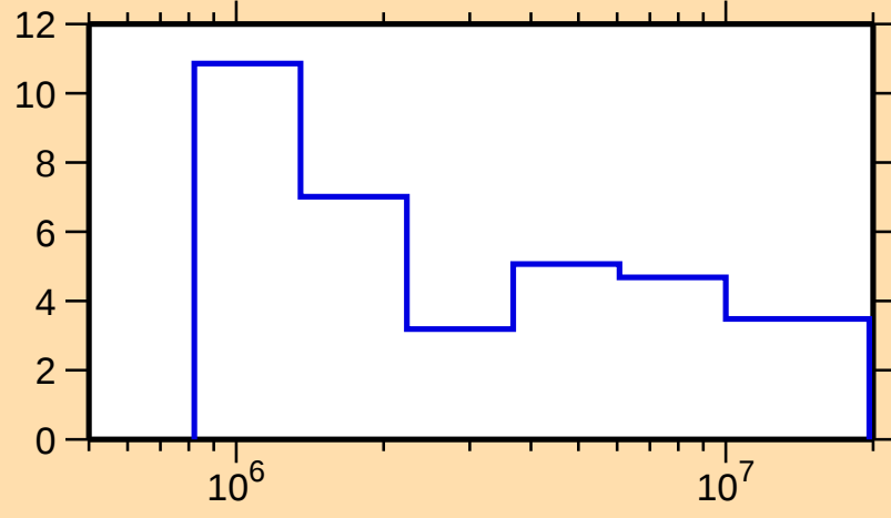
\Delta\sigma/\sigma vs. E for ^{157}\text{Er}(n,n\text{onel.})
