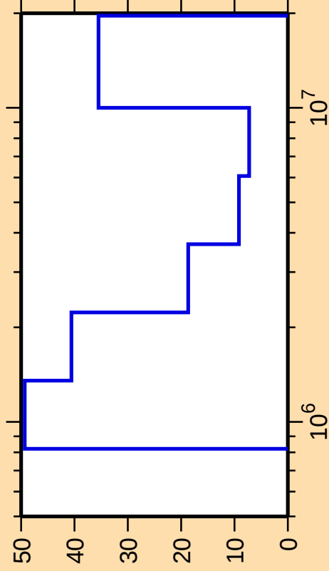
\Delta\sigma/\sigma vs. E for ^{157}\text{Er}(n,\text{ncont.})
