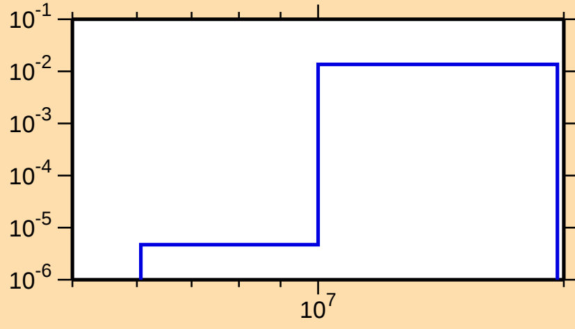
\sigma vs. E for ^{157}\text{Er}(n,np)
