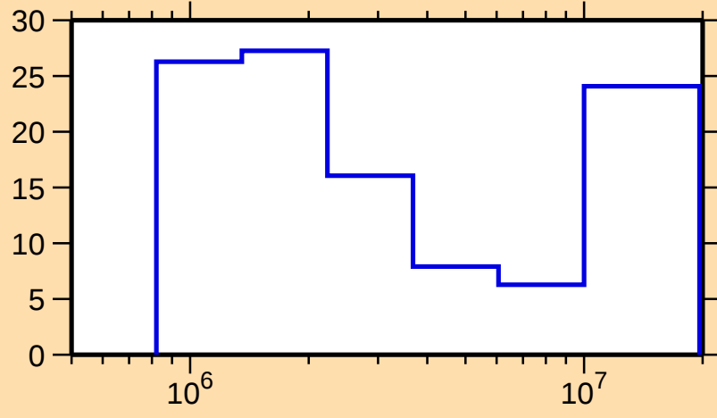
\Delta\sigma/\sigma vs. E for ^{157}\text{Er}(n,\text{inel.})
