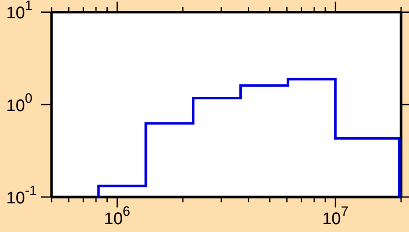
\sigma vs. E for ^{157}\text{Er}(n,n\text{cont.})
