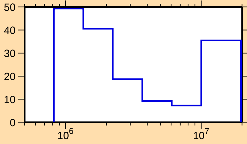
\Delta\sigma/\sigma vs. E for ^{157}\text{Er}(n,n\text{cont.})
