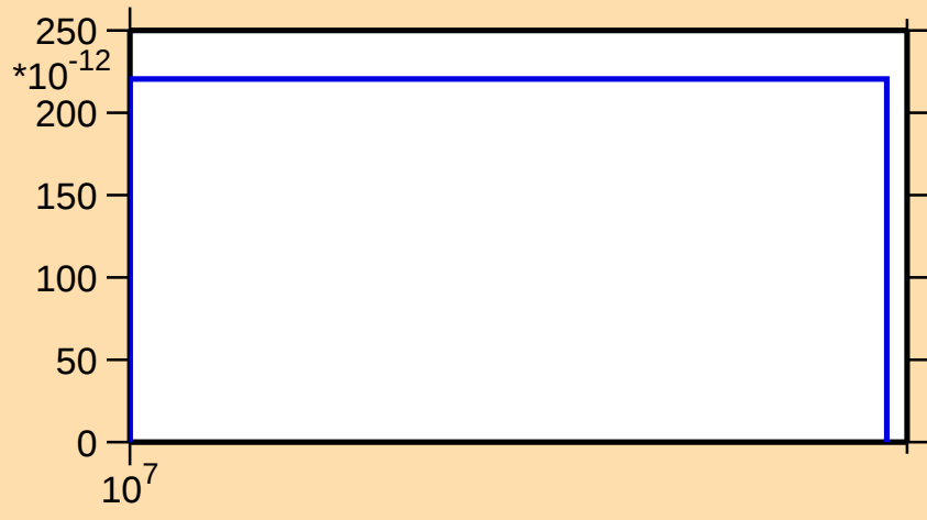
\sigma vs. E for ^{157}\text{Er}(n,\text{pd})
