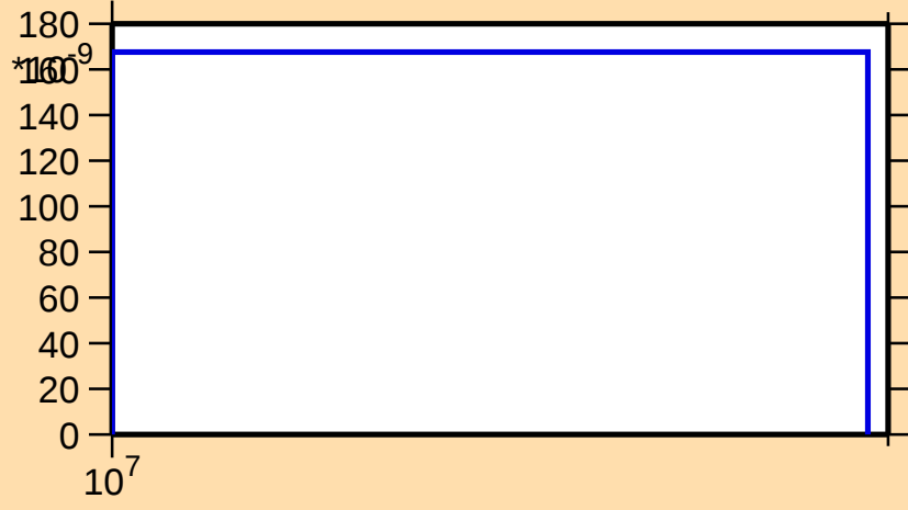
\sigma vs. E for ^{157}\text{Er}(n,\text{nd})
