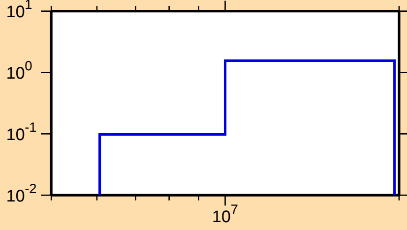
\sigma vs. E for ^{157}\text{Er}(n,2n)
