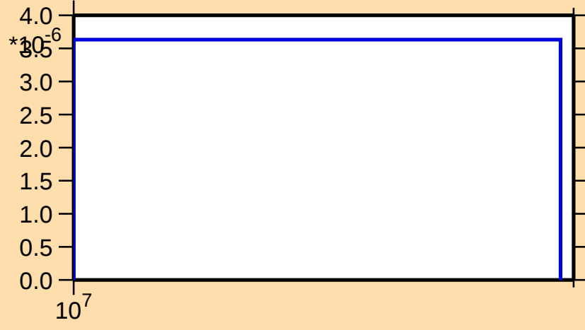
\sigma vs. E for ^{157}\text{Er}(n,2np)
