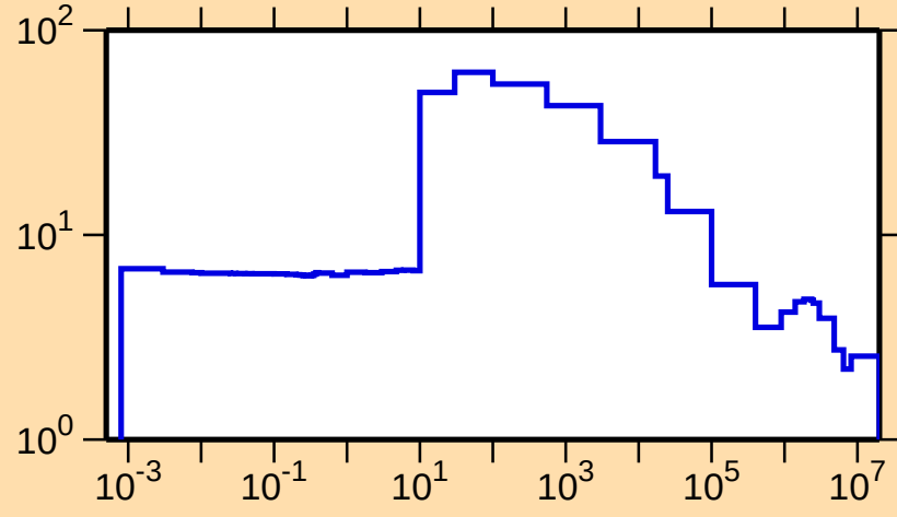
\sigma vs. E for ^{157}\text{Er}(n,\text{el.})
