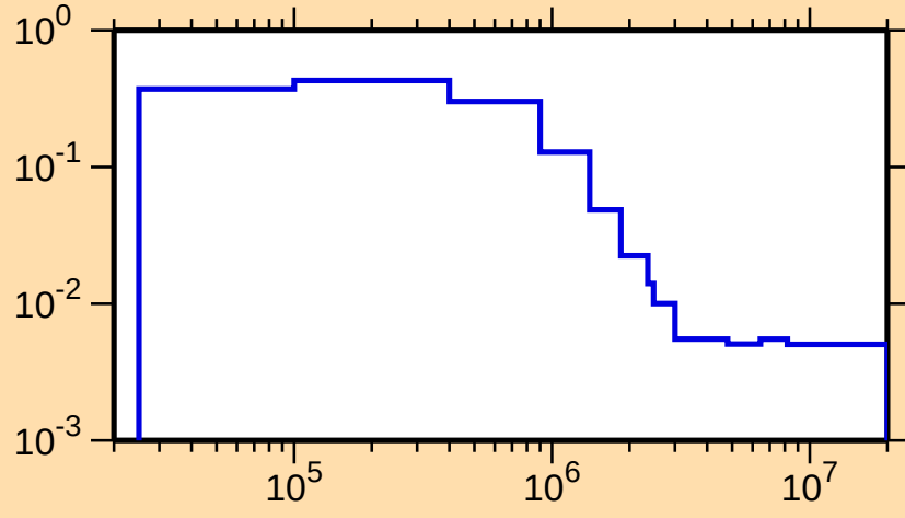
\sigma vs. E for ^{157}\text{Er}(n,n_2)
