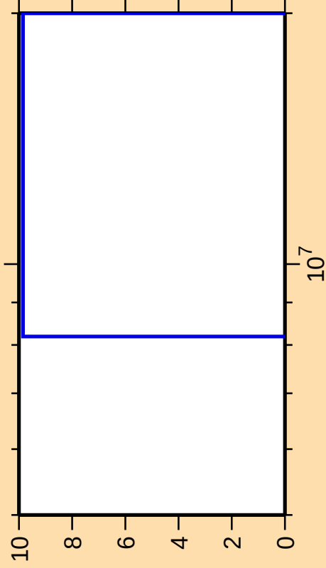
\Delta\sigma/\sigma vs. E for ^{157}\text{Er}(\text{mt } 34)
