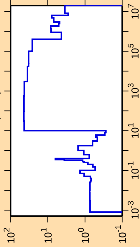
\Delta\sigma/\sigma vs. E for ^{157}\text{Er}(n,\text{el.})
