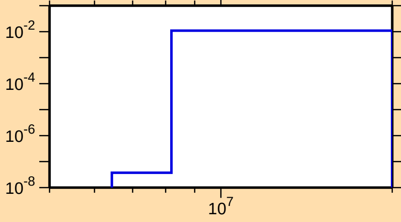
\sigma vs. E for ^{157}\text{Er}(n,np)
