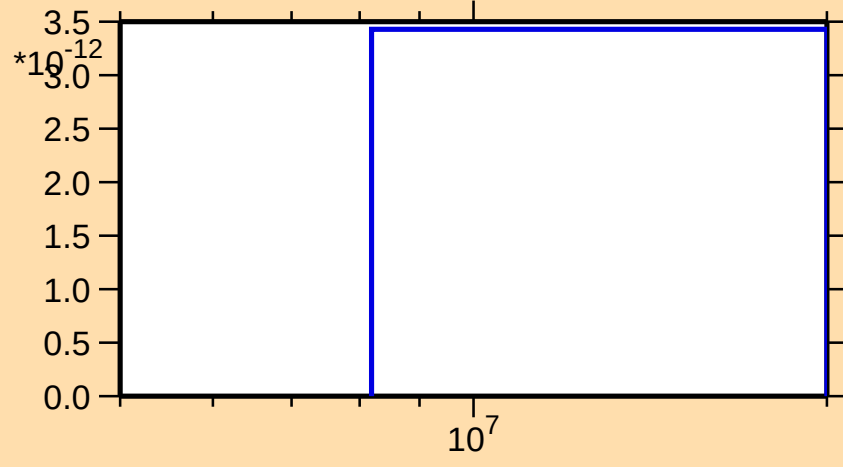
\sigma vs. E for ^{157}\text{Er}(\text{mt } 34)
