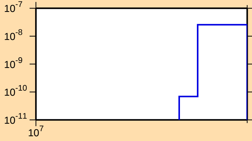
\sigma vs. E for ^{158}\text{Er}(n,\text{nd})
