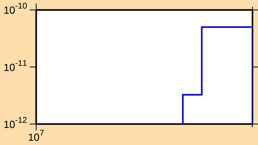
\sigma vs. E for ^{158}\text{Er}(\text{mt117})
