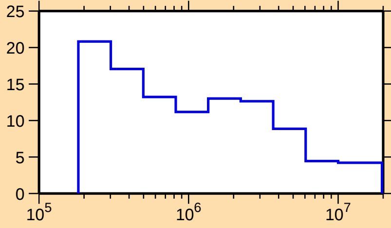
\Delta\sigma/\sigma vs. E for ^{158}\text{Er}(n,\text{tot.})
