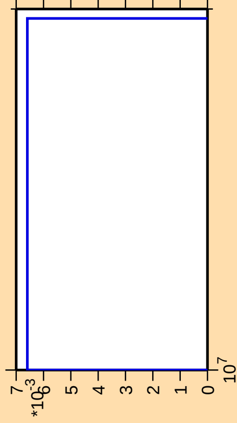
\Delta\sigma/\sigma vs. E for ^{158}\text{Er} (mt 34)
