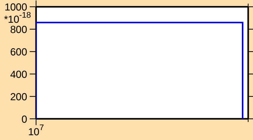
\sigma vs. E for ^{158}\text{Er} (mt 34)
