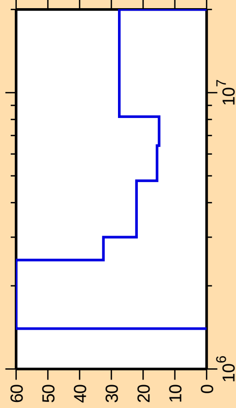
\Delta\sigma/\sigma vs. E for ^{158}\text{Er}(n,\text{ncont.})
