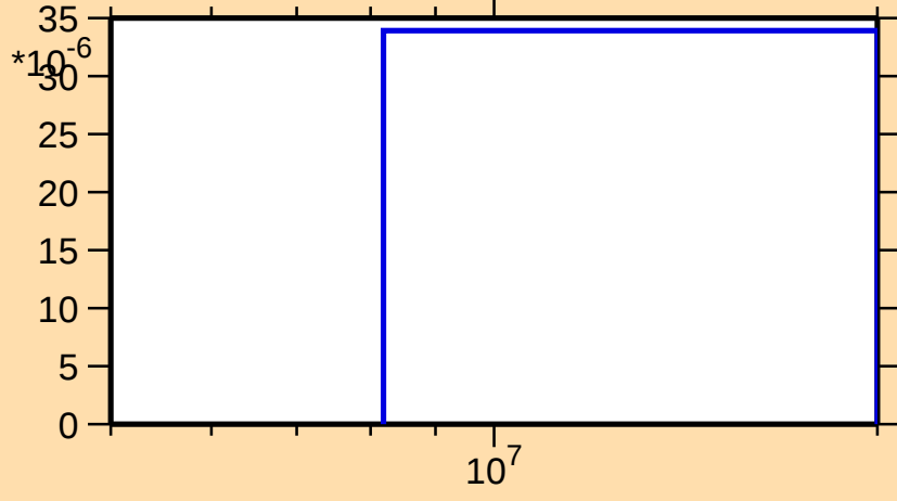
\sigma vs. E for ^{158}\text{Er}(n,3n)
