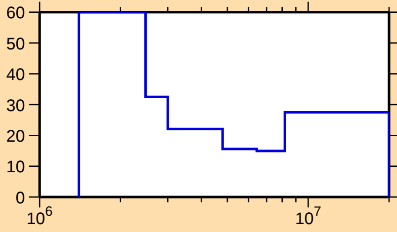
\Delta\sigma/\sigma vs. E for ^{158}\text{Er}(n,\text{ncont.})
