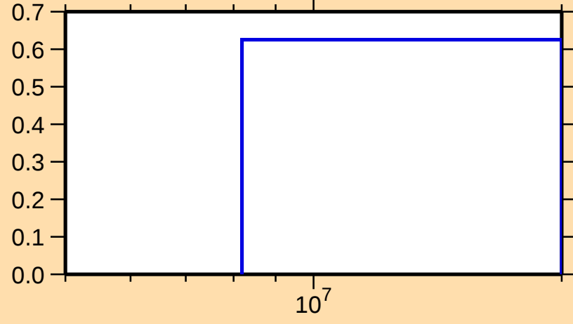
\sigma vs. E for ^{158}\text{Er}(n,2n)
