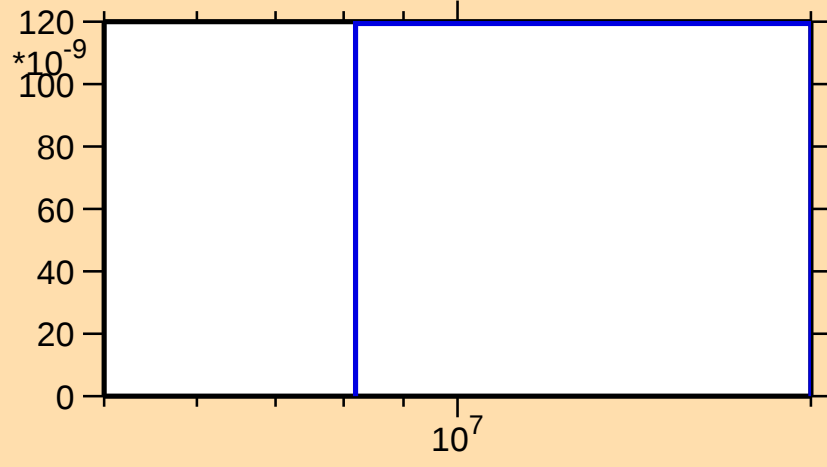
\sigma vs. E for ^{158}\text{Er}(n,2n\alpha)
