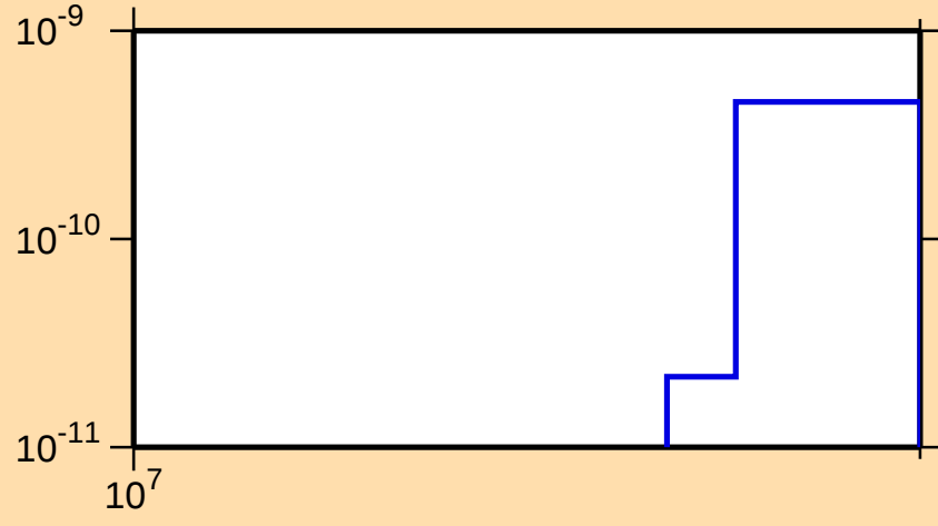
\sigma vs. E for ^{159}\text{Er}(n,\text{pd})
