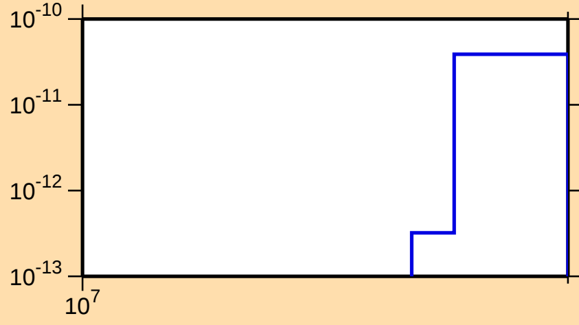
\sigma vs. E for ^{159}\text{Er}(\text{mt } 34)
