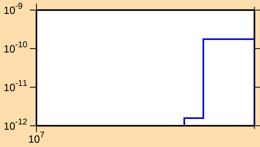
\sigma vs. E for ^{159}\text{Er}(n,\text{pt})
