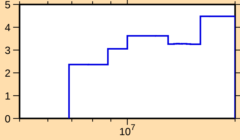
\Delta\sigma/\sigma vs. E for ^{159}\text{Er}(n,\text{tot.})
