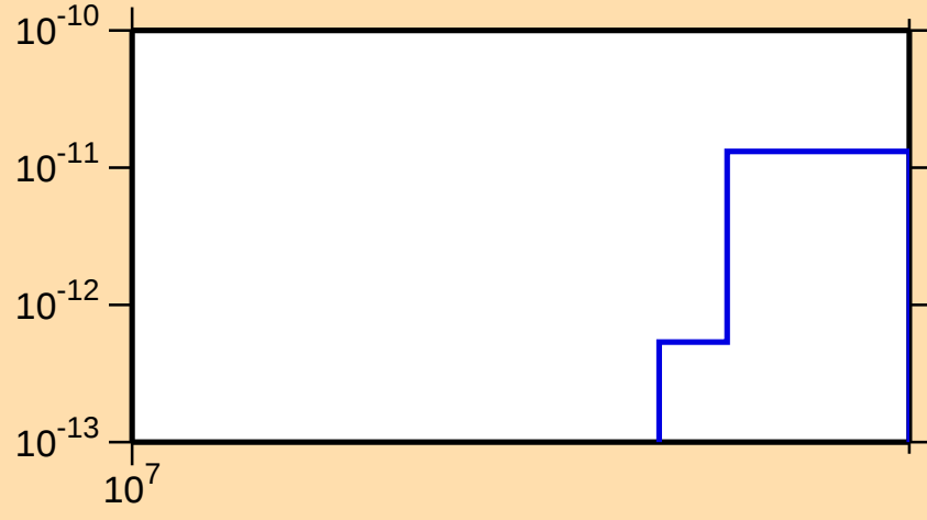
\sigma vs. E for ^{159}\text{Er} (mt 45)
