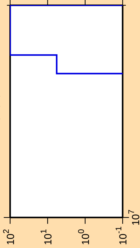
\Delta\sigma/\sigma vs. E for ^{159}\text{Er}(n,\text{pt})
