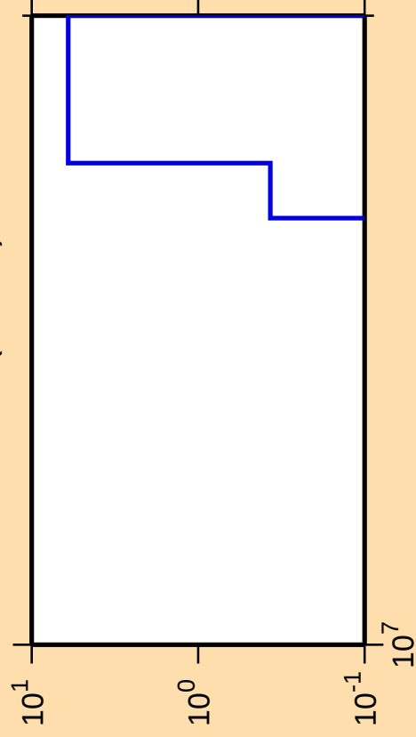
\Delta\sigma/\sigma vs. E for ^{159}\text{Er}(\text{mt117})
