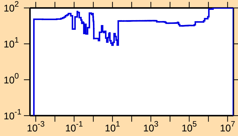
\Delta\sigma/\sigma vs. E for ^{159}\text{Er}(n,\gamma)
