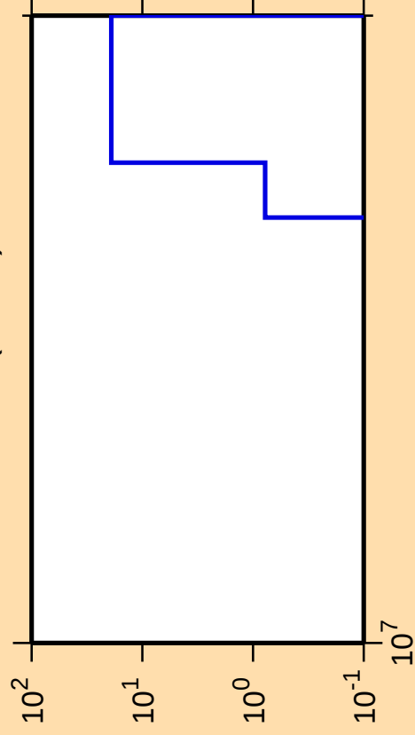
\Delta\sigma/\sigma vs. E for ^{159}\text{Er} (mt 45)
