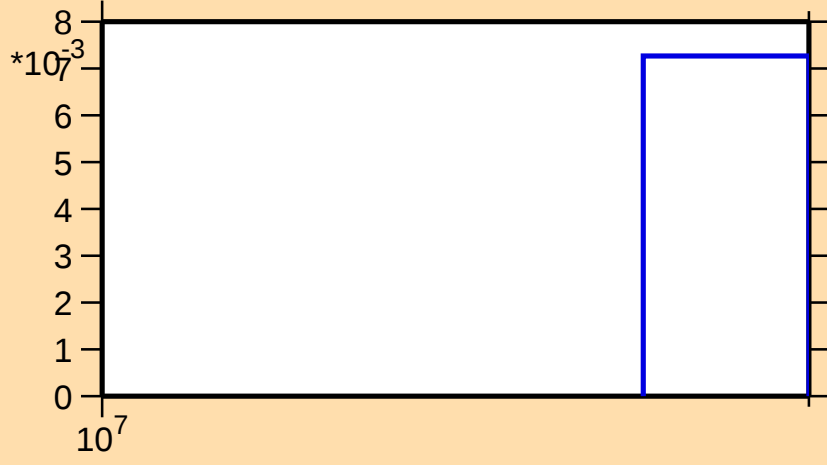
\sigma vs. E for ^{159}\text{Er}(n,3n)
