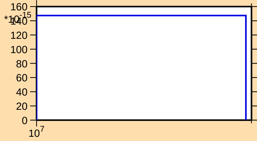
\sigma vs. E for ^{159}\text{Er}(\text{mt 45})
