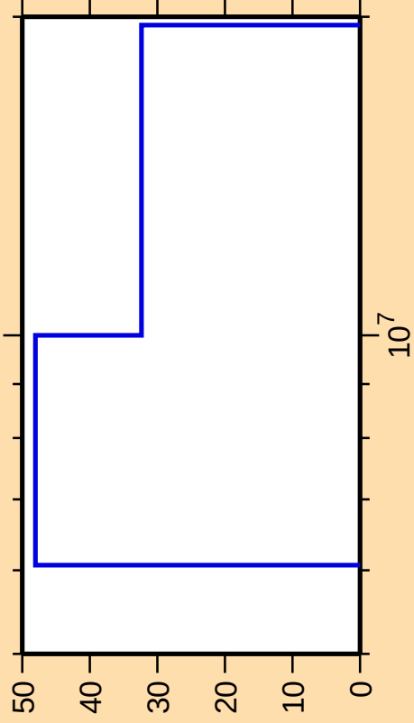
\Delta\sigma/\sigma vs. E for ^{159}\text{Er}(n,2n)
