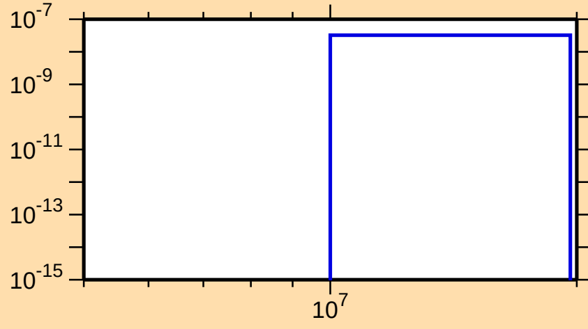
\sigma vs. E for ^{159}\text{Er}(n,\text{He3})
