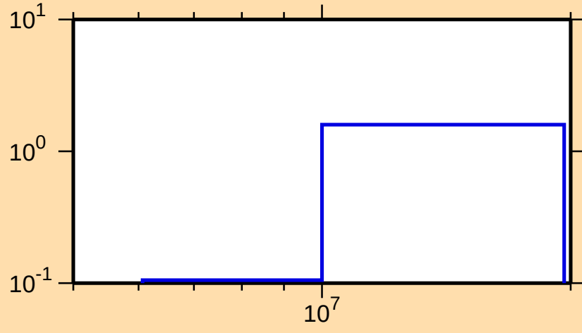
\sigma vs. E for ^{159}\text{Er}(n,2n)
