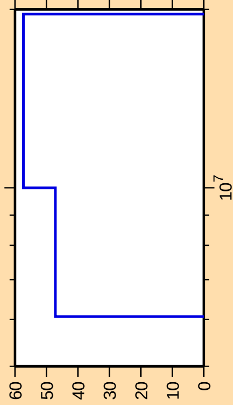
\Delta\sigma/\sigma vs. E for ^{159}\text{Er}(n,n_1)
