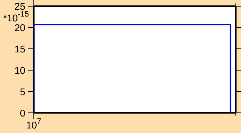
\sigma vs. E for ^{159}\text{Er}(\text{mt117})
