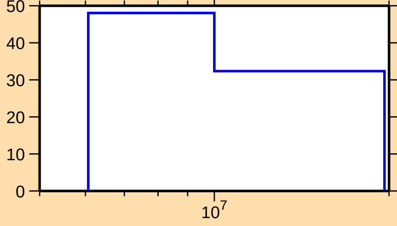
\Delta\sigma/\sigma vs. E for ^{159}\text{Er}(n,2n)
