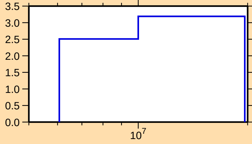
\Delta\sigma/\sigma vs. E for ^{159}\text{Er}(n,\text{tot.})
