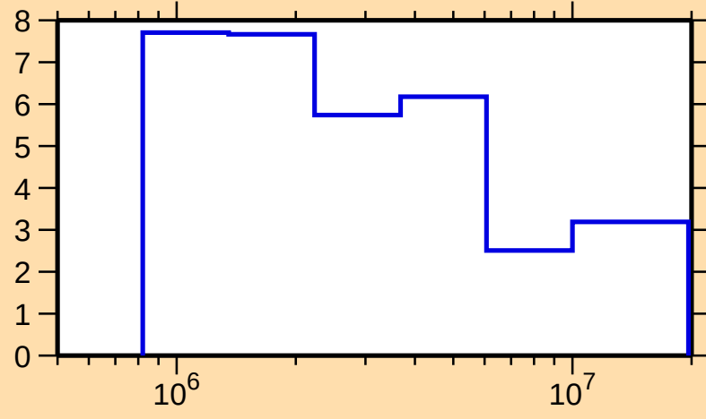
\Delta\sigma/\sigma vs. E for ^{159}\text{Er}(\text{n},\text{tot.})
