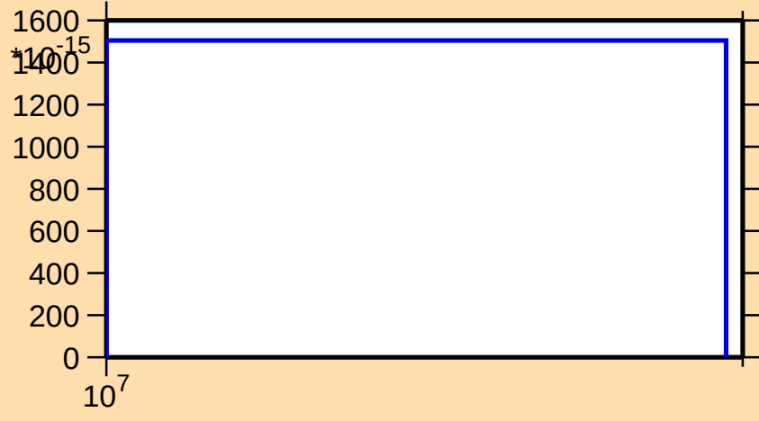
\sigma vs. E for ^{159}\text{Er}(n,\text{pt})
