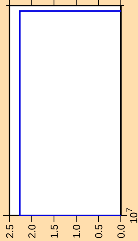
\Delta\sigma/\sigma vs. E for ^{159}\text{Er}(\text{mt } 34)
