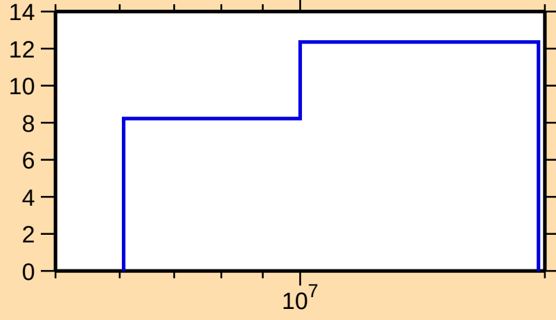
\Delta\sigma/\sigma vs. E for ^{159}\text{Er}(n,\text{el.})
