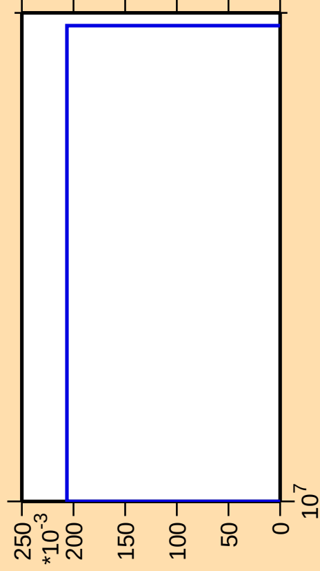
\Delta\sigma/\sigma vs. E for ^{159}\text{Er}(\text{mt 45})
