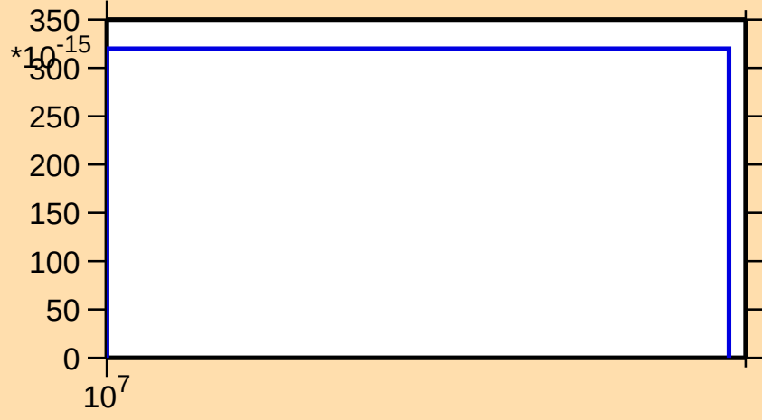
\sigma vs. E for ^{159}\text{Er}(\text{mt } 34)
