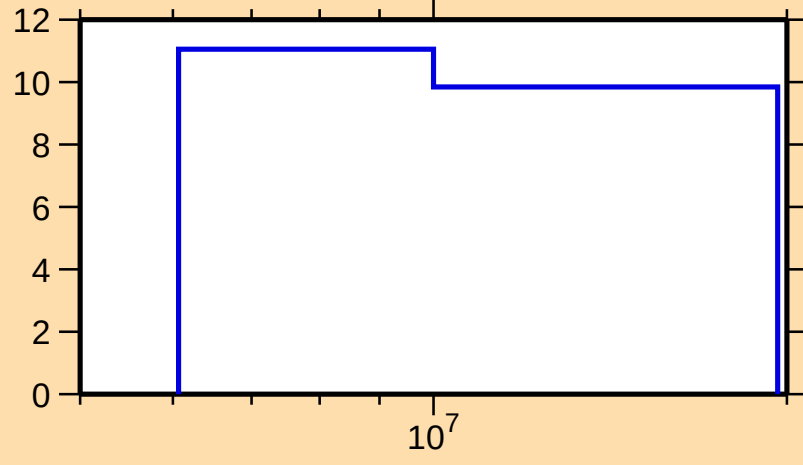
\Delta\sigma/\sigma vs. E for ^{159}\text{Er}(n,\text{nonel.})
