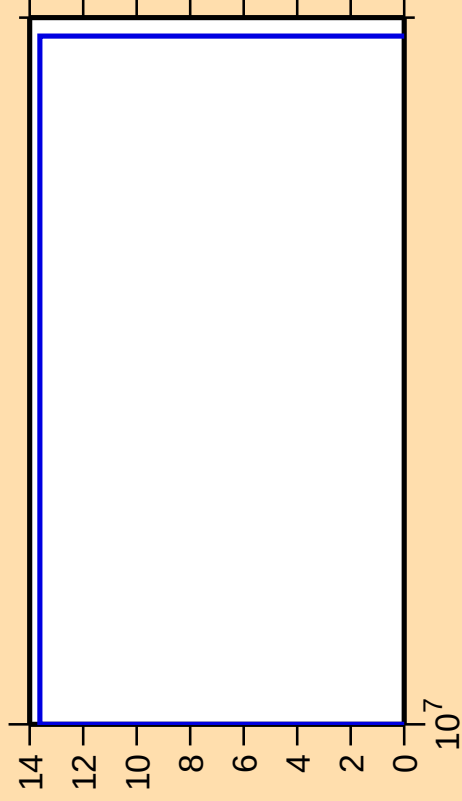
\Delta\sigma/\sigma vs. E for ^{159}\text{Er}(n,\text{pd})
