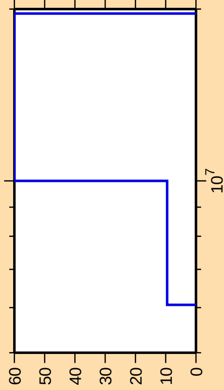
\Delta\sigma/\sigma vs. E for ^{159}\text{Er}(n,n\text{cont.})
