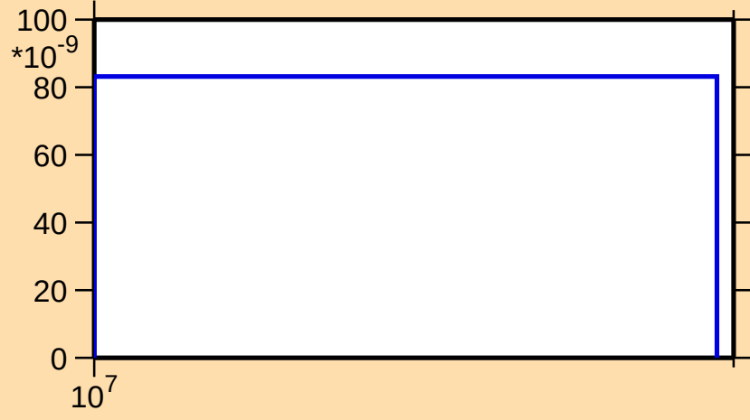
\sigma vs. E for ^{159}\text{Er}(n,\text{nd})
