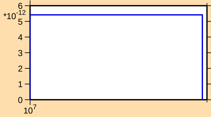
\sigma vs. E for ^{159}\text{Er}(n,\text{pd})
