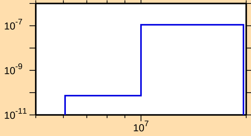
\sigma vs. E for ^{159}\text{Er}(n,p\alpha)
