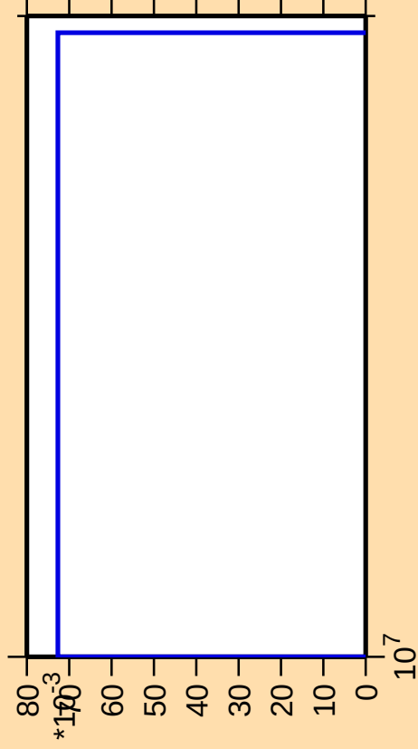
\Delta\sigma/\sigma vs. E for ^{159}\text{Er}(\text{mt117})
