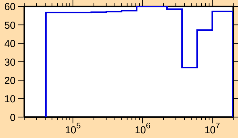
\Delta\sigma/\sigma vs. E for ^{159}\text{Er}(n,n_1)
