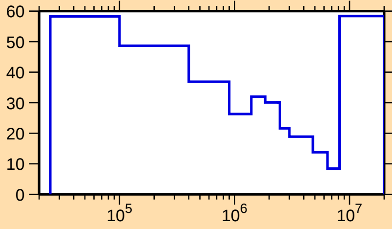
\Delta\sigma/\sigma vs. E for ^{159}\text{Er}(n,\text{inel.})
