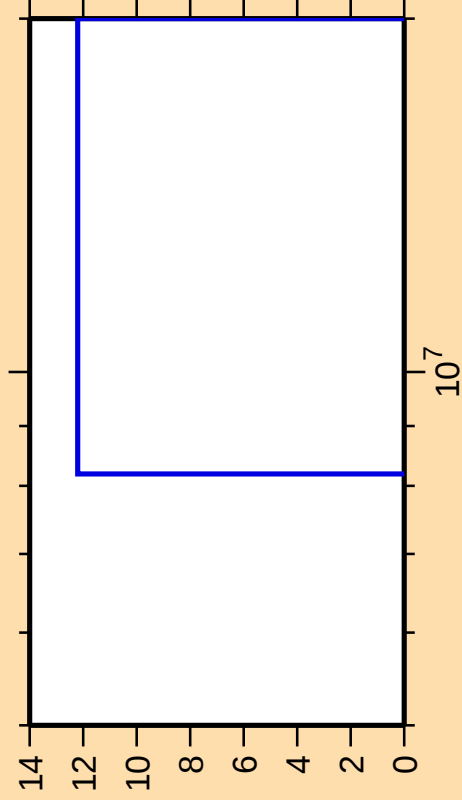
\Delta\sigma/\sigma vs. E for ^{159}\text{Er}(n,nt)
