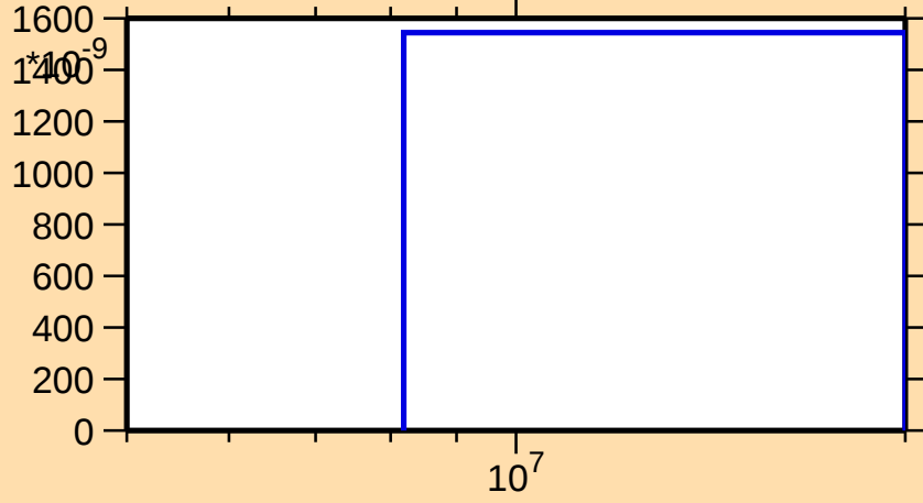
\sigma vs. E for ^{159}\text{Er}(n,2n\alpha)
