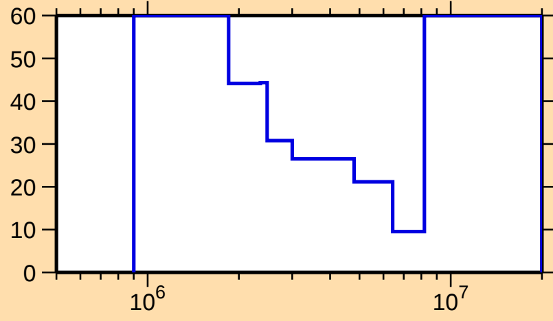
\Delta\sigma/\sigma vs. E for ^{159}\text{Er}(n,n\text{cont.})
