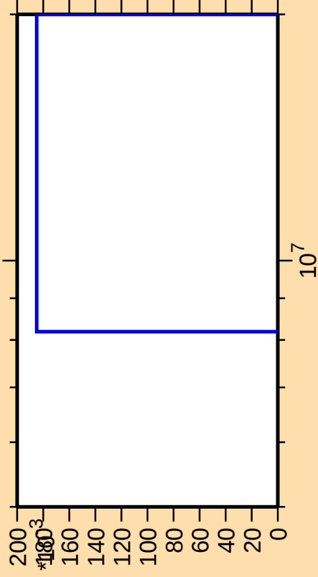
\Delta\sigma/\sigma vs. E for ^{159}\text{Er} (mt 45)
