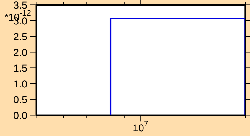
\sigma vs. E for ^{159}\text{Er}(n,nt)
