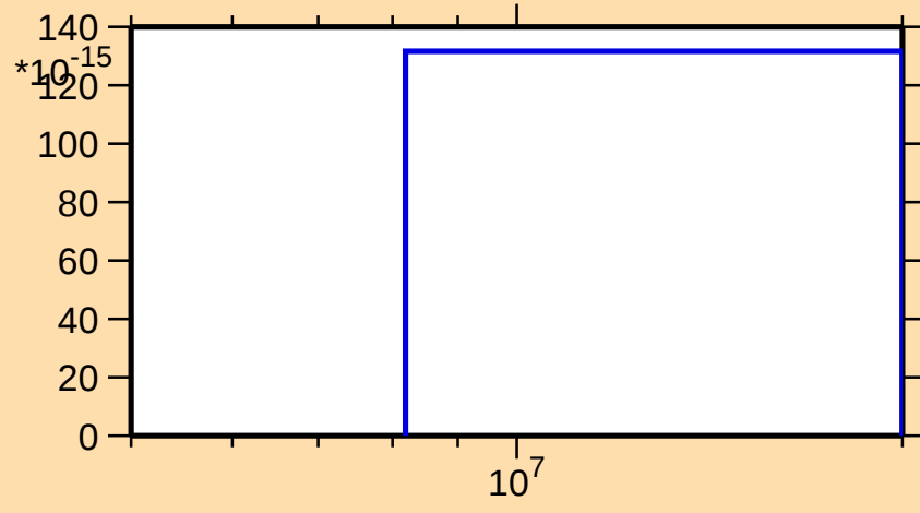
\sigma vs. E for ^{159}\text{Er} (mt 45)
