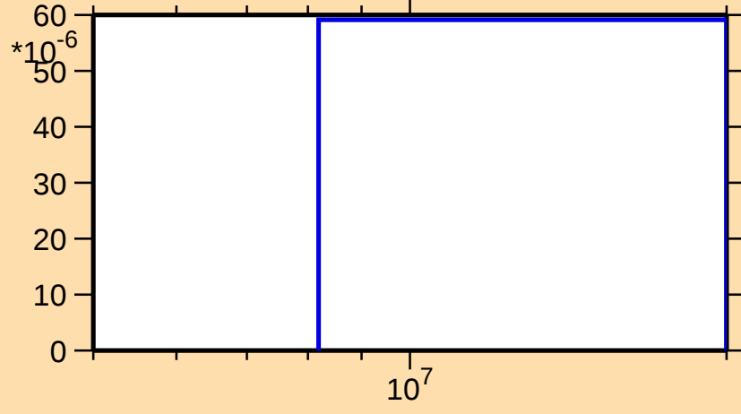
\sigma vs. E for ^{159}\text{Er}(n,3n)
