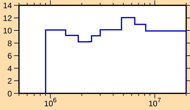
\Delta\sigma/\sigma vs. E for ^{159}\text{Er}(n,n\text{onel.})
