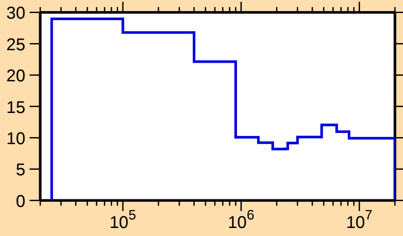
\Delta\sigma/\sigma vs. E for ^{159}\text{Er}(n,\text{nonel.})
