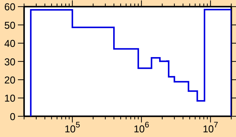
\Delta\sigma/\sigma vs. E for ^{159}\text{Er}(n,\text{inel.})
