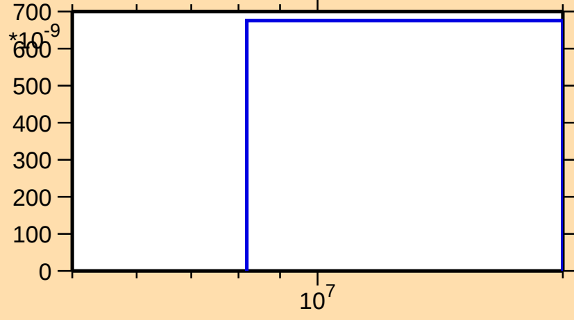
\sigma vs. E for ^{159}\text{Er}(n,2np)
