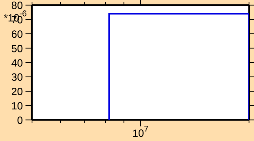
\sigma vs. E for ^{159}\text{Er}(n,t)
