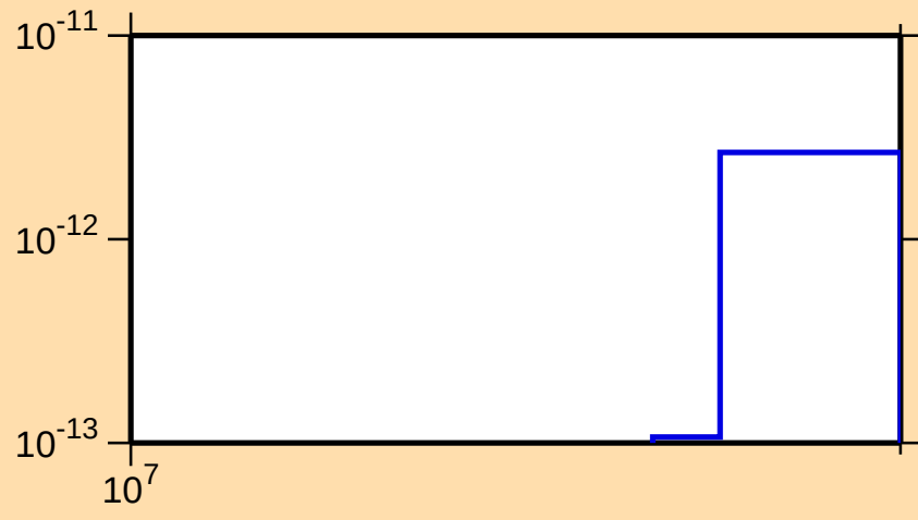
\sigma vs. E for ^{160}\text{Er}(\text{mt117})
