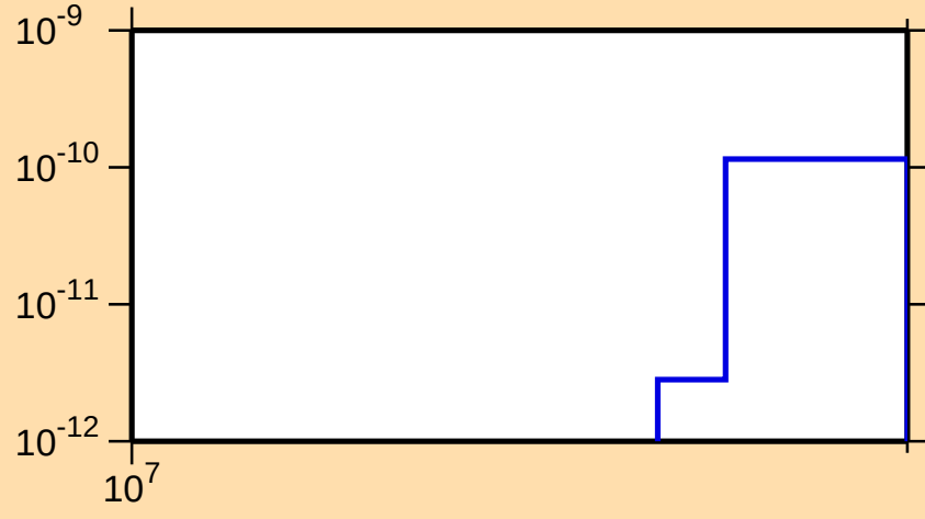
\sigma vs. E for ^{160}\text{Er}(n,\text{pd})
