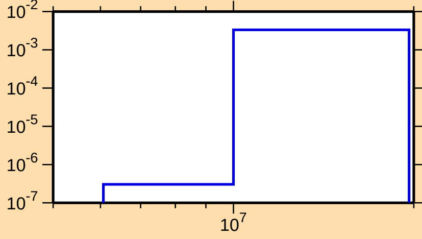
\sigma vs. E for ^{160}\text{Er}(n,np)
