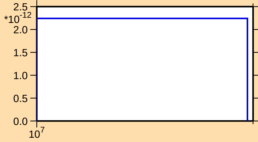
\sigma vs. E for ^{160}\text{Er}(n,\text{nt})
