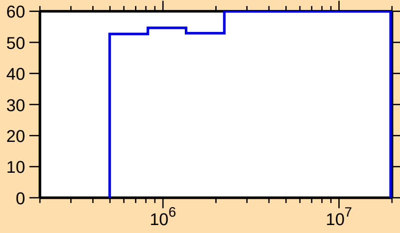
\Delta\sigma/\sigma vs. E for ^{160}\text{Er}(n,\gamma)
