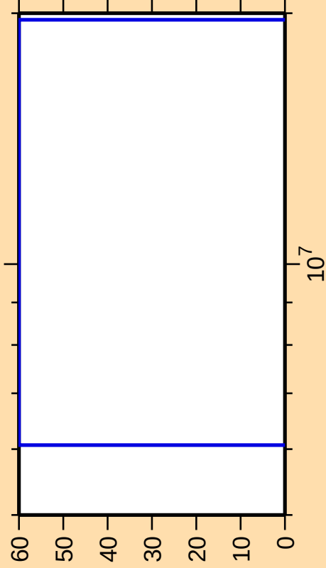
\Delta\sigma/\sigma vs. E for ^{160}\text{Er}(n,np)
