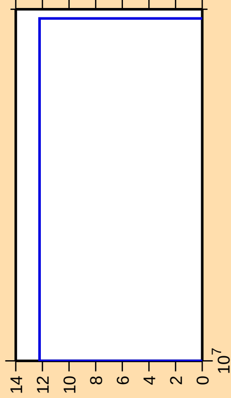
\Delta\sigma/\sigma vs. E for ^{160}\text{Er}(n,\text{nt})
