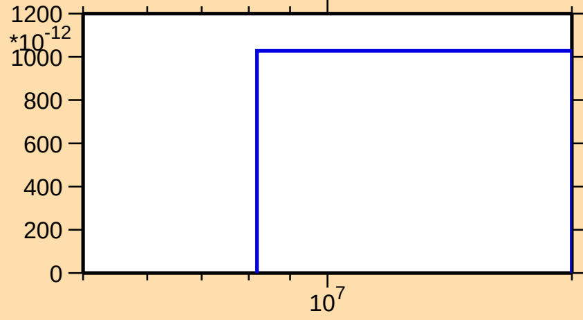
\sigma vs. E for ^{160}\text{Er}(n,p\alpha)
