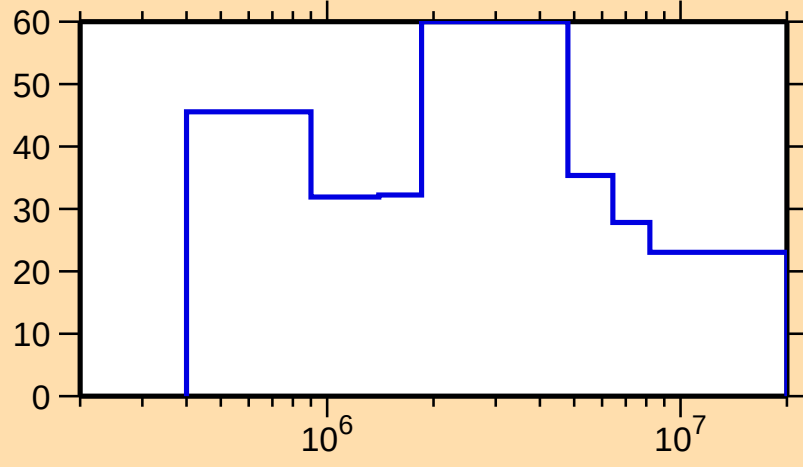
\Delta\sigma/\sigma vs. E for ^{160}\text{Er}(n,n_1)
