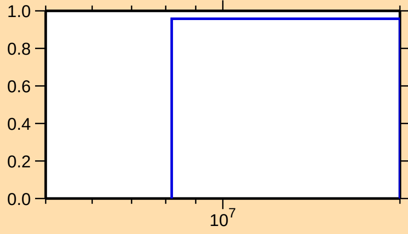
\sigma vs. E for ^{160}\text{Er}(n,2n)
