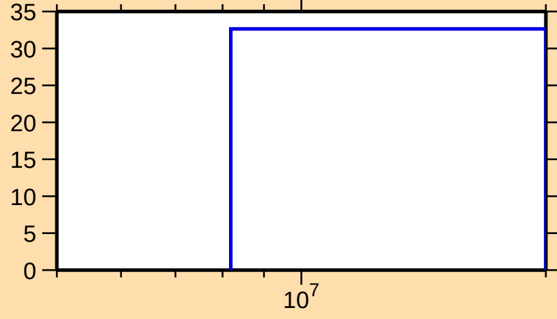
\Delta\sigma/\sigma vs. E for ^{160}\text{Er}(n,\text{inel.})
