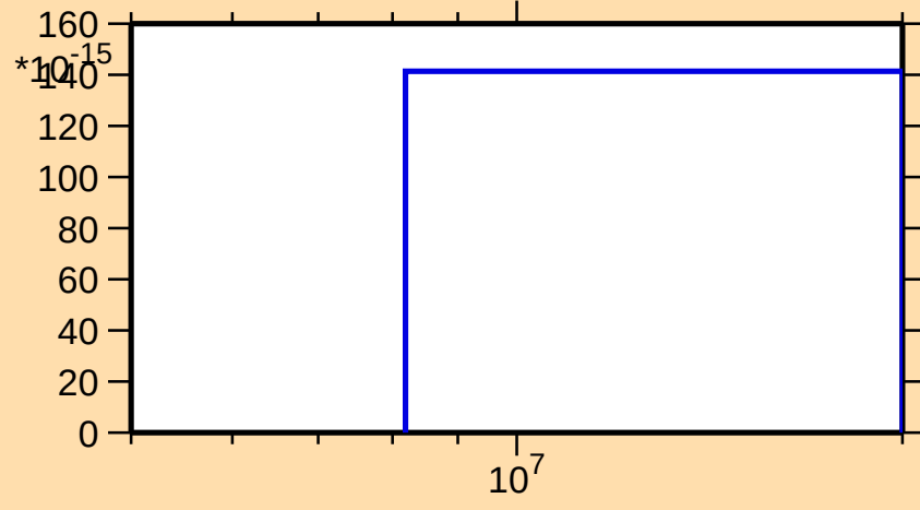
\sigma vs. E for ^{160}\text{Er}(\text{mt } 45)
