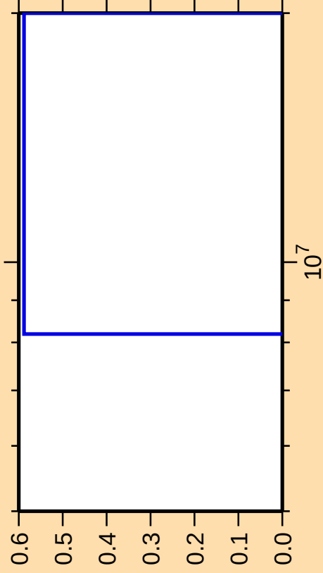
\Delta\sigma/\sigma vs. E for ^{160}\text{Er}(\text{mt } 45)
