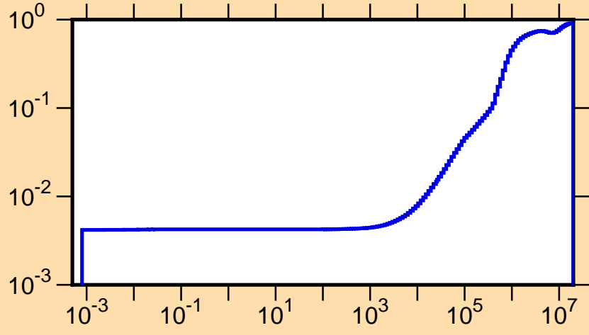
\mu vs. E for ^{161}\text{Er}(\text{mt251})
