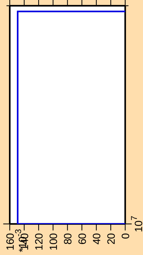
\Delta\sigma/\sigma vs. E for ^{161}\text{Er}(\text{mt } 34)
