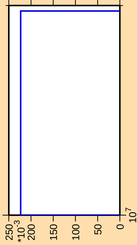
\Delta\sigma/\sigma vs. E for ^{161}\text{Er}(n,\text{pt})
