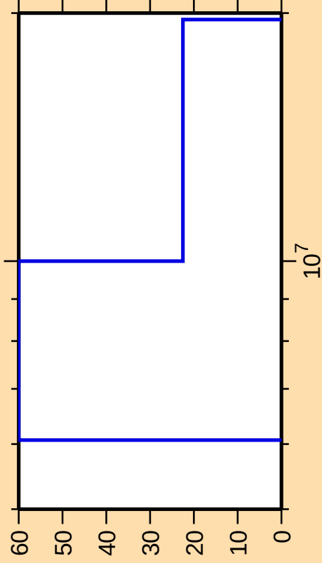
\Delta\sigma/\sigma vs. E for ^{161}\text{Er}(n,np)
