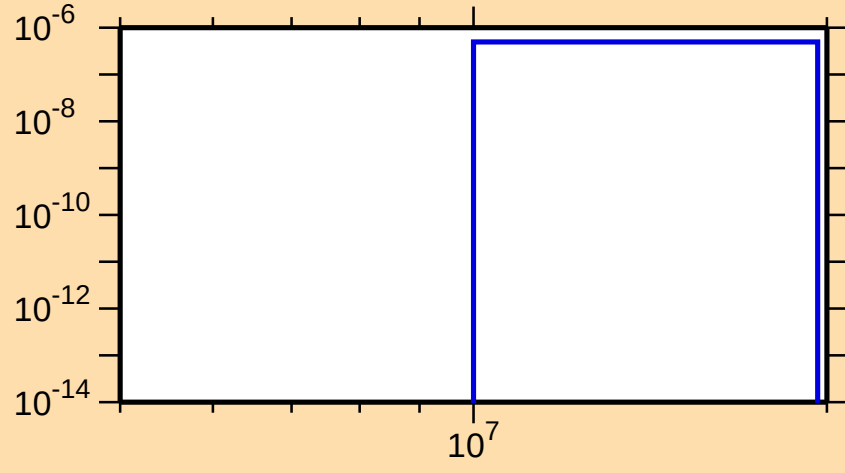
\sigma vs. E for ^{161}\text{Er}(n,2n\alpha)
