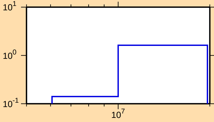
\sigma vs. E for ^{161}\text{Er}(n,2n)
