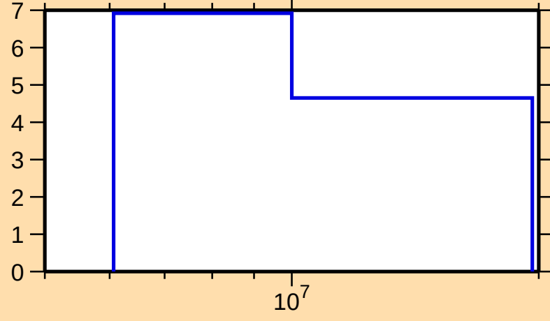
\Delta\sigma/\sigma vs. E for ^{161}\text{Er}(n,\text{nonel.})
