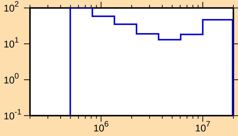
\Delta\sigma/\sigma vs. E for ^{161}\text{Er}(n,\text{ncont.})
