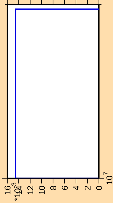
\Delta\sigma/\sigma vs. E for ^{161}\text{Er}(\text{mt117})
