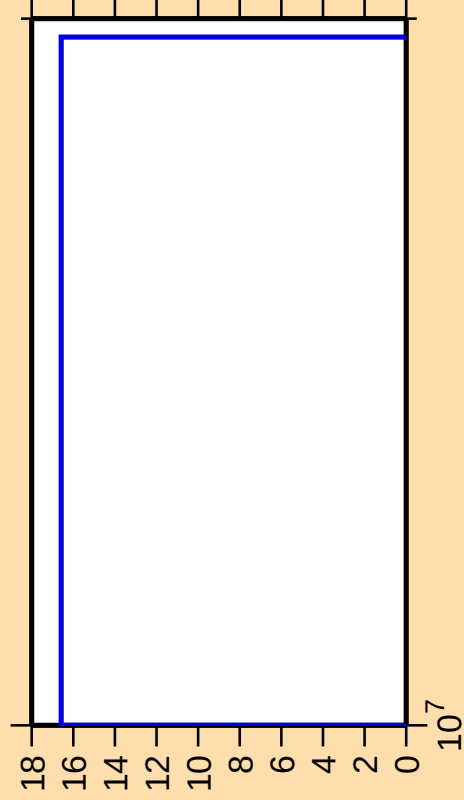
\Delta\sigma/\sigma vs. E for ^{161}\text{Er}(n,\text{nt})
