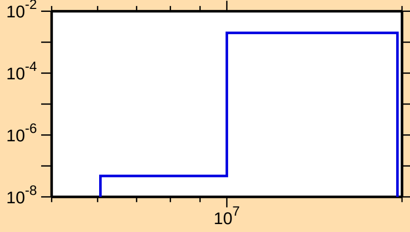
\sigma vs. E for ^{161}\text{Er}(n,np)
