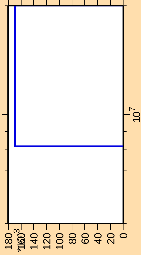
\Delta\sigma/\sigma vs. E for ^{161}\text{Er}(\text{mt 34})
