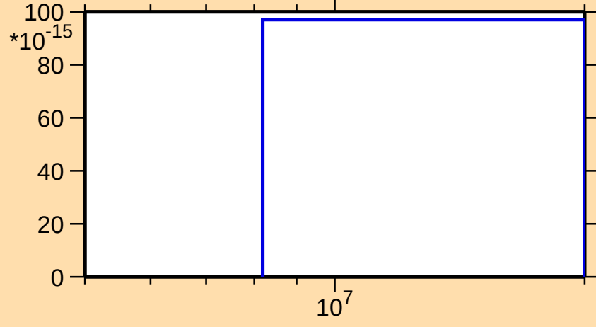
\sigma vs. E for ^{161}\text{Er}(n,\text{pd})
