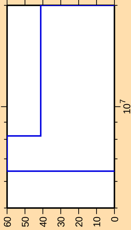
\Delta\sigma/\sigma vs. E for ^{161}\text{Er}(n,p)
