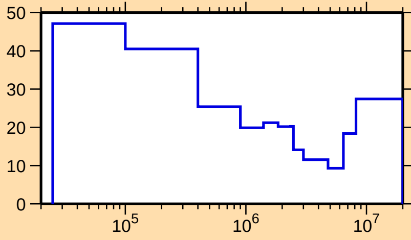
\Delta\sigma/\sigma vs. E for ^{161}\text{Er}(n,\text{inel.})
