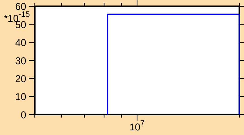
\sigma vs. E for ^{161}\text{Er}(\text{mt 34})
