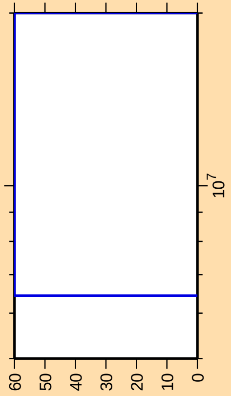
\Delta\sigma/\sigma vs. E for ^{161}\text{Er}(n,\gamma)
