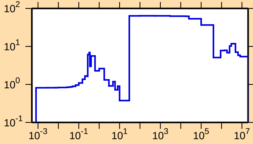
\Delta\sigma/\sigma vs. E for ^{161}\text{Er}(n,\text{el.})
