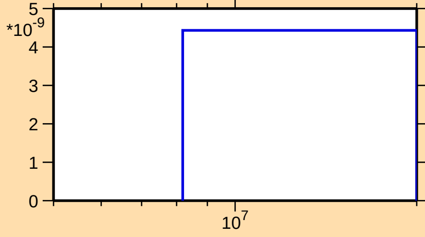
\sigma vs. E for ^{161}\text{Er}(n,\text{He3})
