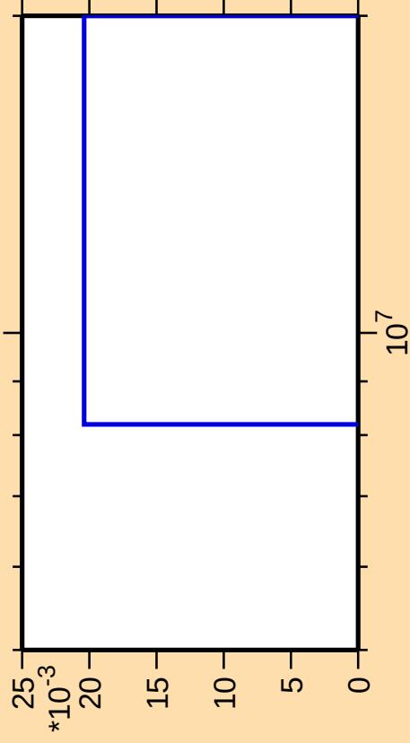
\Delta\sigma/\sigma vs. E for ^{161}\text{Er} (mt 45)
