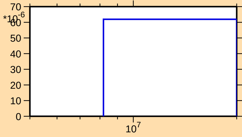
\sigma vs. E for ^{161}\text{Er}(n,t)
