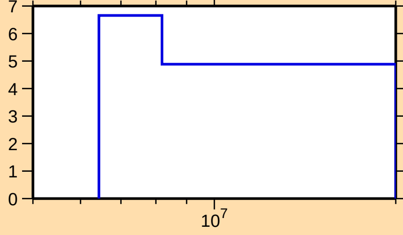
\Delta\sigma/\sigma vs. E for ^{161}\text{Er}(n,\text{nonel.})
