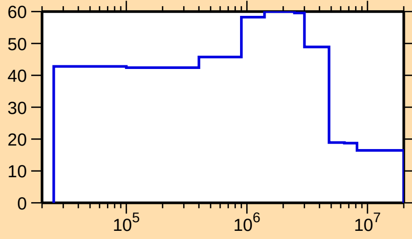
\Delta\sigma/\sigma vs. E for ^{161}\text{Er}(n,n_1)
