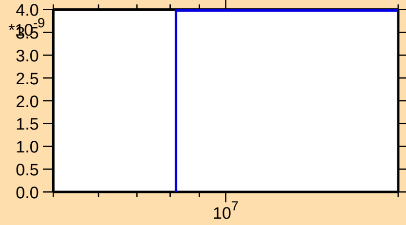
\sigma vs. E for ^{161}\text{Er}(n,p\alpha)
