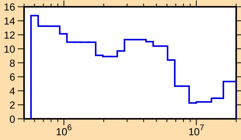
\Delta\sigma/\sigma vs. E for ^{163}\text{Er}(n,\text{tot.})
