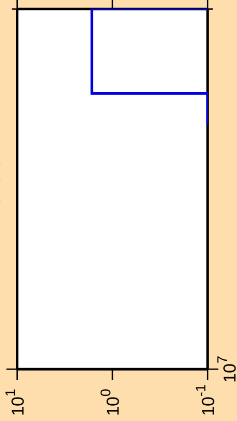
\Delta\sigma/\sigma vs. E for ^{163}\text{Er}(n,\text{pt})
