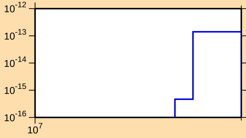
\sigma vs. E for ^{163}\text{Er}(n,\text{pd})
