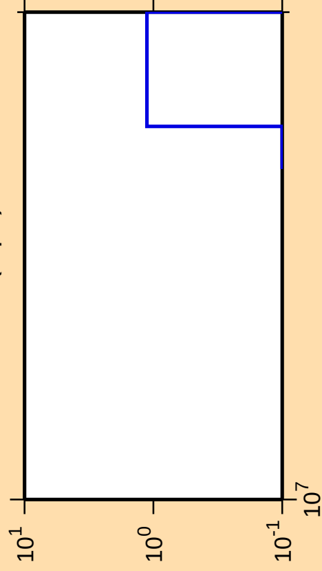
\Delta\sigma/\sigma vs. E for ^{163}\text{Er}(n,\text{pd})
