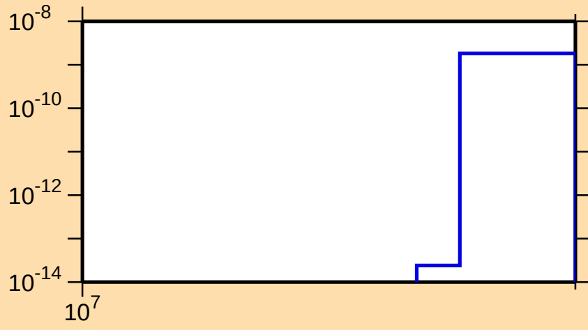
\sigma vs. E for ^{163}\text{Er}(n,nt)
