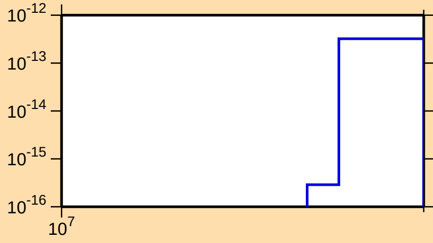
\sigma vs. E for ^{163}\text{Er}(n,\text{pt})
