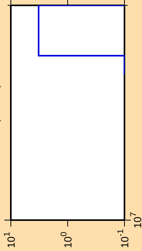
\Delta\sigma/\sigma vs. E for ^{163}\text{Er}(\text{mt } 34)
