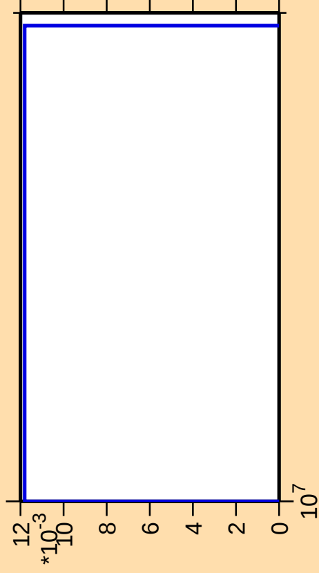
\Delta\sigma/\sigma vs. E for ^{163}\text{Er}(n,\text{pt})
