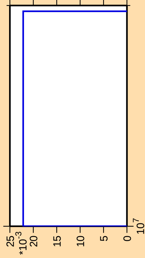
\Delta\sigma/\sigma vs. E for ^{163}\text{Er} (mt 34)
