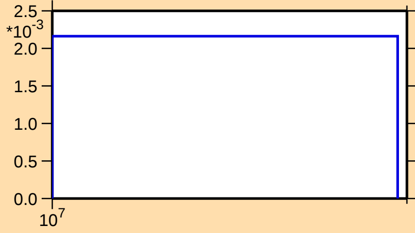
\sigma vs. E for ^{163}\text{Er}(n,3n)
