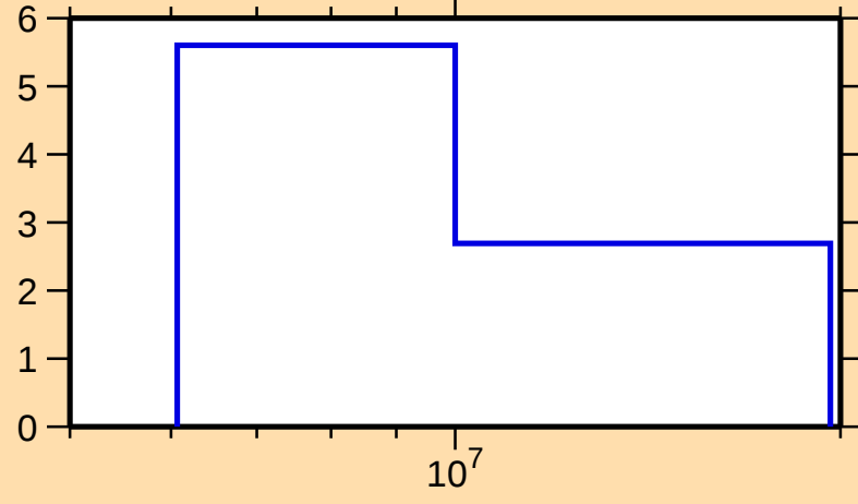
\Delta\sigma/\sigma vs. E for ^{163}\text{Er}(n,\text{tot.})
