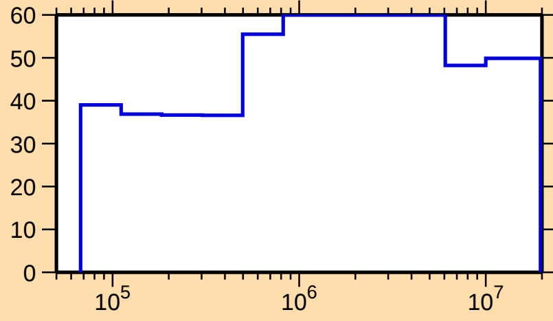
\Delta\sigma/\sigma vs. E for ^{163}\text{Er}(n,n_1)
