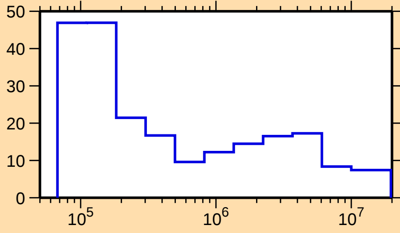
\Delta\sigma/\sigma vs. E for ^{163}\text{Er}(n,\text{el.})
