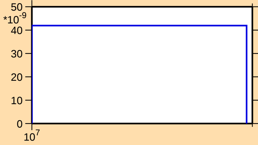
\sigma vs. E for ^{163}\text{Er}(n,\text{nd})
