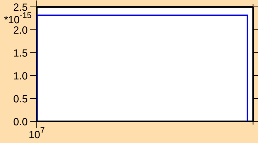
\sigma vs. E for ^{163}\text{Er}(n,\text{pt})
