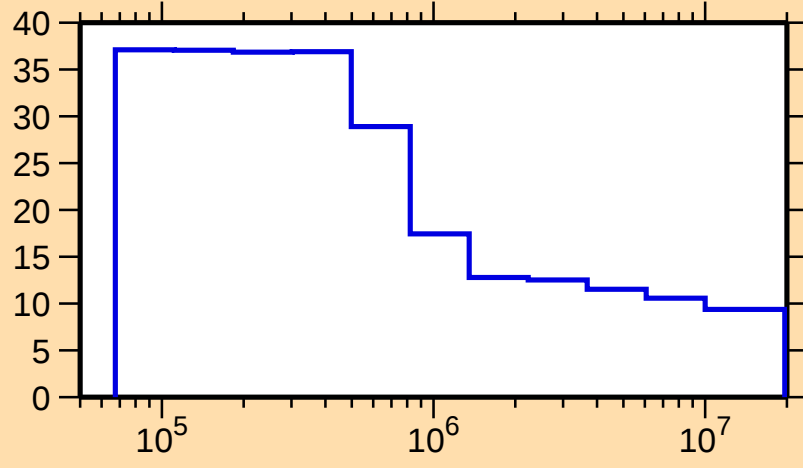
\Delta\sigma/\sigma vs. E for ^{163}\text{Er}(n,\text{nonel.})
