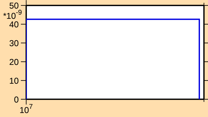
\sigma vs. E for ^{163}\text{Er}(n,2np)
