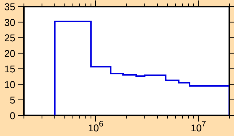
\Delta\sigma/\sigma vs. E for ^{163}\text{Er}(\text{n},\text{nonel.})
