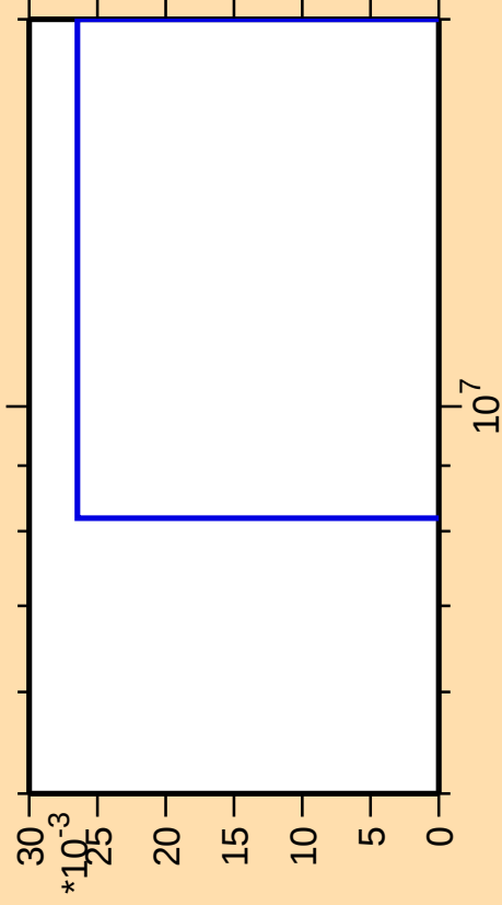
\Delta\sigma/\sigma vs. E for ^{163}\text{Er}(\text{mt } 34)
