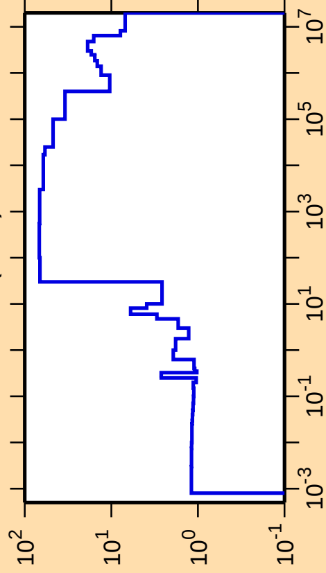
\Delta\sigma/\sigma vs. E for ^{163}\text{Er}(n,\text{el.})
