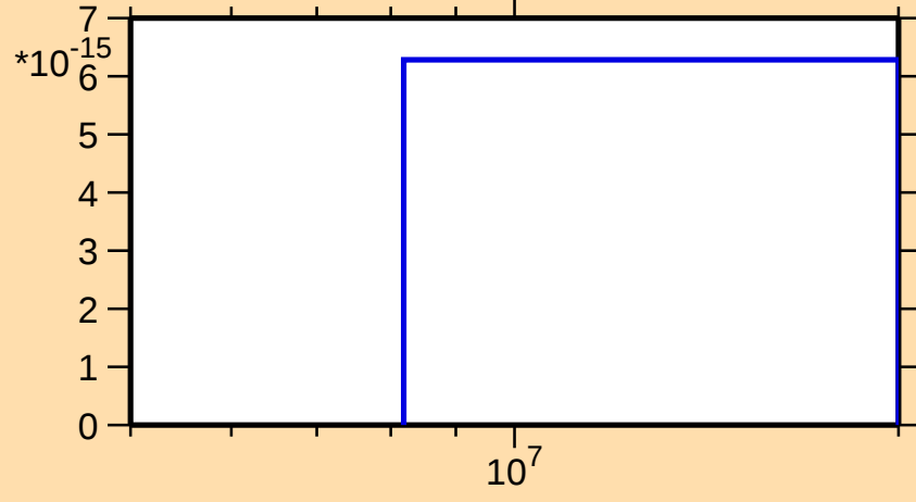
\sigma vs. E for ^{163}\text{Er}(\text{mt } 34)
