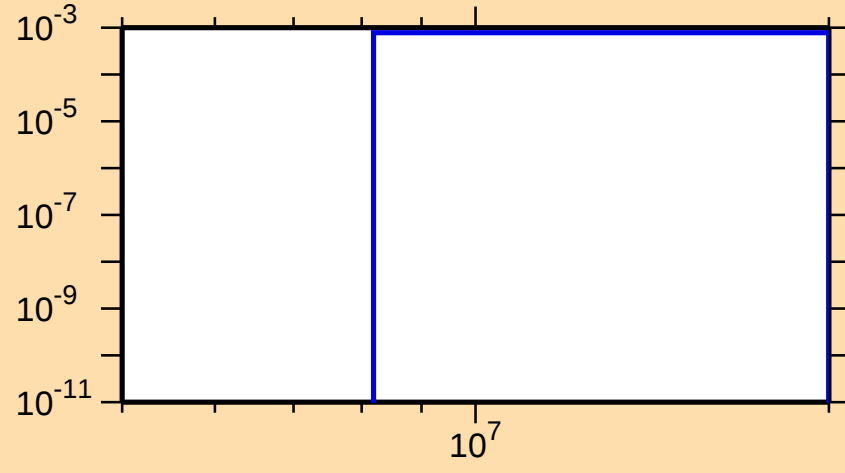
\sigma vs. E for ^{163}\text{Er}(n,np)
