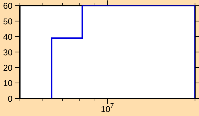
\Delta\sigma/\sigma vs. E for ^{163}\text{Er}(n,\text{inel.})
