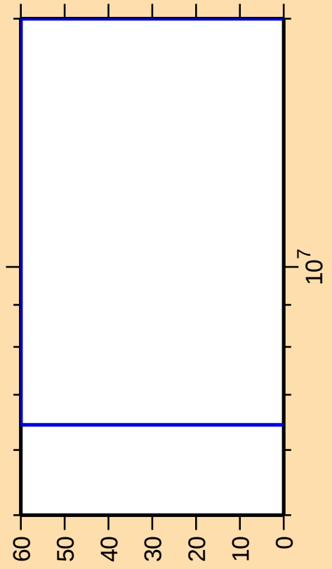
\Delta\sigma/\sigma vs. E for ^{163}\text{Er}(n,\gamma)
