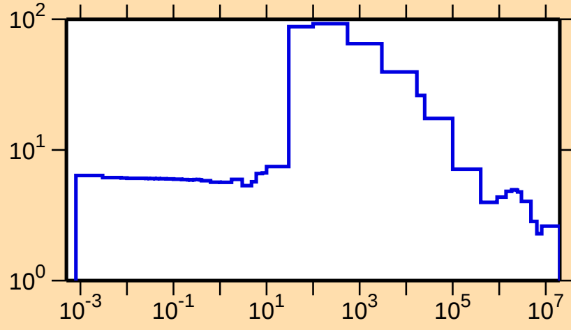
\sigma vs. E for ^{163}\text{Er}(n,\text{el.})
