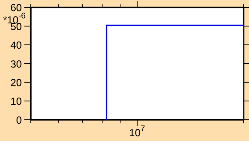
\sigma vs. E for ^{163}\text{Er}(n,t)
