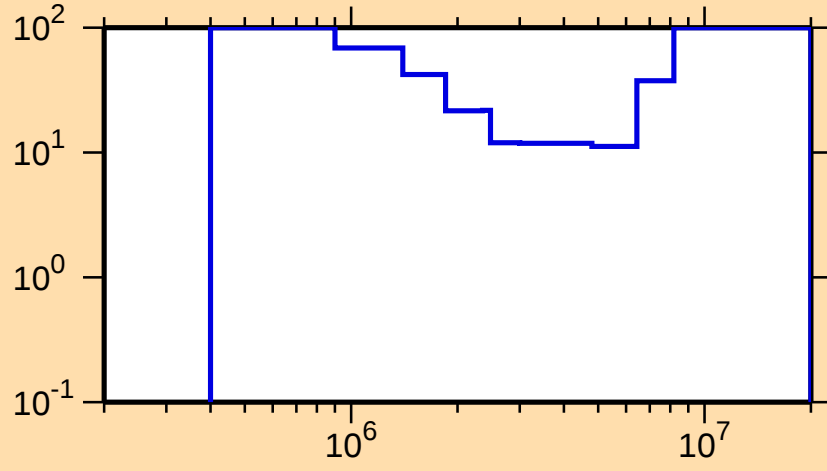
\Delta\sigma/\sigma vs. E for ^{163}\text{Er}(n,n\text{cont.})
