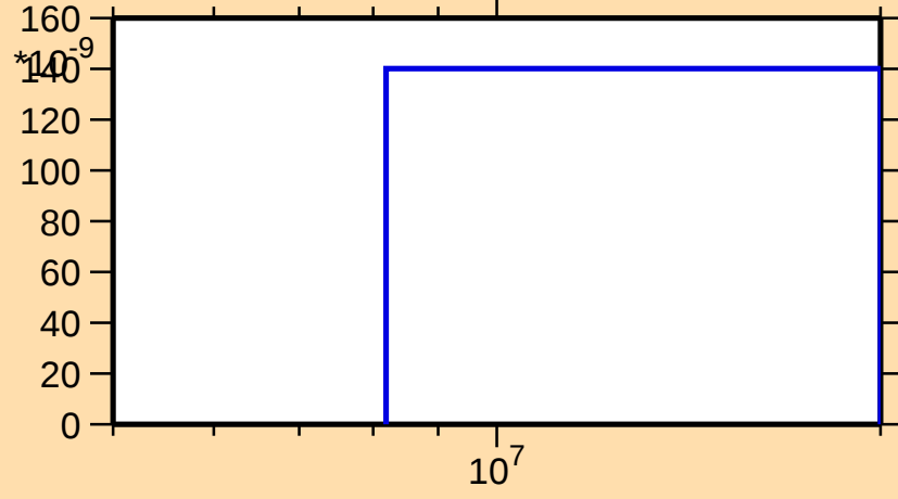
\sigma vs. E for ^{163}\text{Er}(n,2n\alpha)
