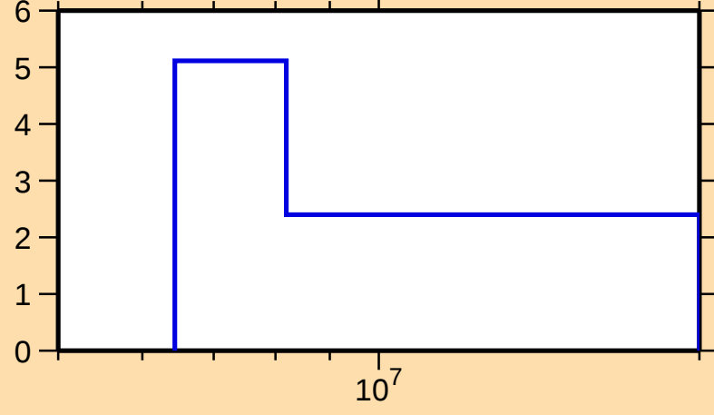
\Delta\sigma/\sigma vs. E for ^{163}\text{Er}(n,\text{tot.})
