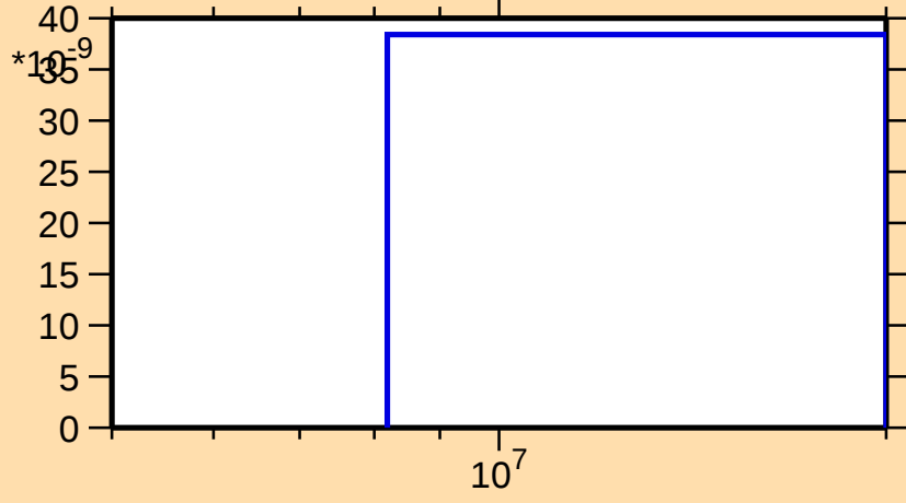
\sigma vs. E for ^{163}\text{Er}(n,2np)
