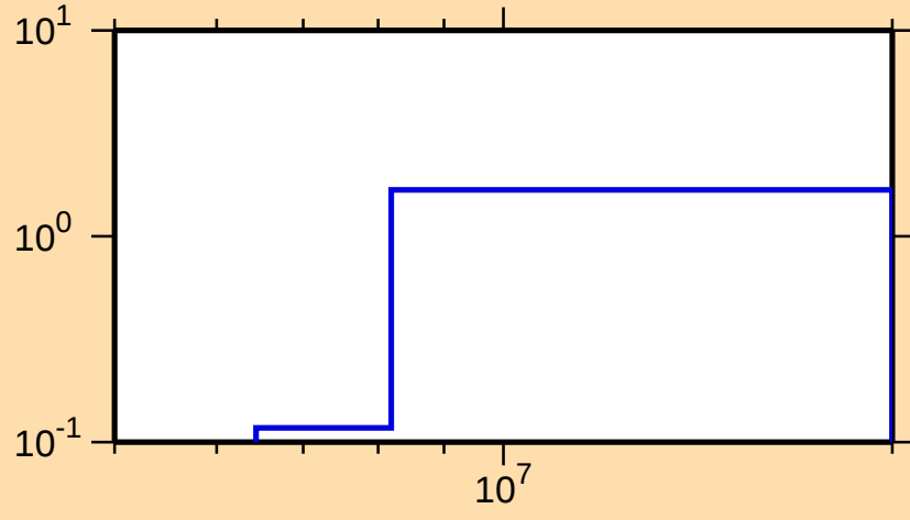
\sigma vs. E for ^{163}\text{Er}(n,2n)
