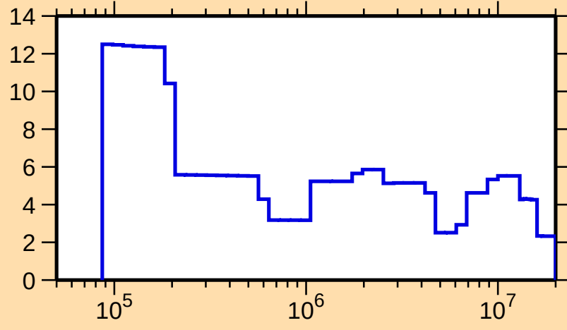
\Delta\sigma/\sigma vs. E for ^{164}\text{Er}(n,\text{el.})
