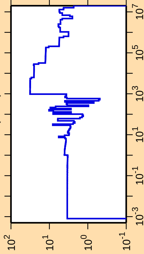
\Delta\sigma/\sigma vs. E for ^{164}\text{Er}(n,\text{el.})
