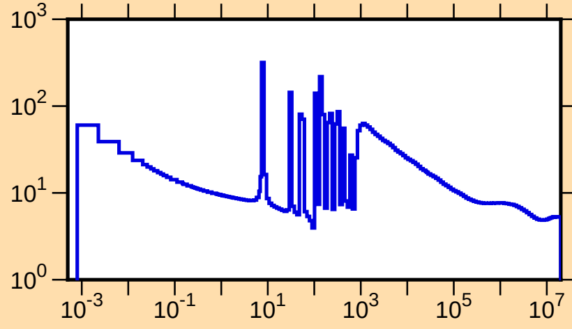
\sigma vs. E for ^{164}\text{Er}(n,\text{tot.})
