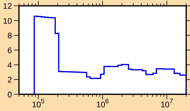
\Delta\sigma/\sigma vs. E for ^{164}\text{Er}(n,\text{tot.})
