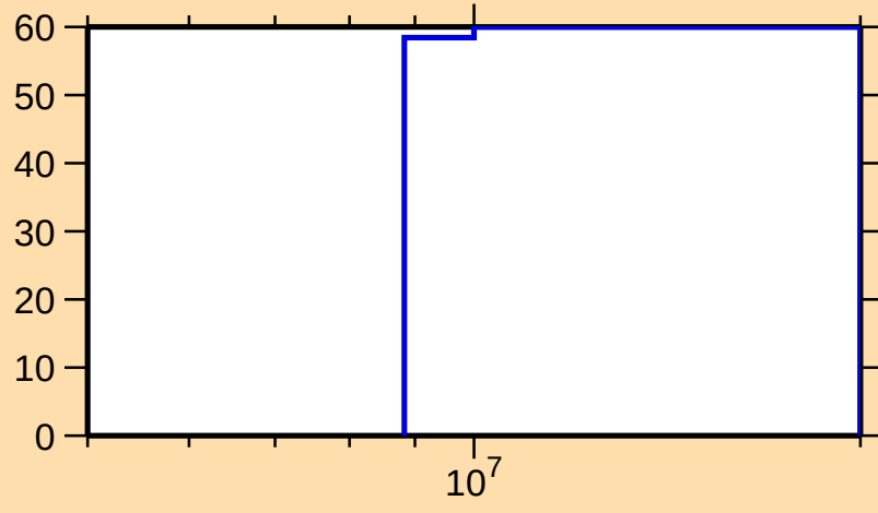
\Delta\sigma/\sigma vs. E for ^{164}\text{Er}(n,\text{inel.})
