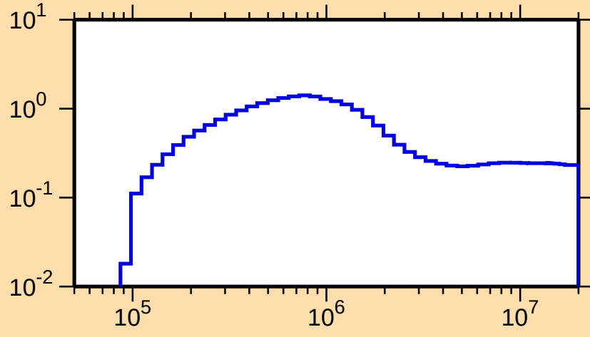
\sigma vs. E for ^{164}\text{Er}(n,n_1)
