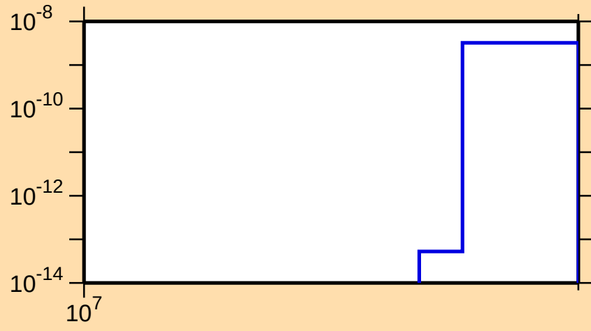
\sigma vs. E for ^{164}\text{Er}(n,nt)
