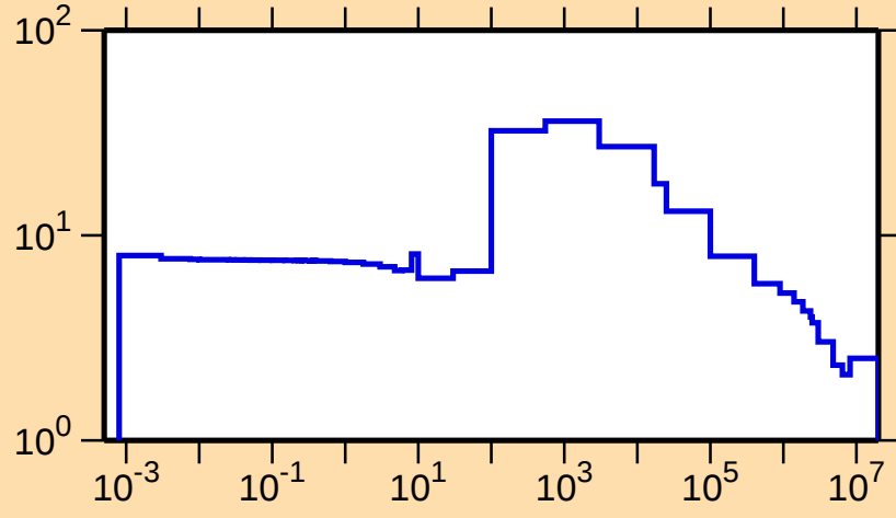
\sigma vs. E for ^{164}\text{Er}(n,\text{el.})
