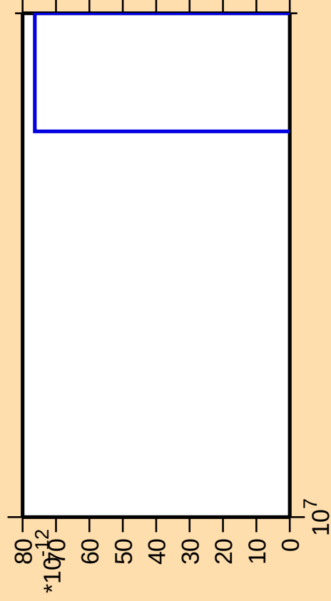
\Delta\sigma/\sigma vs. E for ^{165}\text{Er}(\text{mt 11})
