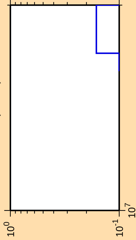
\Delta\sigma/\sigma vs. E for ^{165}\text{Er}(\text{mt } 34)
