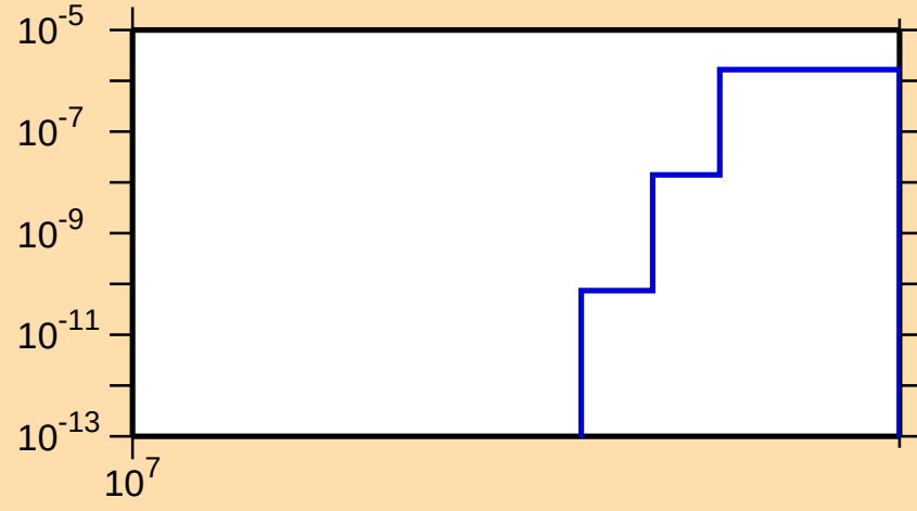
\sigma vs. E for ^{165}\text{Er}(n,2np)
