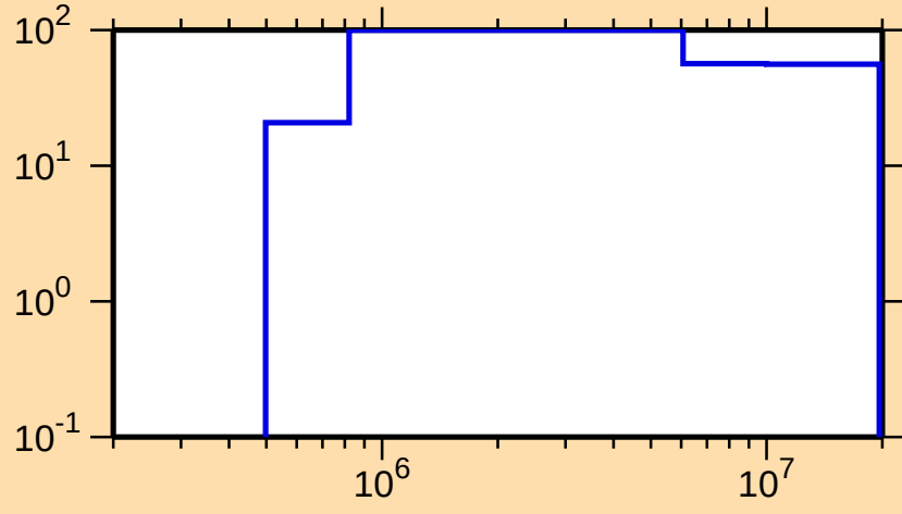
\Delta\sigma/\sigma vs. E for ^{165}\text{Er}(n,p)
