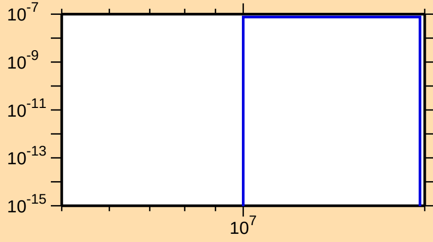
\sigma vs. E for ^{165}\text{Er}(n,2n\alpha)
