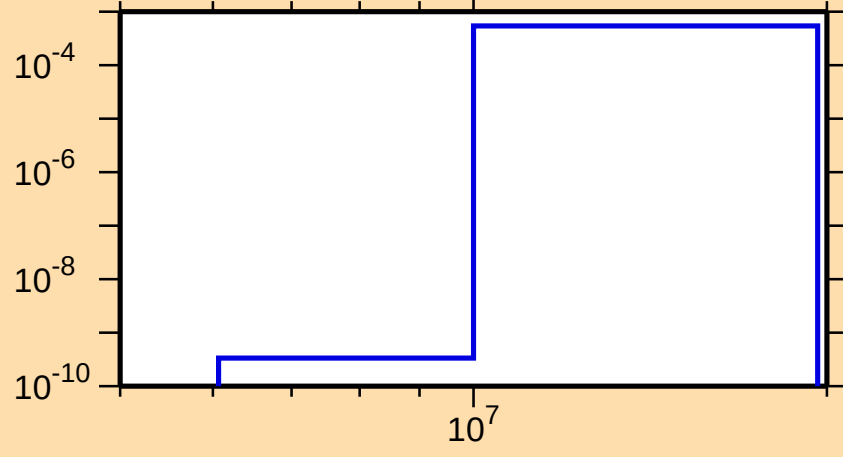
\sigma vs. E for ^{165}\text{Er}(n,np)
