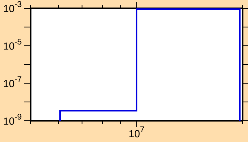
\sigma vs. E for ^{165}\text{Er}(n,d)
