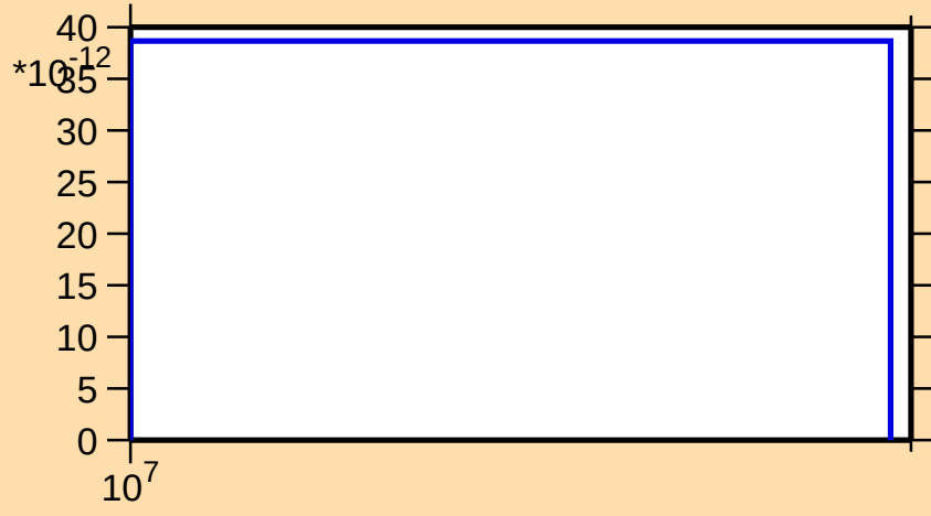
\sigma vs. E for ^{165}\text{Er}(n,\text{nt})
