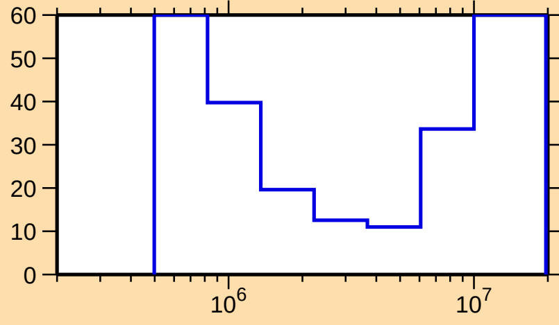
\Delta\sigma/\sigma vs. E for ^{165}\text{Er}(n,n\text{cont.})
