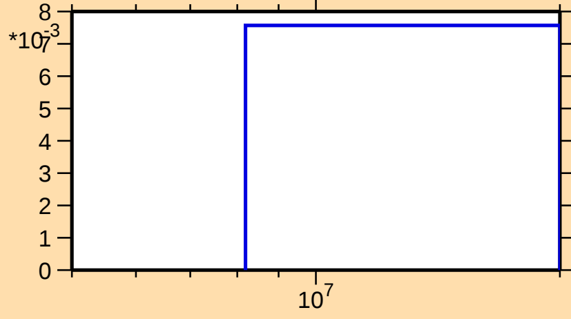
\sigma vs. E for ^{165}\text{Er}(n,3n)
