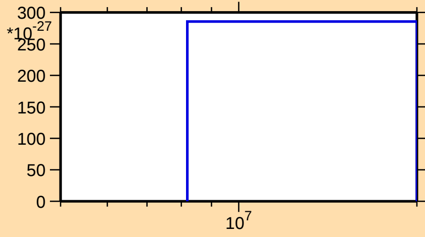
\sigma vs. E for ^{165}\text{Er}(\text{mt } 11)
