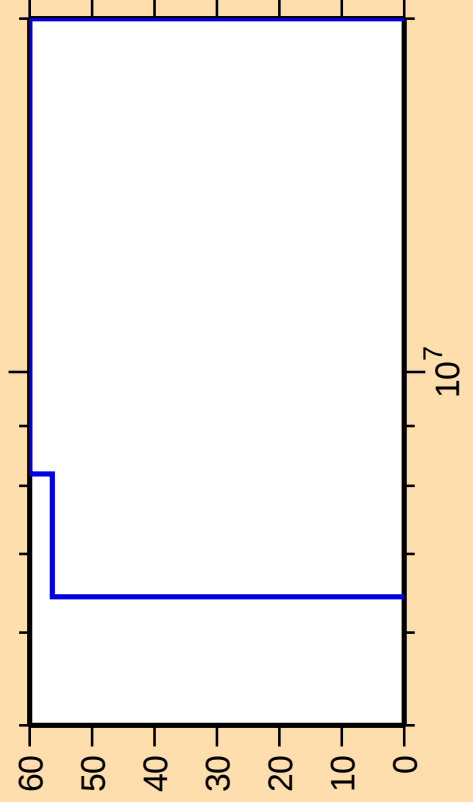
\Delta\sigma/\sigma vs. E for ^{165}\text{Er}(n,\gamma)
