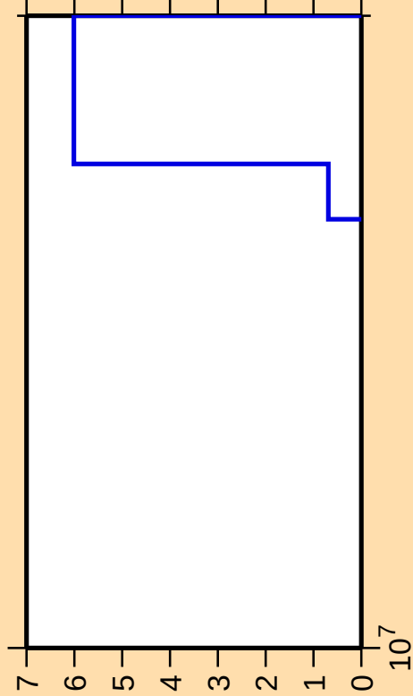
\Delta\sigma/\sigma vs. E for ^{166}\text{Er}(n,p\alpha)
