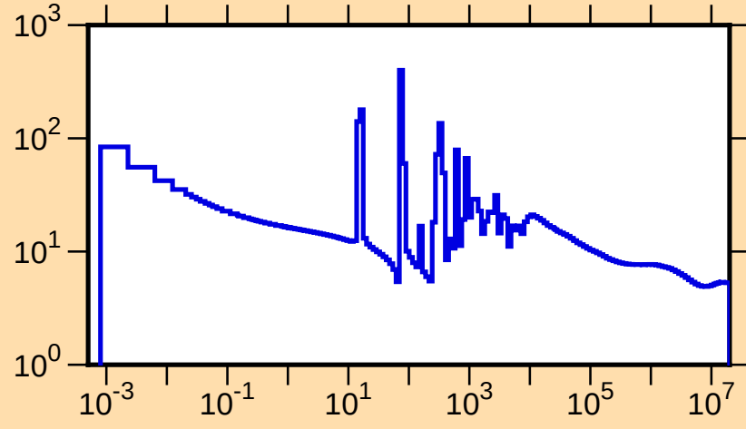
\sigma vs. E for ^{166}\text{Er}(n,\text{tot.})
