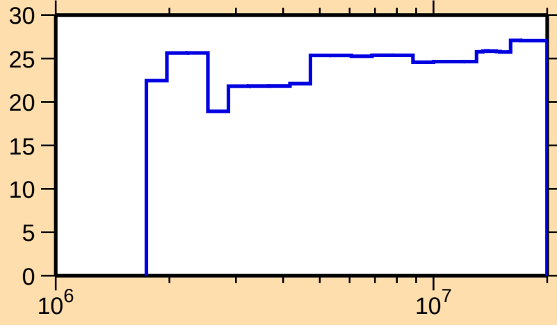
\Delta\sigma/\sigma vs. E for ^{166}\text{Er}(n,n_1)
