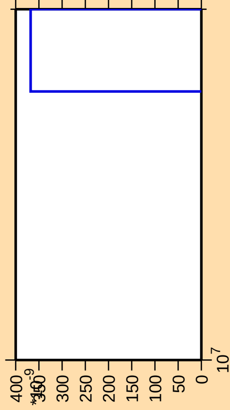
\Delta\sigma/\sigma vs. E for ^{166}\text{Er}(\text{mt } 11)
