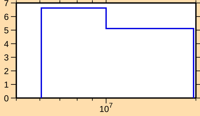
\Delta\sigma/\sigma vs. E for ^{166}\text{Er}(n,\text{nonel.})
