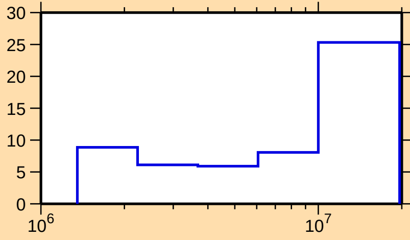
\Delta\sigma/\sigma vs. E for ^{166}\text{Er}(n,\text{inel.})
