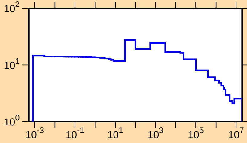
\sigma vs. E for ^{166}\text{Er}(n,\text{el.})
