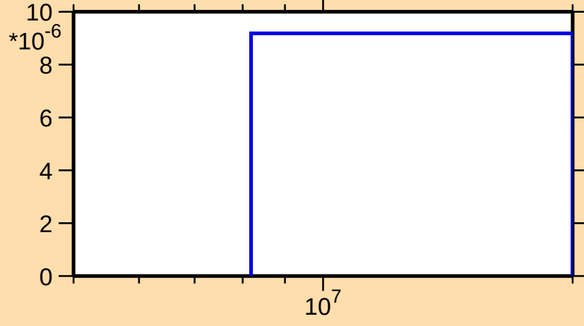
\sigma vs. E for ^{166}\text{Er}(n,t)
