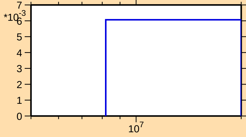
\sigma vs. E for ^{166}\text{Er}(n,3n)
