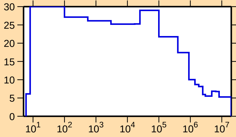
\Delta\sigma/\sigma vs. E for ^{166}\text{Er}(n,\text{nonel.})
