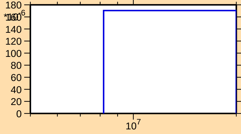
\sigma vs. E for ^{166}\text{Er}(n,np)
