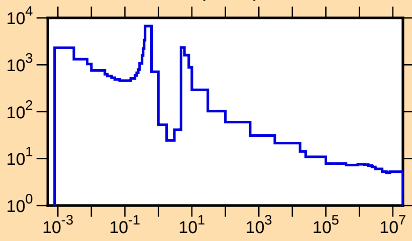
\sigma vs. E for ^{167}\text{Er}(n,\text{tot.})
