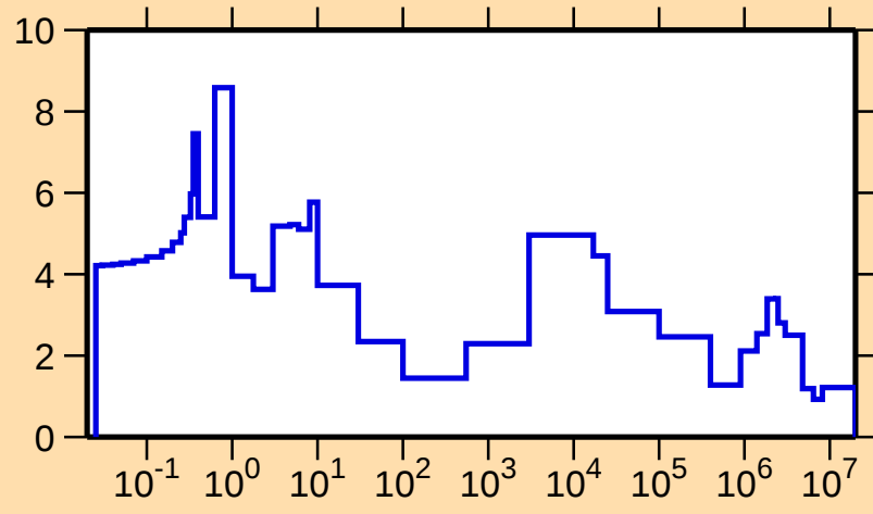
\Delta\sigma/\sigma vs. E for ^{167}\text{Er}(n,\text{tot.})
