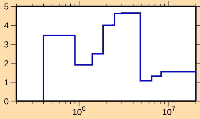
\Delta\sigma/\sigma vs. E for ^{167}\text{Er}(\text{n},\text{el.})
