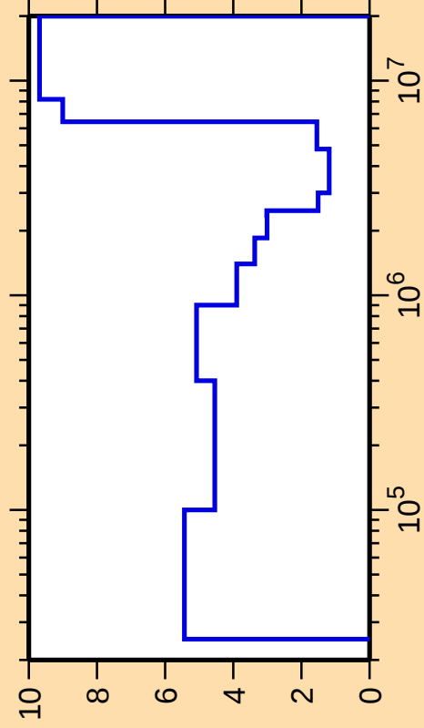
\Delta\sigma/\sigma vs. E for ^{167}\text{Er}(n,\text{inel.})
